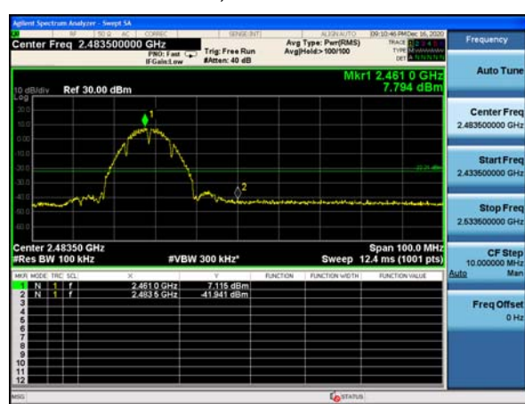
802.11g, Channel No.: 11
