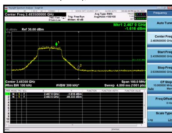
802.11n(HT20), Channel No.: 11
