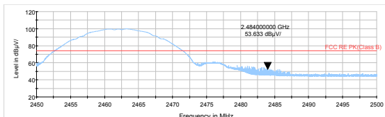
802.11b-Channel 11 Peak
