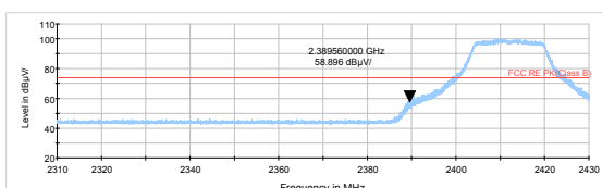
802.11g-Channel 1 Peak
