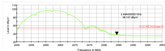
802.11b-Channel 11 Average
