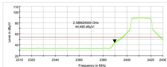
802.11g-Channel 1 Average
