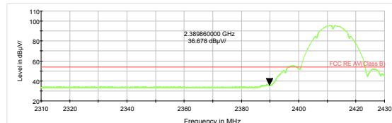
802.11b-Channel 1 Average
