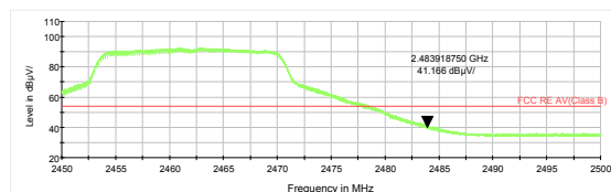
802.11g-Channel 11 Average
