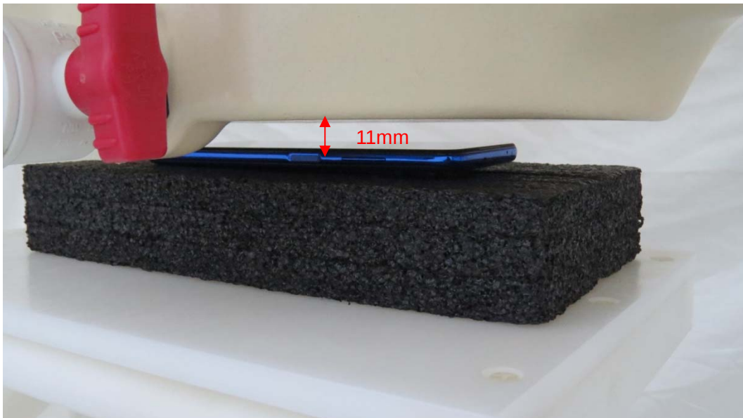
Picture 8: Front Side, the distance from handset to the bottom of the Phantom is 11mm
