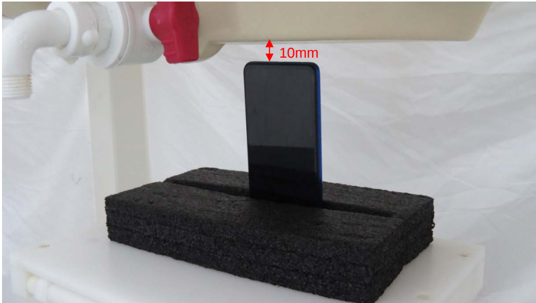
Picture 13: Bottom Edge, the distance from handset to the bottom of the Phantom is 16mm
