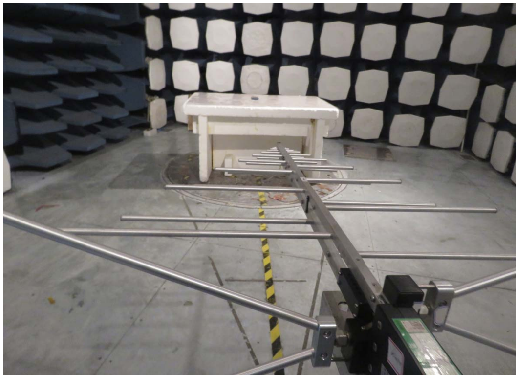
30MHz-1GHz
