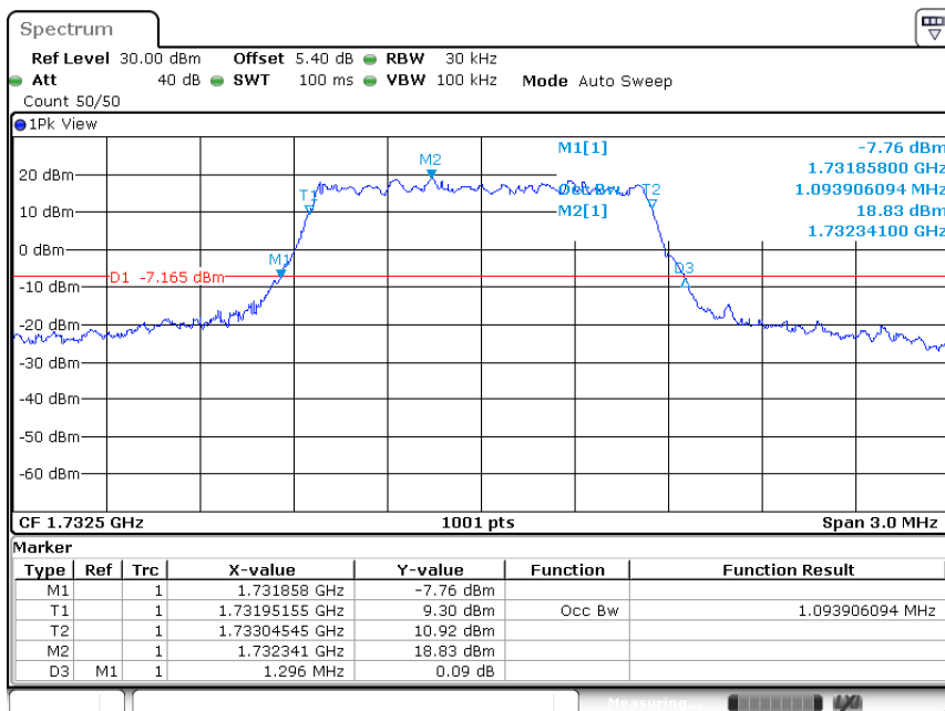
Band4-1.4MHz-QPSK-20175-6RB#0-1.094
