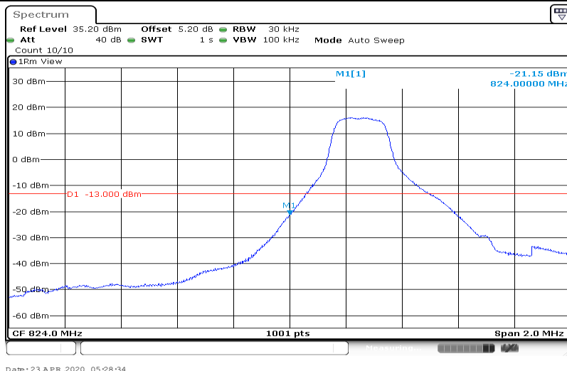
Band5-1.4MHz-QPSK-20407-6RB#0
