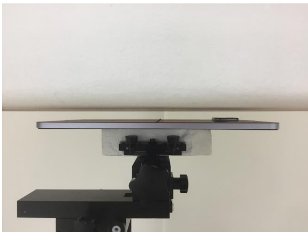
Bottom Face, Test Separation 15 mm(Sensor off)
