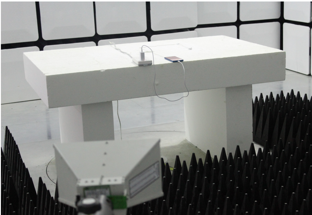
1.3 Setup for Unwanted Emissions that fall Outside of the Restricted Bands(Radiated) and Unwanted Emissions in the Restricted Bands (Radiated) above 1GHz ( Test Location: SGS-CSTC STANDARDS TECHNICAL SERVICES (XI 'AN) CO., LTD.)
