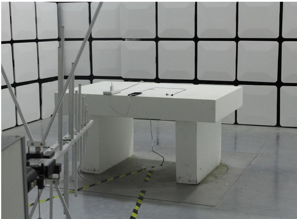
1.2 Setup for Unwanted Emissions that fall Outside of the Restricted Bands(Radiated) and Unwanted Emissions in the Restricted Bands (Radiated) below 1GHz ( Test Location: SGS-CSTC STANDARDS TECHNICAL SERVICES (XI 'AN) CO., LTD.)
