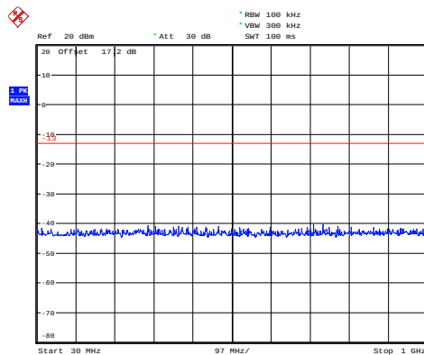
WCDMA Band IV CH-Middle 30MHz~1GHz
