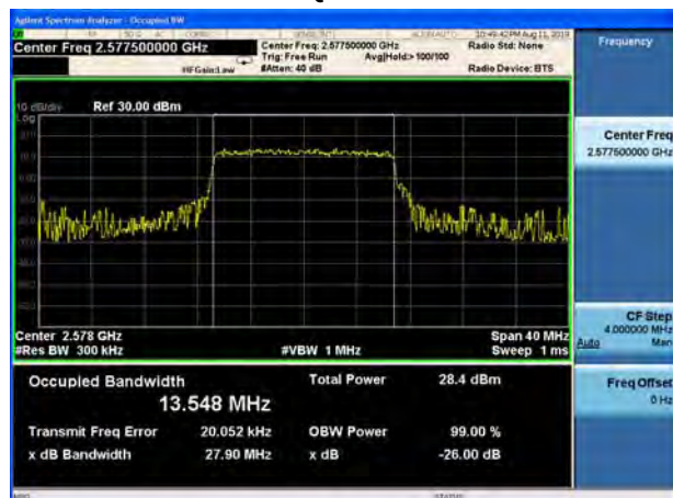
LTE Band 38 64QAM 15MHz CH-Middle
