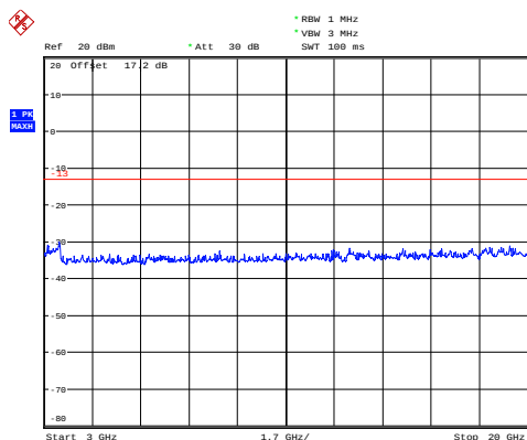
WCDMA Band IV CH-Low 3GHz~20GHz
