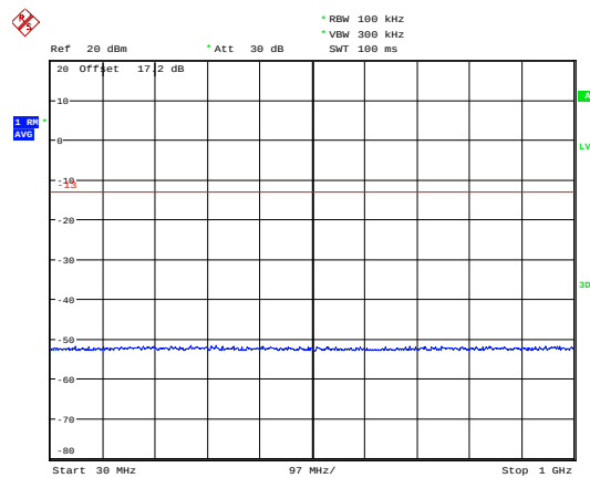
LTE Band 2 3MHz CH-High 30MHz~1GHz
