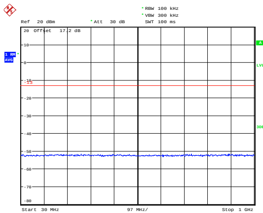
LTE Band 2 3MHz CH-Middle 30MHz~1GHz
