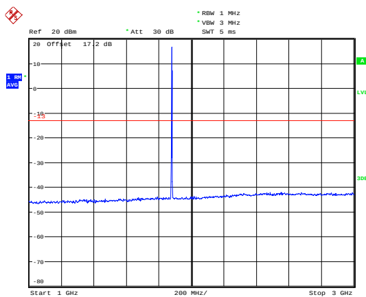
LTE Band 2 3MHz CH-Middle 1GHz~3GHz
