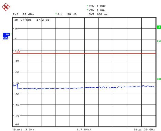
LTE Band 2 3MHz CH-Middle 3GHz~20GHz
