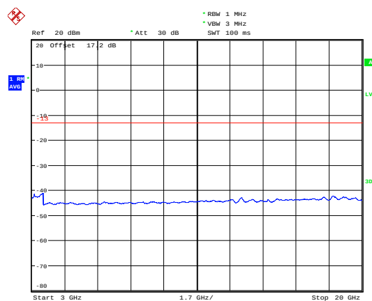
LTE Band 2 3MHz CH-High 3GHz~20GHz
