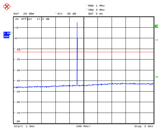
LTE Band 2 3MHz CH-High 1GHz~3GHz
