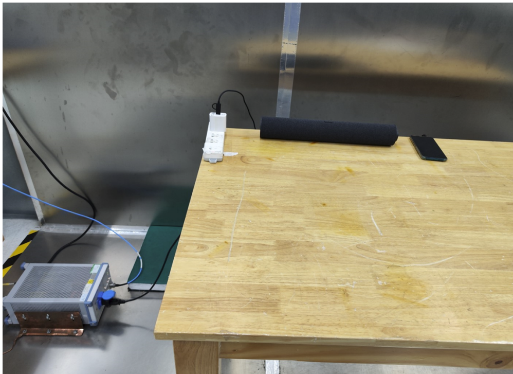
Photograph 4: Set-up for Conducted Emission on AC Mains
