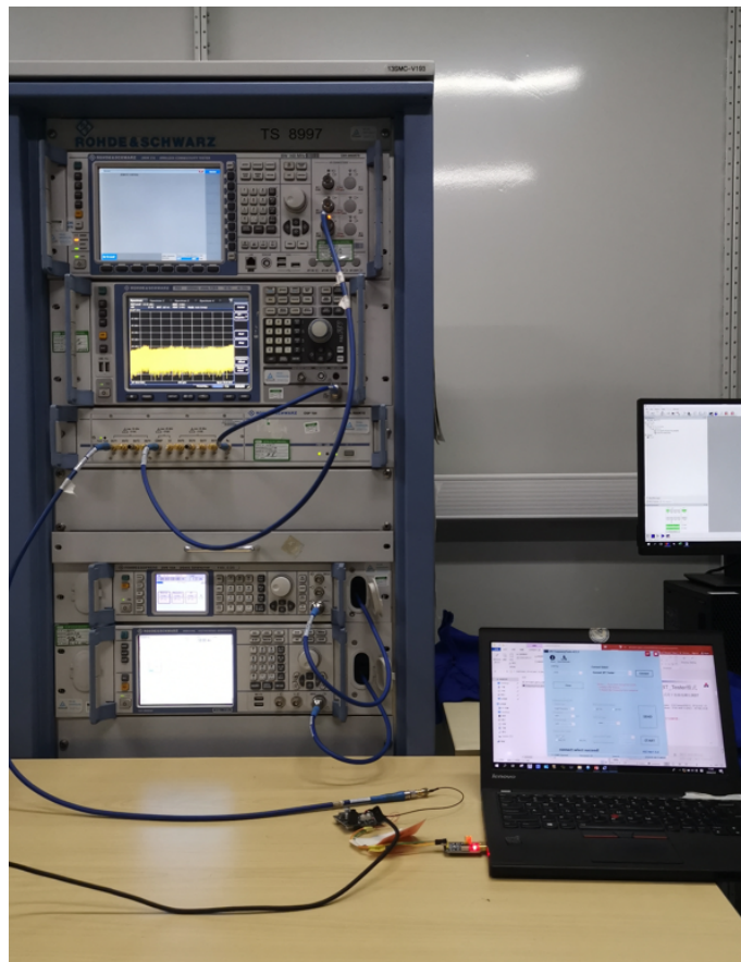
Photograph 1: Set-up photo for Radio Spectrum Testing
