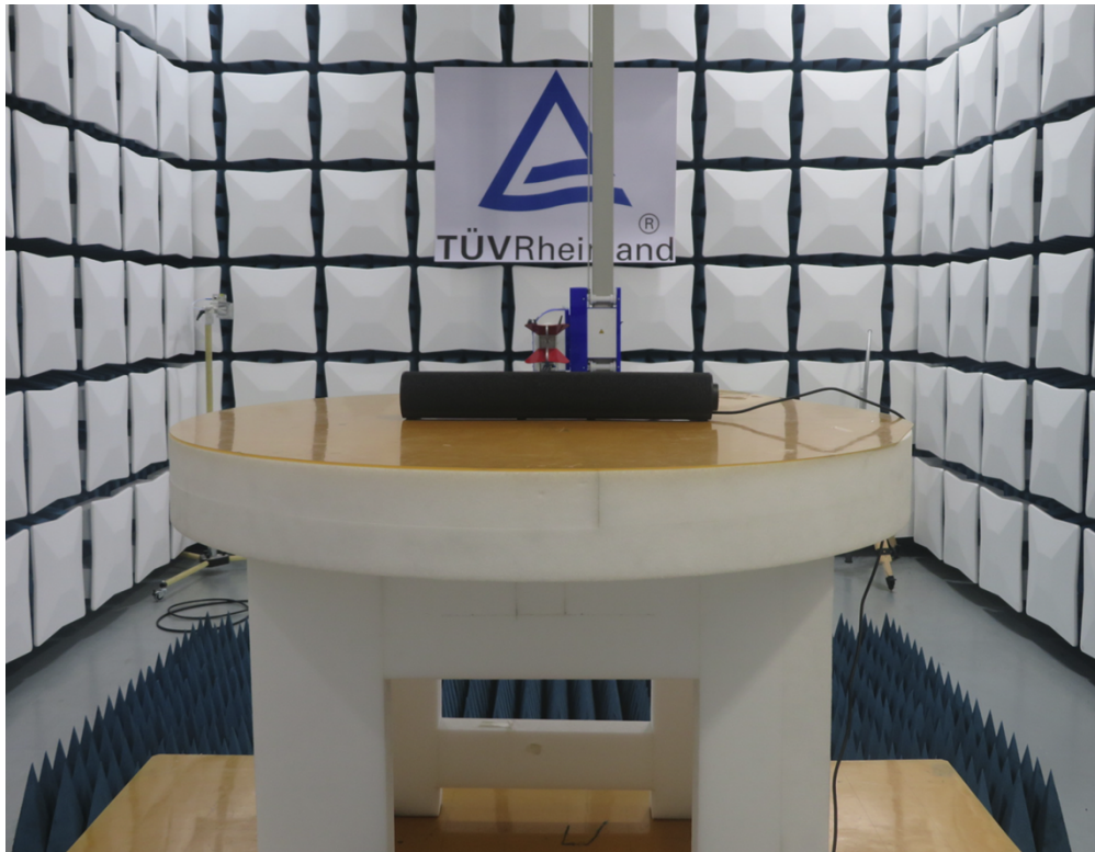
Photograph 3: Set-up photo for Radiated Spurious Emission, above 1GHz
