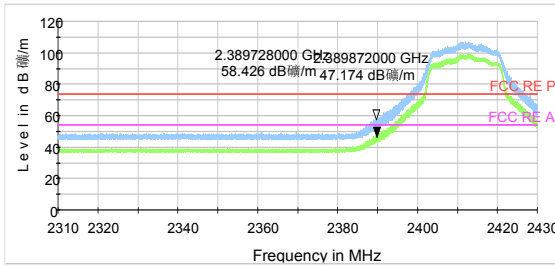
802.11n HT20 -Channel 1 Peak+ Average
