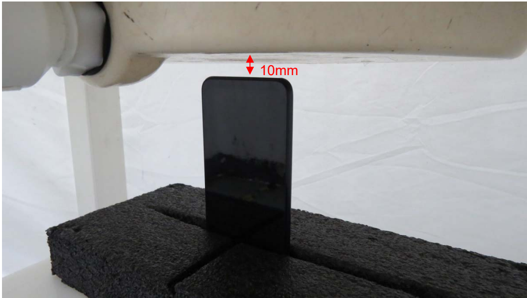
Picture 13: Bottom Edge, the distance from handset to the bottom of the Phantom is 10mm
