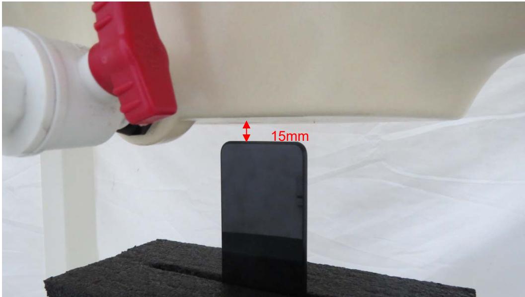
Picture 7: Bottom Edge, the distance from handset to the bottom of the Phantom is 15mm
