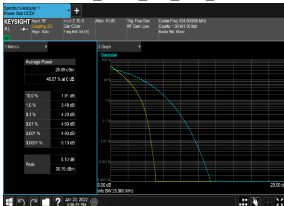
N5(20M)_DFT-s-OFDM_PI_2- BPSK_Outer_Full_Low_CH
