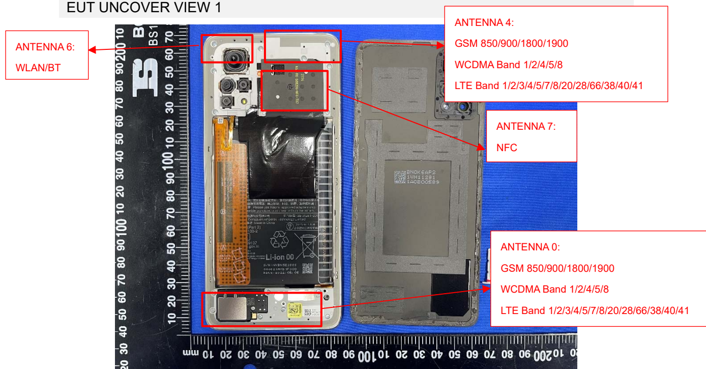
EUT UNCOVER VIEW 1
