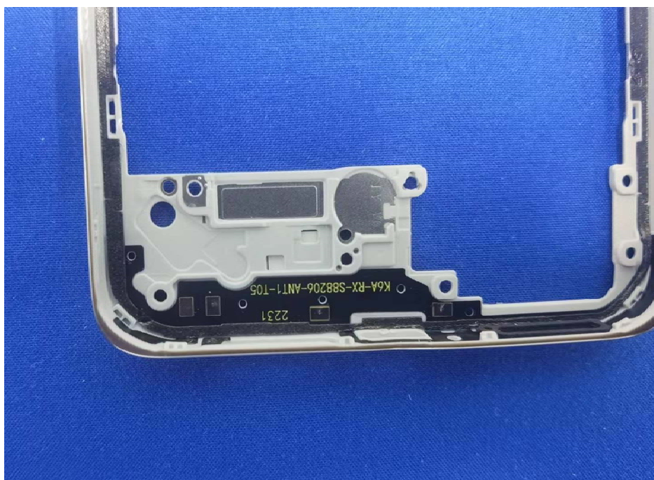
MAIN ANT 0 CLOSE VIEW
