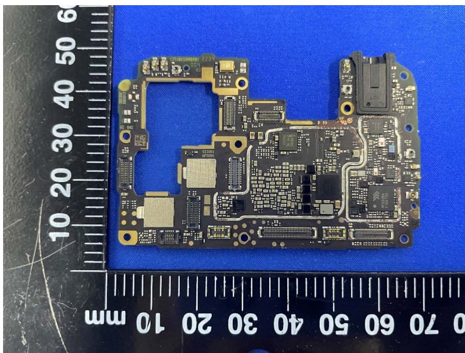
MAIN BOARD TOP VIEW (WITHOUT SHIELD COVER)
