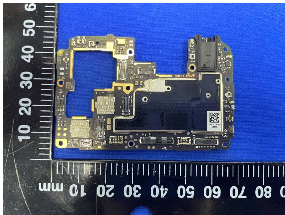
MAIN BOARD TOP VIEW (WITH SHIELD COVER)
