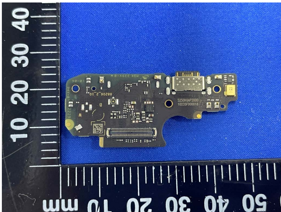
SECONDARY BOARD TOP VIEW
