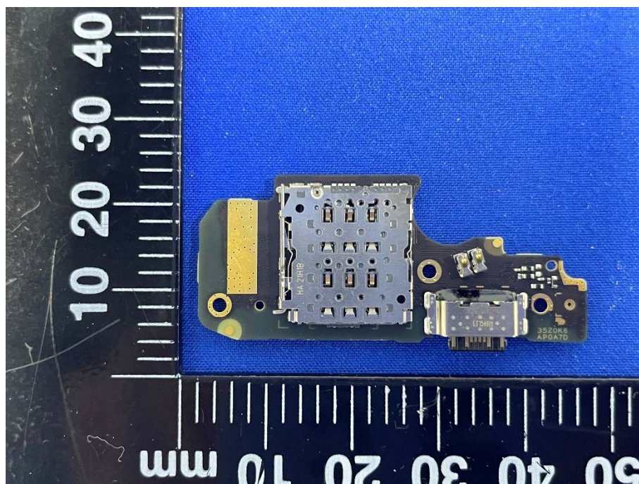
SECONDARY BOARD REAR VIEW
