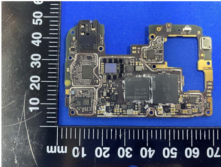
MAIN BOARD REAR VIEW (WITHOUT SHIELD COVER)
