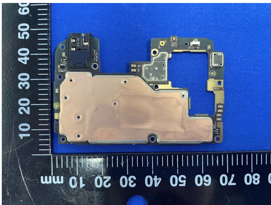
MAIN BOARD REAR VIEW (WITH SHIELD COVER)
