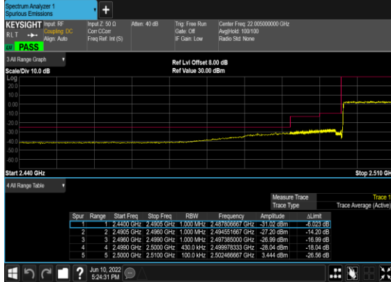
B66_N7(20M)_DFT-s- OFDM_QPSK_Outer_Full_Low_CH
