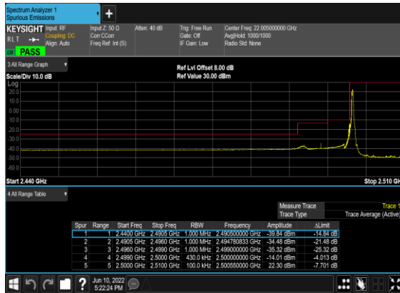
B66_N7(20M)_DFT-s- OFDM_BPSK_Edge_1RB_Left_Low_CH
