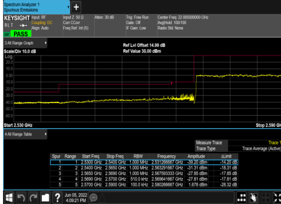
N38(25M)_DFT-s- OFDM_QPSK_Outer_Full_Low_CH
