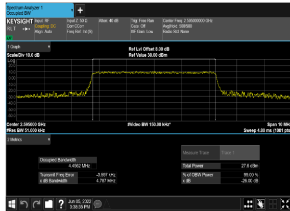
N38(5M)_CP-OFDM_16 QAM_Outer_Full_519000_CH
