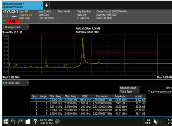
B66_N7(50M)_DFT-s- OFDM_BPSK_Edge_1RB_Right_High_CH
