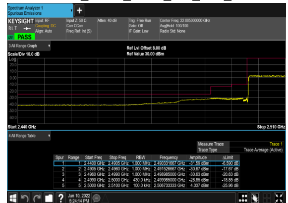
B66_N7(20M)_DFT-s- OFDM_BPSK_Outer_Full_Low_CH
