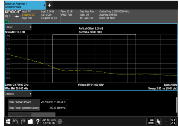
B66_N7(50M)_DFT-s- OFDM_BPSK_Edge_1RB_Right_High_CH_CHP_PASS
