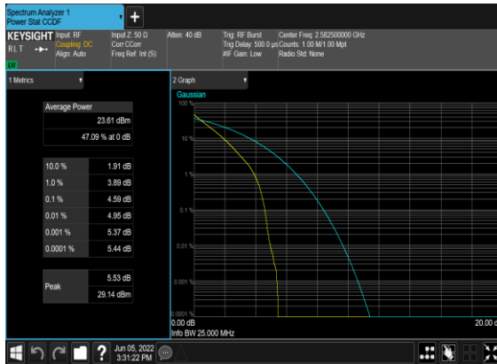
N38(25M)_DFT-s-OFDM_PI_2-BPSK_Outer_Full_Low_CH
