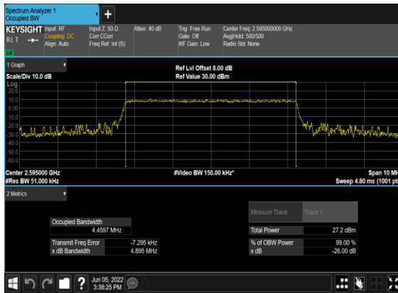
N38(5M)_CP- OFDM_QPSK_Outer_Full_519000_CH
