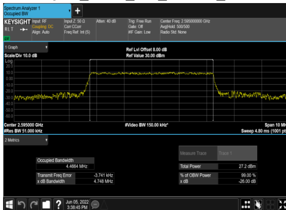
N38(5M)_CP-OFDM_64 QAM_Outer_Full_519000_CH
