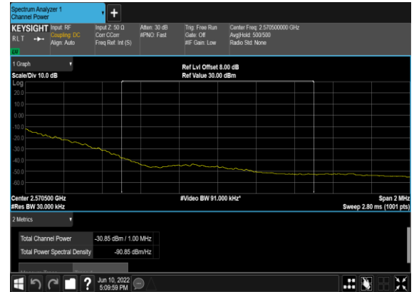
B66_N7(50M)_DFT-s- OFDM_QPSK_Edge_1RB_Right_High_CH_CHP_PASS
