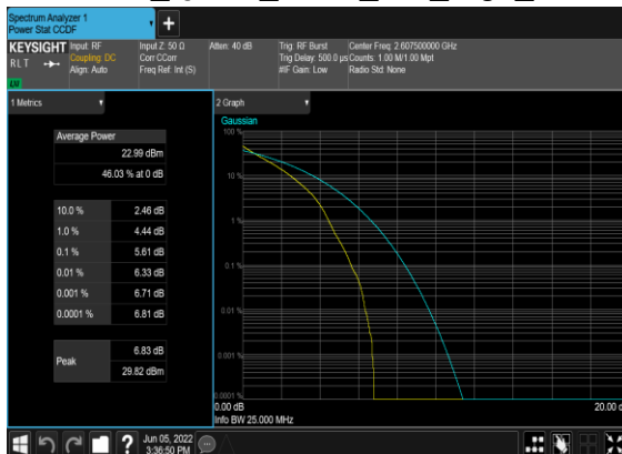
N38(25M)_DFT-s-OFDM_QPSK_Outer_Full_High_CH
