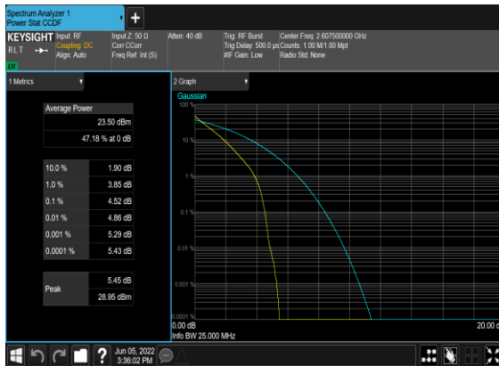
N38(25M)_DFT-s-OFDM_PI_2-BPSK_Outer_Full_High_CH
