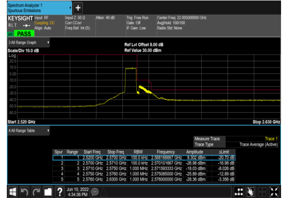
B66_N7(5M)_DFT-s- OFDM_QPSK_Outer_Full_High_CH
