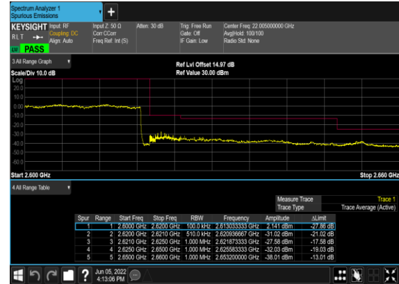
N38(25M)_DFT-s- OFDM_BPSK_Outer_Full_High_CH
