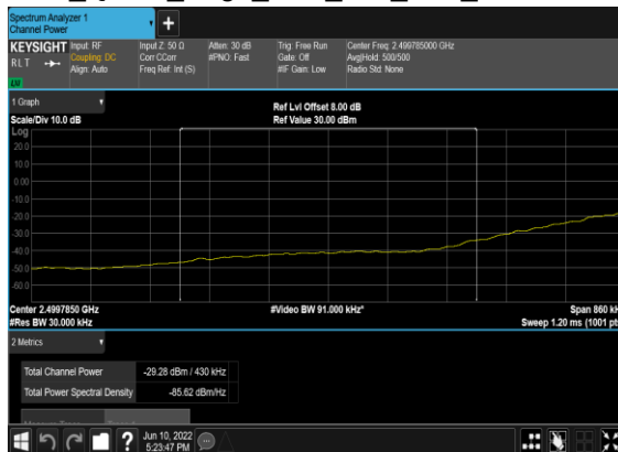
B66_N7(20M)_DFT-s- OFDM_QPSK_Edge_1RB_Left_Low_CH_chp_PASS
