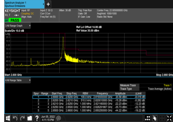
N38(25M)_DFT-s- OFDM_BPSK_Edge_1RB_Right_High_CH
