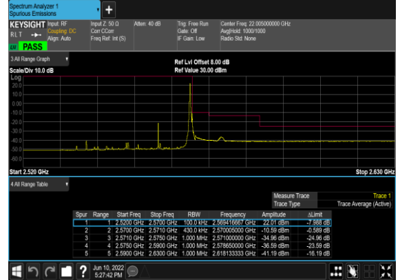
B66_N7(20M)_DFT-s- OFDM_BPSK_Edge_1RB_Right_High_CH
