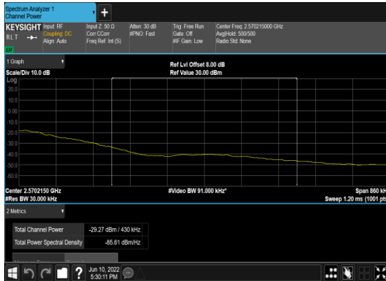
B66_N7(20M)_DFT-s- OFDM_QPSK_Edge_1RB_Right_High_CH_CHP_PASS
