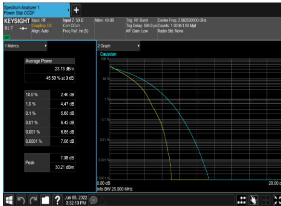
N38(25M)_DFT-s-OFDM_QPSK_Outer_Full_Low_CH
