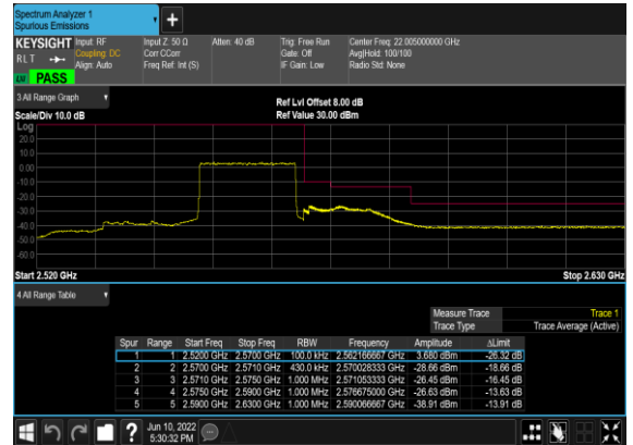
B66_N7(20M)_DFT-s- OFDM_BPSK_Outer_Full_High_CH
