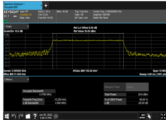
N38(5M)_DFT-s- OFDM_QPSK_Outer_Full_519000_CH
