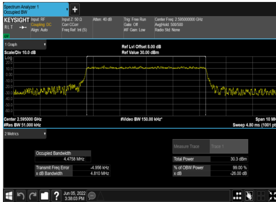
N38(5M)_DFT-s-OFDM_PI_2- BPSK_Outer_Full_519000_CH
