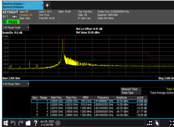
N38(25M)_DFT-s- OFDM_QPSK_Edge_1RB_Right_High_CH
