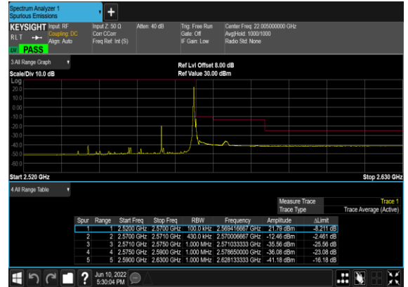
B66_N7(20M)_DFT-s- OFDM_QPSK_Edge_1RB_Right_High_CH
