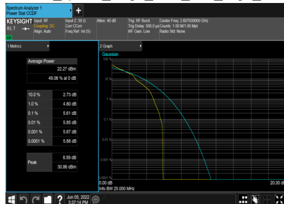
N38(25M)_DFT-s-OFDM_QPSK_Edge_1RB_Left_High_CH
