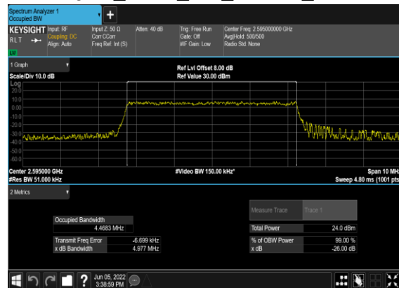
N38(5M)_CP-OFDM_256 QAM_Outer_Full_519000_CH
