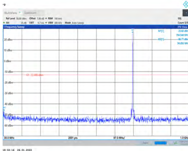
Band17-10MHz-16QAM-23780-1RB#0-Range4:1000~10000MHz
