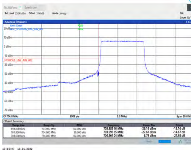
Band17-5MHz-QPSK-23755-25RB#0
