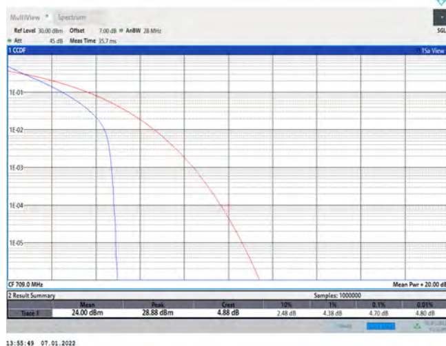
Band17-10MHz-QPSK-23790-50RB#0
