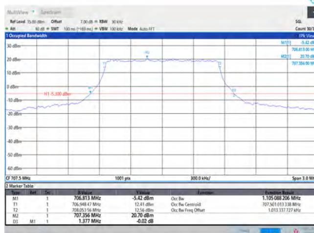
Band12-1.4MHz-QPSK-23095-6RB#0
