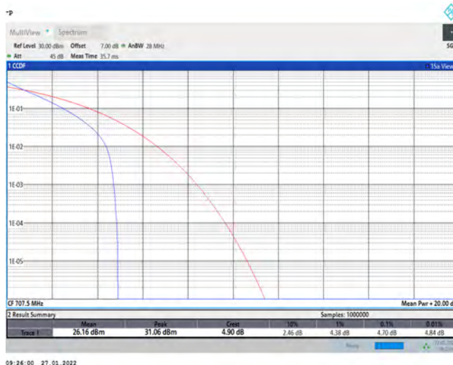
Band12-10MHz-QPSK-23095-50RB#0
