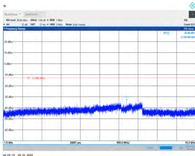
Band12-10MHz-256QAM-23060-1RB#0-Range1:0.009~0.15MHz
