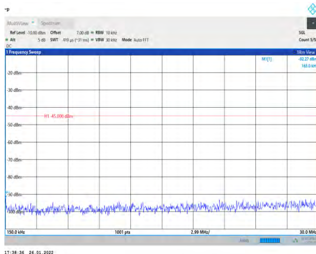
Band7-20MHz-64QAM-20850-1RB#0-Range3:30~1000MHz
