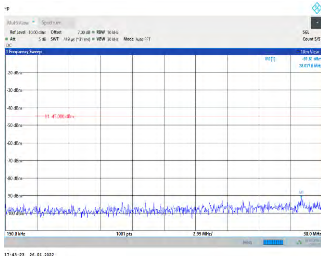
Band7-20MHz-256QAM-21100-1RB#0-Range2:0.15~30MHz
