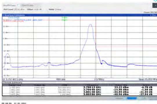
1-N78-3700-3800-PC2-30-15-H-5-CP-QPSK-Edge_1R B_Right-1@37-Ant1-PASS-see graph
