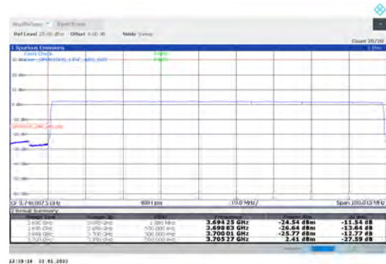
1-N78-3700-3800-PC2-30-90-L-6-CP-QPSK-Outer _Full-245@0-Ant1-PASS-see graph
