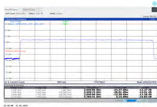
1-N78-3700-3800-PC2-30-90-L-3-DFT-PI2BPSK-Outer _Full-240@0-Ant1-PASS-see graph
