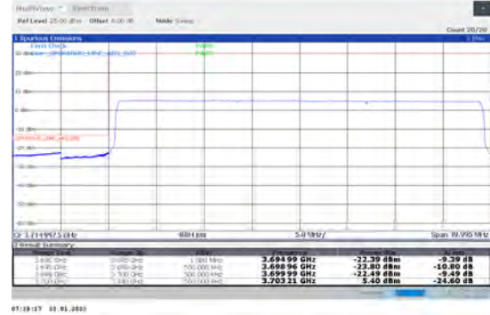
1-N78-3700-3800-PC2-30-40-L-6-CP-QPSK-Outer _Full-106@0-Ant1-PASS-see graph
