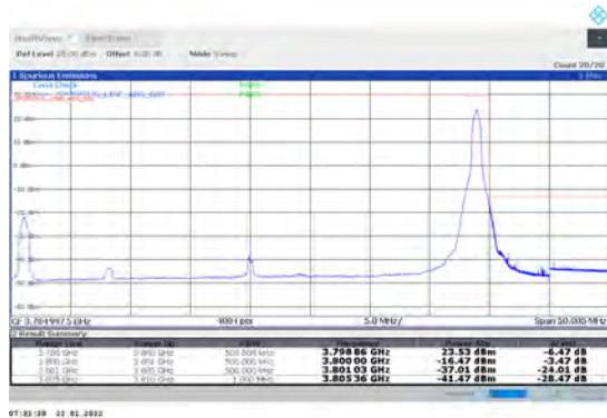
1-N78-3700-3800-PC2-30-40-H-5-CP-QPSK-Edge_1R B_Right-1@105-Ant1-PASS-see graph
