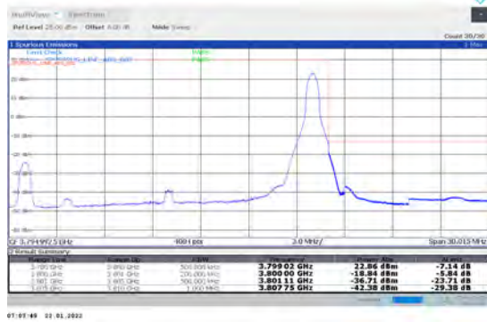
1-N78-3700-3800-PC2-30-20-H-5-CP-QPSK-Edge_1R B_Right-1@50-Ant1-PASS-see graph
