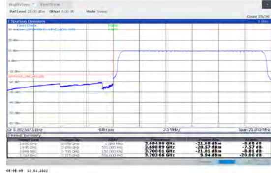
1-N78-3700-3800-PC2-30-15-L-6-CP-QPSK-Outer _Full-38@0-Ant1-PASS-see graph
