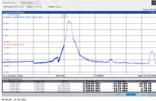
1-N78-3700-3800-PC2-30-15-L-4-CP-QPSK-Edge_1R B_Left-1@0-Ant1-PASS-see graph
