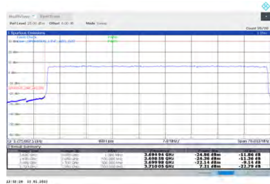
1-N78-3700-3800-PC2-30-60-L-3-DFT-PI2BPSK-Outer _Full-162@0-Ant1-PASS-see graph
