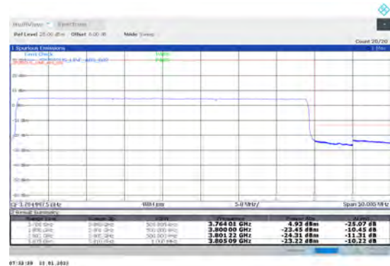
1-N78-3700-3800-PC2-30-40-H-6-CP-QPSK-Outer _Full-106@0-Ant1-PASS-see graph
