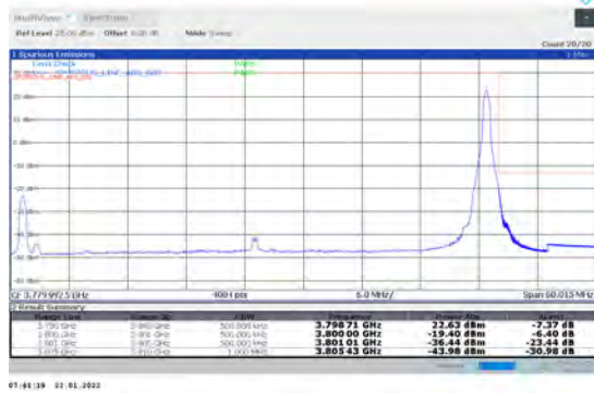
1-N78-3700-3800-PC2-30-50-H-5-CP-QPSK-Edge_1R B_Right-1@132-Ant1-PASS-see graph
