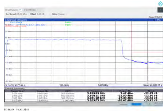
1-N78-3700-3800-PC2-30-40-H-3-DFT-PI2BPSK-Outer _Full-100@0-Ant1-PASS-see graph
