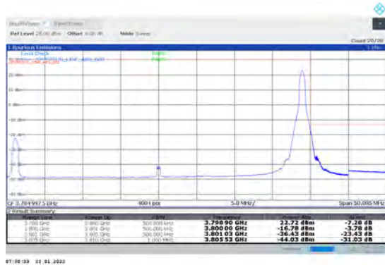
1-N78-3700-3800-PC2-30-40-H-2-DFT-PI2BPSK-Edge _1RB_Right-1@105-Ant1-PASS-see graph
