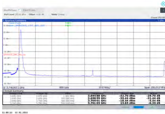
1-N78-3700-3800-PC2-30-90-L-1-DFT-PI2BPSK-Edge _1RB_Left-1@0-Ant1-PASS-see graph
