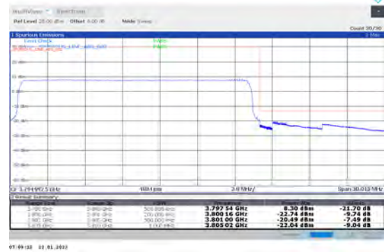
1-N78-3700-3800-PC2-30-20-H-3-DFT-QPSK-Out er_Full-50@0-Ant1-PASS-see graph
