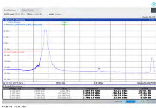
1-N78-3700-3800-PC3-30-30-L-1-DFT-PI2BPSK-Edge _1RB_Left-1@0-Ant1-PASS-see graph
