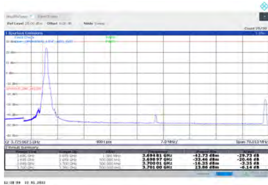
1-N78-3700-3800-PC2-30-60-L-1-DFT-PI2BPSK-Edge _1RB_Left-1@0-Ant1-PASS-see graph
