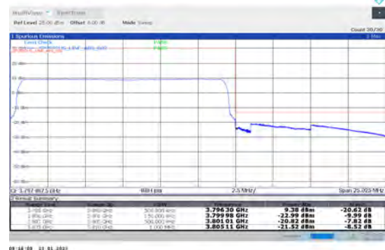
1-N78-3700-3800-PC2-30-15-H-6-CP-QPSK-Outer _Full-38@0-Ant1-PASS-see graph
