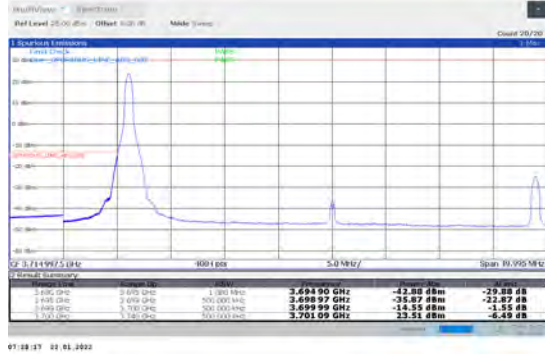
1-N78-3700-3800-PC2-30-40-L-4-CP-QPSK-Edge_1R B_Left-1@0-Ant1-PASS-see graph
