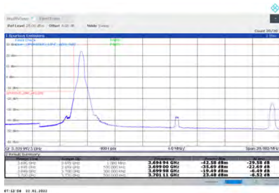
1-N78-3700-3800-PC3-30-30-L-4-CP-QPSK-Edge_1R B_Left-1@0-Ant1-PASS-see graph
