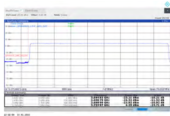
1-N78-3700-3800-PC2-30-60-L-6-CP-QPSK-Outer _Full-162@0-Ant1-PASS-see graph
