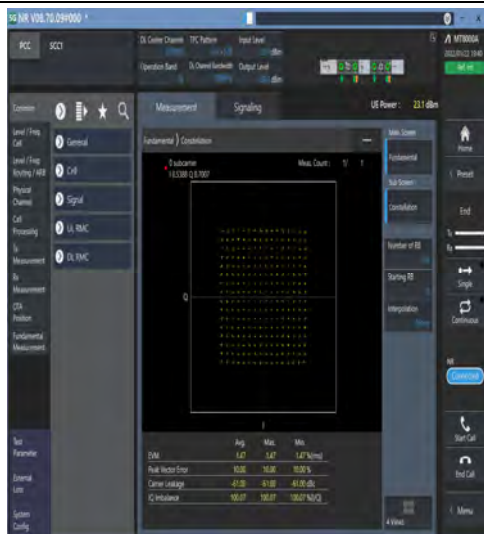
1-N78-3700-3800-PC2-30-100-M-5-DFT-256QAM-Ou ter_Full-270@0-Ant1-see graph-PASS
