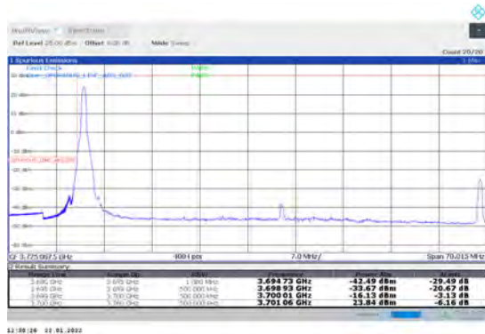
1-N78-3700-3800-PC2-30-60-L-4-CP-QPSK-Edge_1R B_Left-1@0-Ant1-PASS-see graph
