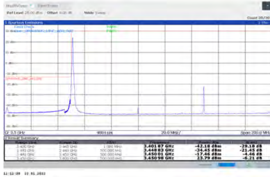
1-N78-3450-3550-PC2-30-100-L-1-DFT-PI2BPSK-Edge_1RB_Left-1@0-Ant1-PASS-see graph
