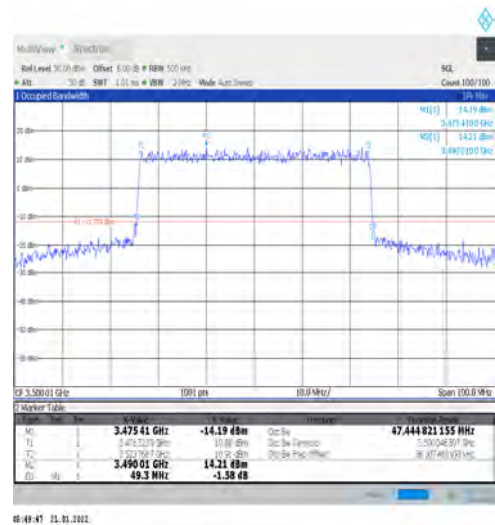
1-N78-3450-3550-PC2-30-50-M-7-CP-16QAM-Outer_Full-133@0-Ant1-47.445-49.300-≤50-PASS
