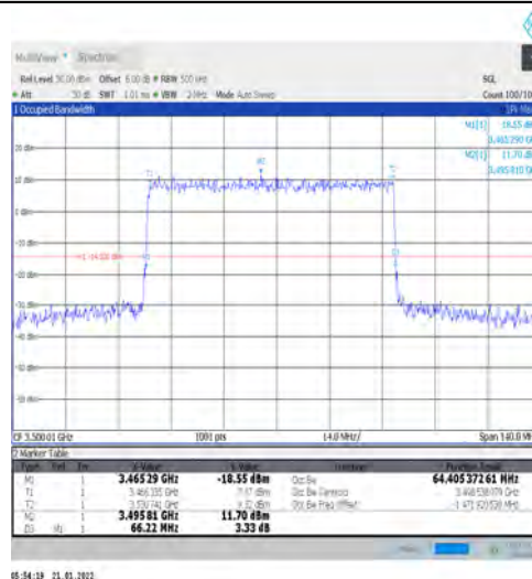
1-N78-3450-3550-PC2-30-70-M-5-DFT-256QAM-Out_Full-Outer_Full@N/A-Ant1-64.405-66.220-≤70-P ASS
