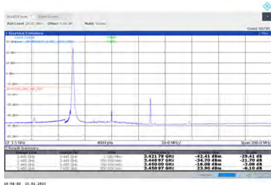
1-N78-3450-3550-PC2-30-60-L-4-CP-QPSK-Edge_1R B Left-1@0-Ant1-PASS-see graph
