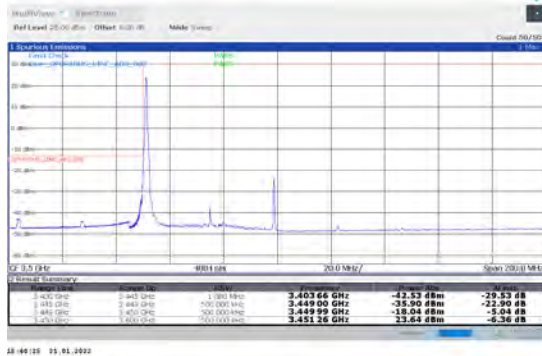
1-N78-3450-3550-PC2-30-50-L-4-CP-QPSK-Edge_1RB_Left-1@0-Ant1-PASS-see graph
