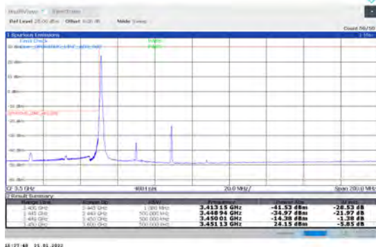
1-N78-3450-3550-PC2-30-40-L-4-CP-QPSK-Edge_1R_B_Left-1@0-Ant1-PASS-see graph
