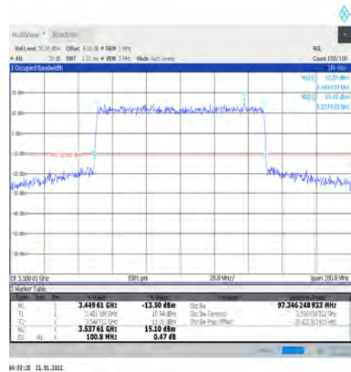
1-N78-3450-3550-PC2-30-100-M-6-CP-QPSK-Outer _Full-273@0-Ant1-97.346-100.800-≤100-PASS
