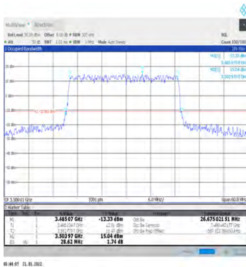
1-N78-3450-3550-PC2-30-30-M-4-DFT-64QAM-Outer_Full-75@0-Ant1-26.677-28.620-≤30-PASS
