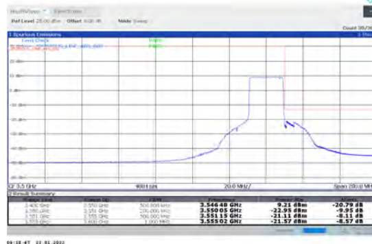
1-N78-3450-3550-PC2-30-20-H-6-CP-QPSK-Outer _Full-51@0-Ant1-PASS-see graph
