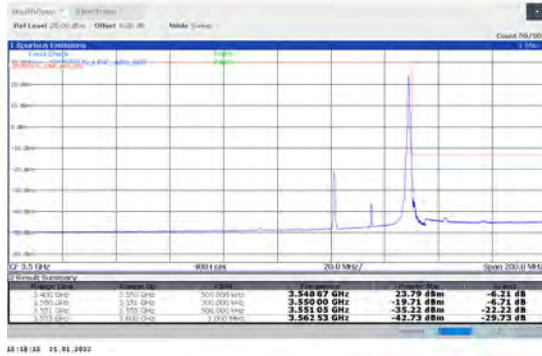
1-N78-3450-3550-PC2-30-30-H-2-DFT-PI2BPSK-Edge_1RB_Right-1@77-Ant1-PASS-see graph
