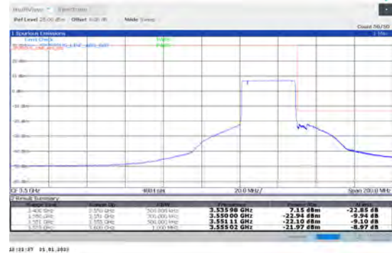
1-N78-3450-3550-PC2-30-30-H-6-CP-QPSK-Outer_Full-78@0-Ant1-PASS-see graph
