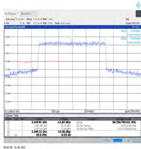
1-N78-3450-3550-PC2-30-100-M-4-DFT-64QAM-Ou ter_Full-270@0-Ant1-96.357-99.800-≤100-PASS
