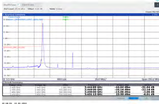
1-N78-3450-3550-PC2-30-40-L-1-DFT-PI2BPSK-Edge_1RB_Left-1@0-Ant1-PASS-see graph
