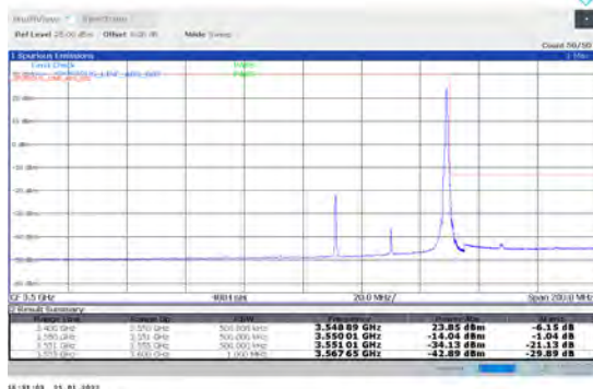
1-N78-3450-3550-PC2-30-40-H-2-DFT-PI2BPSK-Edge_1RB_Right-1@105-Ant1-PASS-see graph
