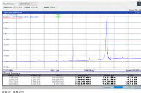
1-N78-3450-3550-PC2-30-50-H-2-DFT-PI2BPSK-Edge_1RB_Right-1@132-Ant1-PASS-see graph
