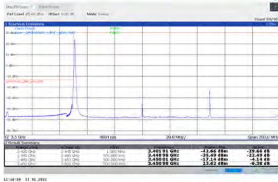
1-N78-3450-3550-PC2-30-100-L-4-CP-QPSK-Edge_1RB_Left-1@0-Ant1-PASS-see graph
