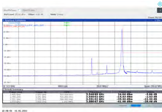
1-N78-3450-3550-PC2-30-40-H-5-CP-QPSK-Edge_1R_B_Right-1@105-Ant1-PASS-see graph
