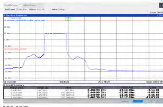
1-N78-3450-3550-PC2-30-30-L-3-DFT-PI2BPSK-Outer _Full-75@0-Ant1-PASS-see graph
