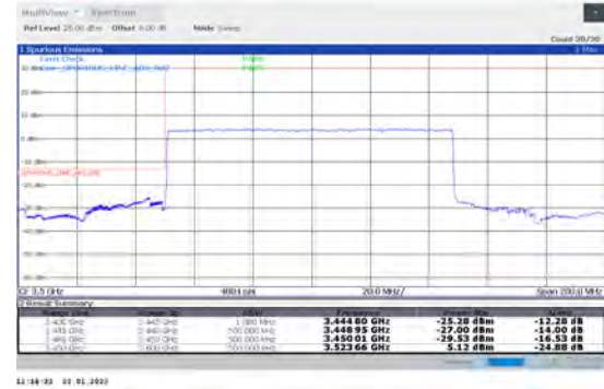
1-N78-3450-3550-PC2-30-100-L-3-DFT-PI2BPSK-Outer_Full-270@0-Ant1-PASS-see graph
