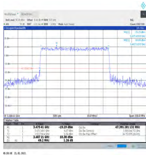
1-N78-3450-3550-PC2-30-50-M-9-CP-256QAM-Outer_Full-133@0-Ant1-47.391-49.200-≤50-PASS
