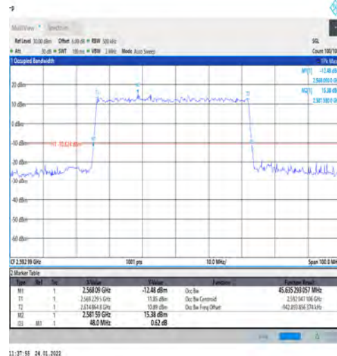
1-N41-PC3-30-50-M-3-DFT-16QAM-Outter_Full-128 @0-Ant1-45.635-48.000-≤50-PASS
