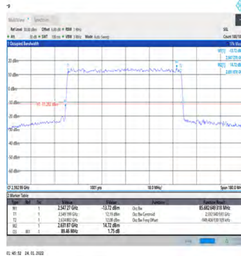
1-N41-PC3-30-90-M-3-DFT-16QAM-Outer_Full-240 @0-Ant1-85.683-89.460-≤90-PASS
