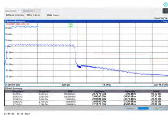
1-N41-PC3-30-20-H-6-CP-QPSK-Outer_Full-51@0-Ant1-PASS-see graph
