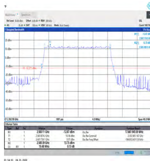
1-N41-PC3-30-20-M-4-DFT-64QAM-Outer_Full-50@ 0-Ant1-17.862-19.480-≤20-PASS
