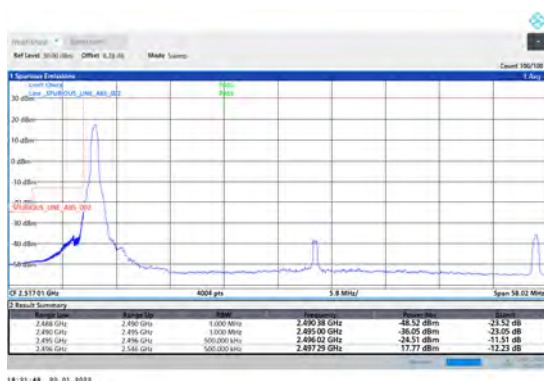
1-N41-PC3-30-50-L-4-CP-QPSK-Edge_1RB_Left-1 @0-Ant1-PASS-see graph
