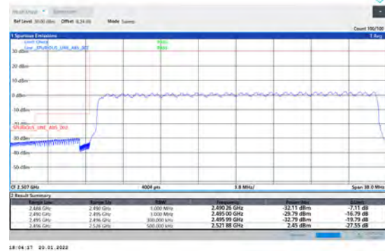
1-N41-PC3-30-30-L-6-CP-QPSK-Outer_Full-78@0-A nt1-PASS-see graph
