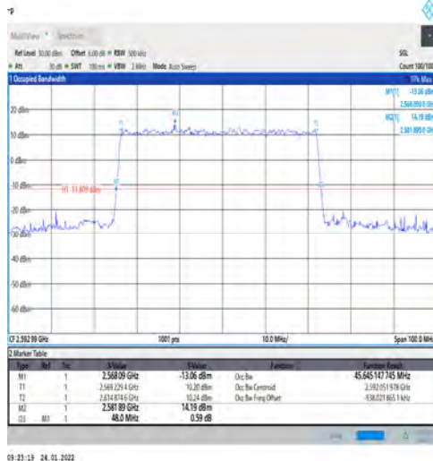
1-N41-PC3-30-50-M-2-DFT-PI2BPSK-Outter_Full-12 8@0-Ant1-45.645-48.000-≤50-PASS
