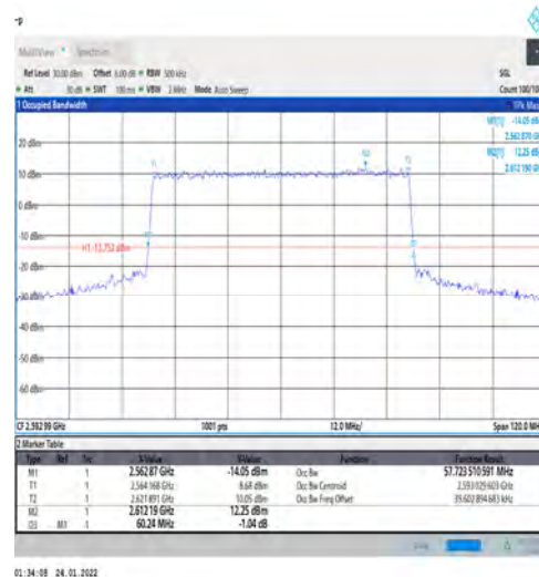
1-N41-PC3-30-60-M-8-CP-64QAM-Outet_Full-162@ 0-Ant1-57.724-60.240-≤60-PASS
