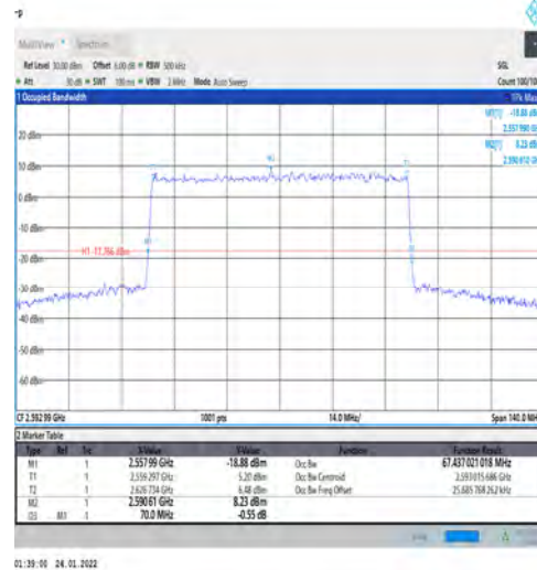
1-N41-PC3-30-70-M-9-CP-256QAM-Outer_Full-Outer_Full@N/A-Ant1-67.437-70.000-≤70-PASS
