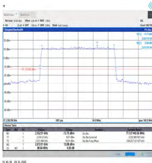
1-N41-PC3-30-80-M-5-DFT-256QAM-Outer_Full-216 @0-Ant1-77.127-80.640-≤80-PASS
