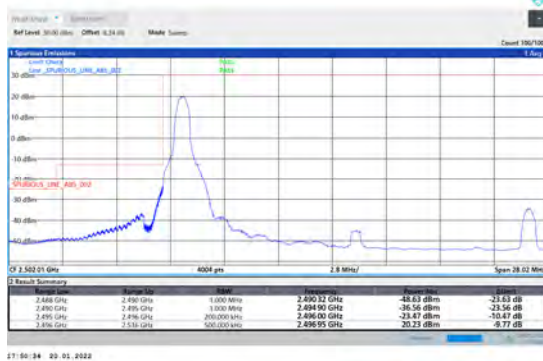
1-N41-PC3-30-20-L-1-DFT-PI2BPSK-Edge_1RB_Left-1@0-Ant1-PASS-see graph
