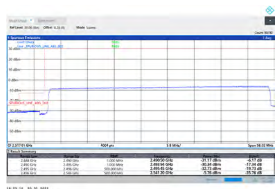
1-N41-PC3-30-50-L-6-CP-QPSK-Outer_Full-133@0-Ant1-PASS-see graph
