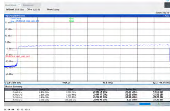
1-N41-PC3-30-100-L-6-CP-QPSK-Outer_Full-273@0-Ant1-PASS-see graph
