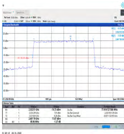
1-N41-PC3-30-80-M-9-CP-256QAM-Outer_Full-217 @0-Ant1-77.42-80.960-≤80-PASS
