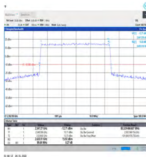
1-N41-PC3-30-90-M-1-DFT-QPSK-Outer_Full-240@ 0-Ant1-85.524-89.640-≤90-PASS
