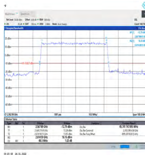
1-N41-PC3-30-50-M-1-DFT-QPSK-Outer_Full-128@ 0-Ant1-45.742-48.300-≤50-PASS
