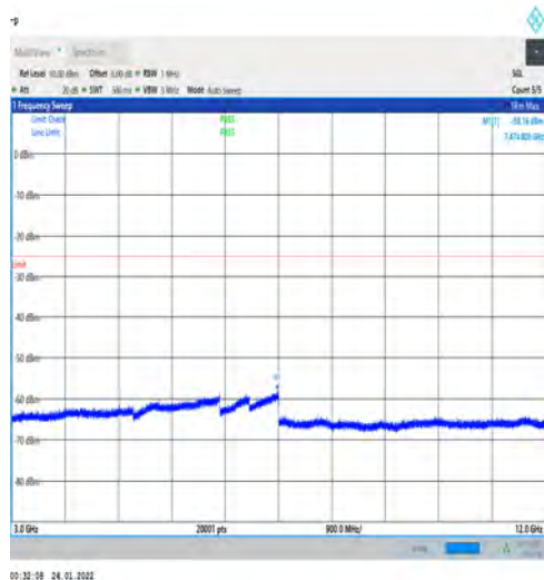
1-N41-PC3-30-100-M-1-DFT-PI2BPSK-Edge_1RB_L Left-1@0-3000-12000-Ant1--58.16--25-PASS
