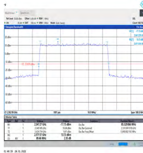
1-N41-PC3-30-90-M-5-DFT-256QAM-Outer_Full-240 @0-Ant1-85.529-89.460-≤90-PASS
