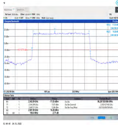
1-N41-PC3-30-100-M-2-DFT-PI2BPSK-Outter_Full-270 @0-Ant1-96.287-100.400-≤100-PASS
