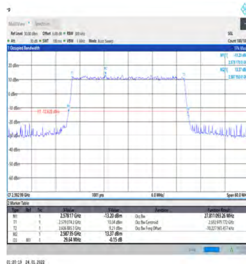
1-N41-PC3-30-30-M-7-CP-16QAM-Outer_Full-78@0- Ant1-27.811-29.640-≤30-PASS
