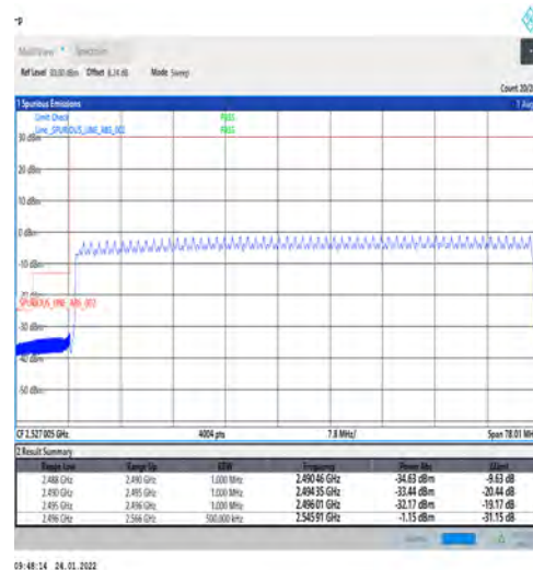
1-N41-PC3-30-70-L-6-CP-QPSK-Outer_Full-Outer_Full@N/A-Ant1-PASS-see graph
