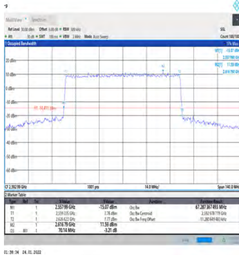
1-N41-PC3-30-70-M-8-CP-64QAM-Outer_Full-Outer_Full@N/A-Ant1-67.287-70.140-≤70-PASS
