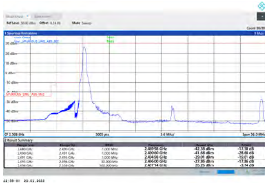
1-N41-PC3-30-40-L-1-CP-QPSK -Edge_1RB_Left-1@0-Ant1-PASS-see graph
