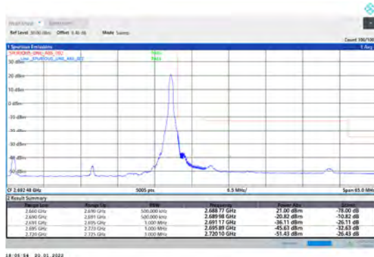
1-N41-PC3-30-30-H-2-DFT-PI2BPSK-Edge_1RB_Right-1@77-Ant1-PASS-see graph
