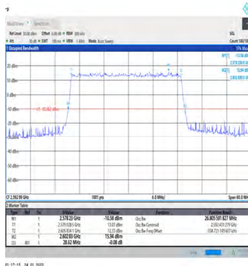
1-N41-PC3-30-30-M-1-DFT-QPSK-Outer_Full-75@0- Ant1-26.806-28.620-≤30-PASS
