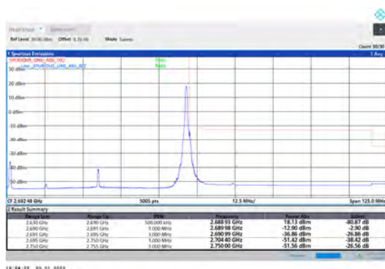
1-N41-PC3-30-60-H-5-CP-QPSK-Edge_1RB_Right-1@161-Ant1-PASS-see graph
