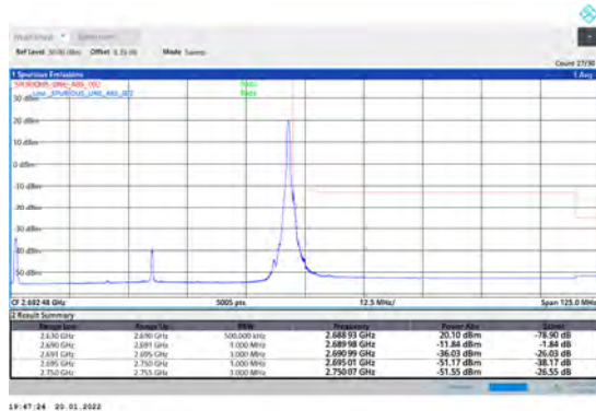
1-N41-PC3-30-60-H-2-DFT-PI2BPSK-Edge_1RB_Right-1@161-Ant1-PASS-see graph
