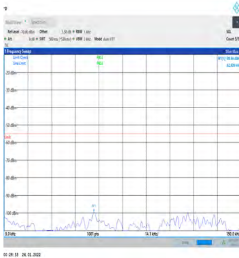
1-N41-PC3-30-100-L-1-DFT-PI2BPSK-Edge_1RB_L eft-1@0-0.009-0.15-Ant1--99.46--55-PASS
