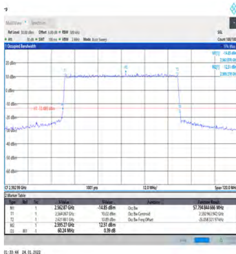
1-N41-PC3-30-60-M-7-CP-16QAM-Outet_Full-162@ 0-Ant1-57.795-60.240-≤60-PASS
