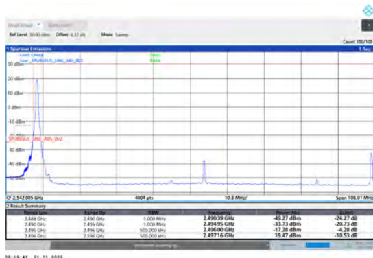
1-N41-PC3-30-100-L-1-DFT-PI2BPSK-Edge_1RB_Left-1@0-Ant1-PASS-see graph
