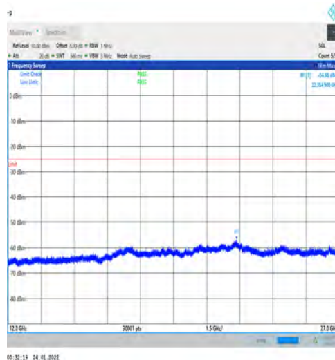
1-N41-PC3-30-100-M-1-DFT-PI2BPSK-Edge_1RB_L eft-1@0-12000-27000-Ant1--56.98--25-PASS
