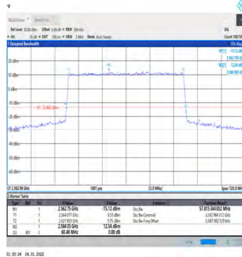
1-N41-PC3-30-60-M-6-CP-QPSK-Outet_Full-162@0 -Ant1-57.815-60.480-≤60-PASS
