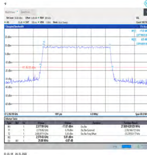
1-N41-PC3-30-30-M-9-CP-256QAM-Outer_Full-78@0-Ant1-27.809-29.880-≤30-PASS
