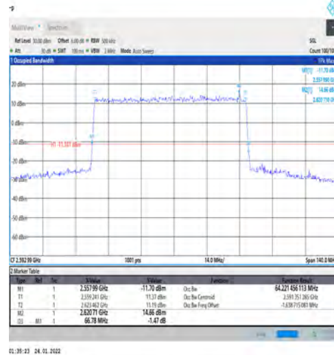
1-N41-PC3-30-70-M-1-DFT-QPSK-Outer_Full-Outer_Full@N/A-Ant1-64.221-66.780-≤70-PASS
