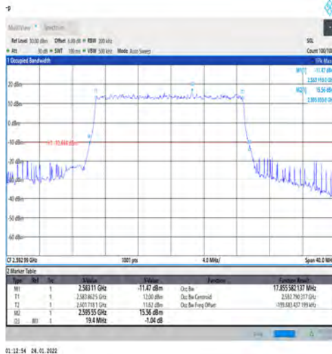
1-N41-PC3-30-20-M-1-DFT-QPSK-Outer_Full-50@0 -Ant1-17.856-19.400-≤20-PASS
