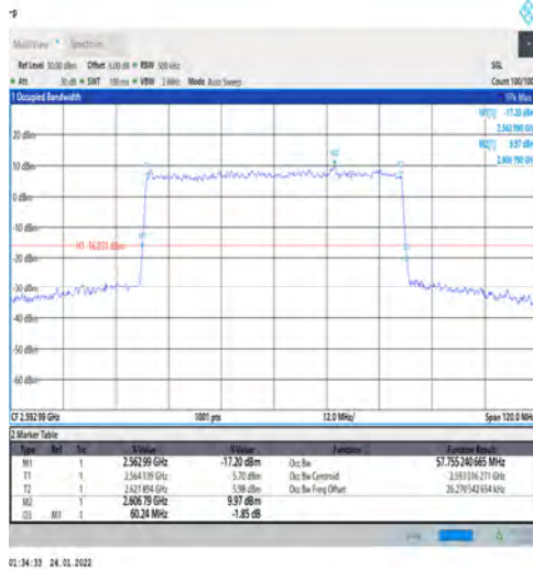
1-N41-PC3-30-60-M-9-CP-256QAM-Outer_Full-162 @0-Ant1-57.755-60.240-≤60-PASS
