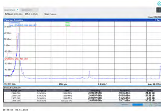
1-N41-PC3-30-90-L-1-DFT-PI2BPSK-Edge_1RB_Lef t-1@0-Ant1-PASS-see graph
