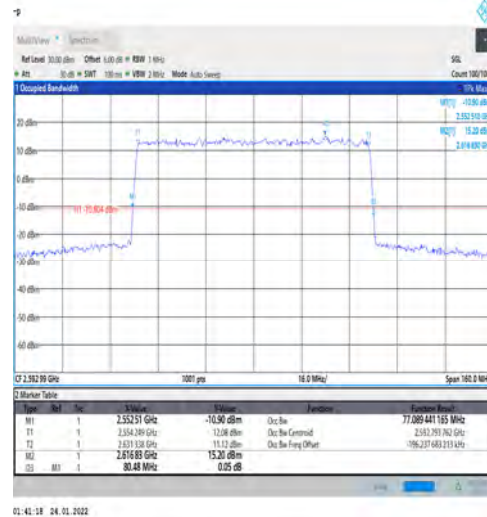
1-N41-PC3-30-80-M-4-DFT-64QAM-Outer_Full-216 @0-Ant1-77.089-80.480-≤80-PASS
