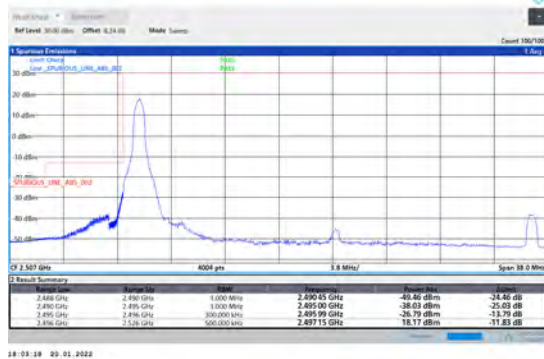
1-N41-PC3-30-30-L-4-CP-QPSK-Edge_1RB_Left-1 @0-Ant1-PASS-see graph
