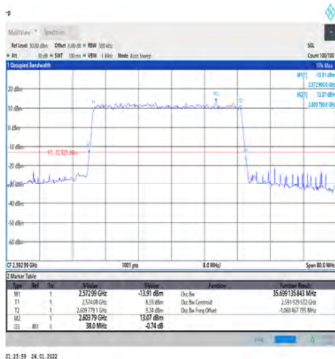
1-N41-PC3-30-40-M-5-DFT-256QAM-Outer_Full-100 @0-Ant1-35.699-38.000-≤40-PASS
