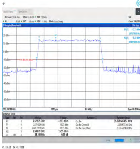
1-N41-PC3-30-40-M-3-DFT-16QAM-Outer_Full-100 @0-Ant1-35.699-38.160-≤40-PASS
