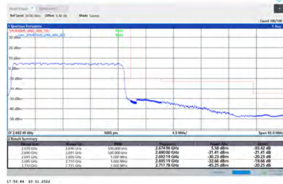
1-N41-PC3-30-20-H-3-DFT-PI2BPSK-Outer_Full-50@0-Ant1-PASS-see graph
