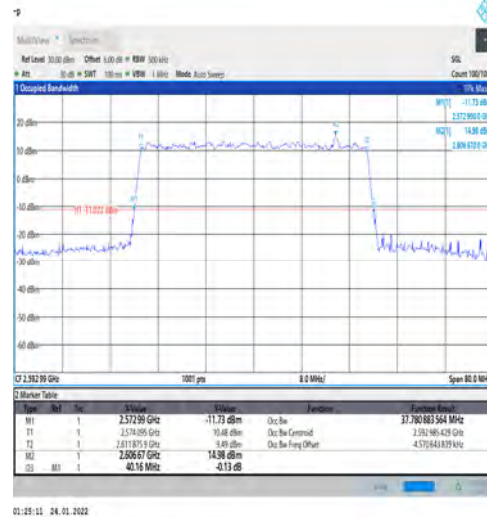
1-N41-PC3-30-40-M-8-CP-64QAM-Outer_Full-106@ 0-Ant1-37.781-40.160-≤40-PASS
