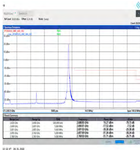
1-N41-PC3-30-70-H-5-CP-QPSK-Edge_1RB_Right- Edge_1_Right@N/A-Ant1-PASS-see graph
