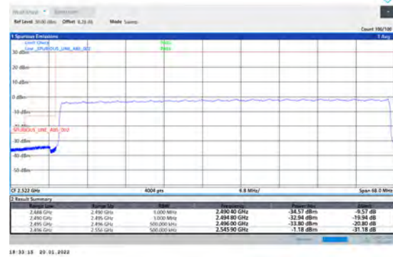
1-N41-PC3-30-60-L-6-CP-QPSK-Outer_Full-162@0 Ant1-PASS-see graph
