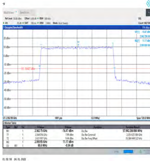
1-N41-PC3-30-60-M-5-DFT-256QAM-Outet_Full-162@ @0-Ant1-57.942-60.600-≤60-PASS
