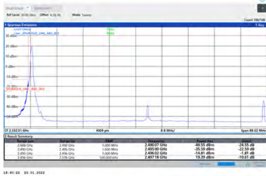
1-N41-PC3-30-80-L-1-DFT-PI2BPSK-Edge_1RB_Lef t-1@0-Ant1-PASS-see graph
