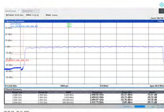
1-N41-PC3-30-60-L-3-DFT-PI2BPSK-Outer_Full-162 @0-Ant1-PASS-see graph
