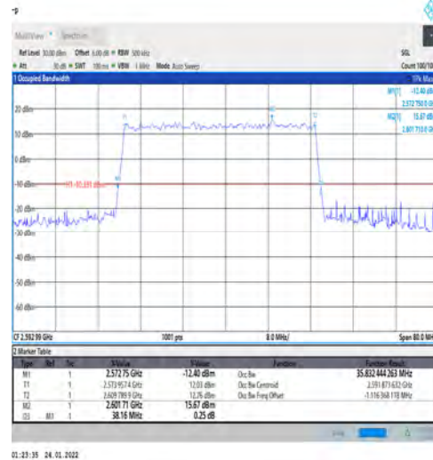
1-N41-PC3-30-40-M-4-DFT-64QAM-Outer_Full-100 @0-Ant1-35.832-38.160-≤40-PASS
