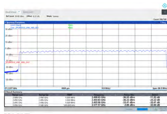
1-N41-PC3-30-90-L-6-CP-QPSK-Outer_Full-245@0-Ant1-PASS-see graph
