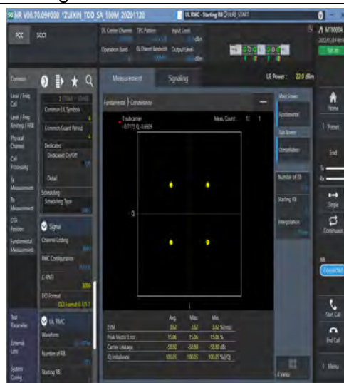
1-N41-PC3-30-100-M-6-CP-QPSK-Outer_Full-273 @0-Ant1-see graph-PASS
