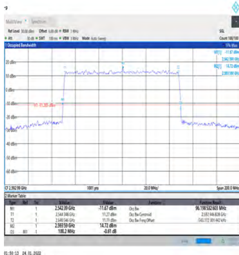
1-N41-PC3-30-100-M-3-DFT-16QAM-Outter_Full-270 @0-Ant1-96.199-100.200-≤100-PASS
