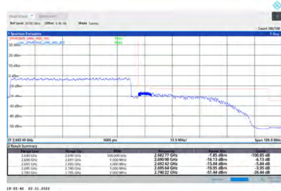
1-N41-PC3-30-50-H-3-DFT-PI2BPSK-Outer_Full-12 8@0-Ant1-PASS-see graph
