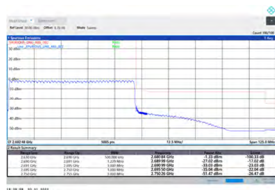
1-N41-PC3-30-60-H-6-CP-QPSK-Outer_Full-162@0 -Ant1-PASS-see graph
