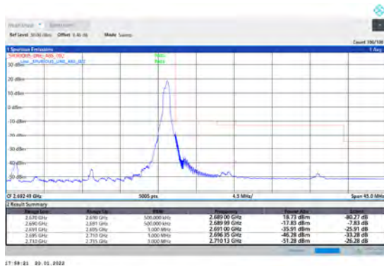
1-N41-PC3-30-20-H-5-CP-QPSK-Edge_1RB_Right-1@50-Ant1-PASS-see graph
