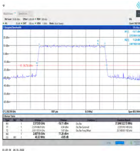
1-N41-PC3-30-40-M-9-CP-256QAM-Outer_Full-106@ 0-Ant1-37.847-40.320-≤40-PASS
