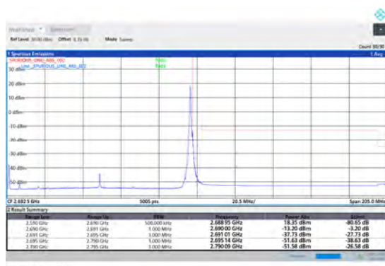
1-N41-PC3-30-100-H-5-CP-QPSK-Edge_1RB_Right-1@272-Ant1-PASS-see graph
