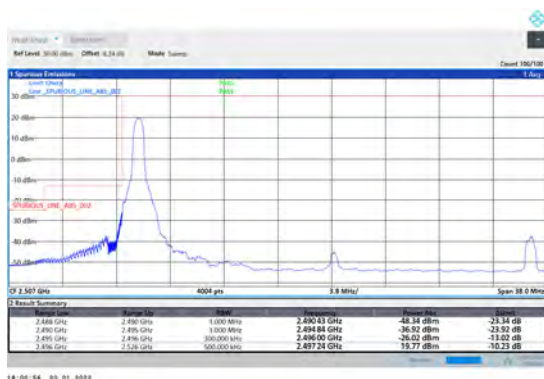
1-N41-PC3-30-30-L-1-DFT-PI2BPSK-Edge_1RB_Left-1@0-Ant1-PASS-see graph
