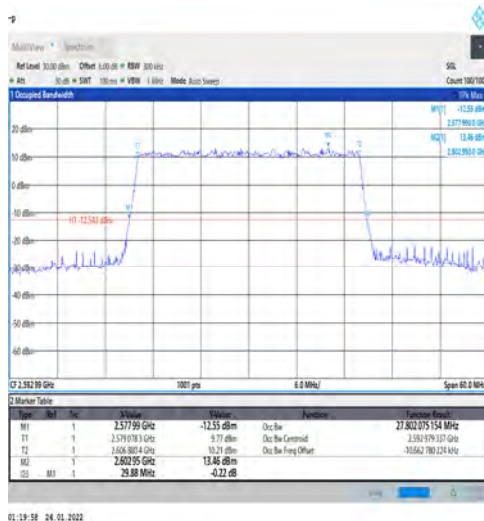
1-N41-PC3-30-30-M-6-CP-QPSK-Outer_Full-78@0- Ant1-27.802-29.880-≤30-PASS
