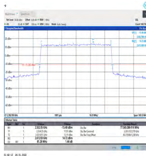
1-N41-PC3-30-80-M-6-CP-QPSK-Outer_Full-217@0 -Ant1-77.565-81.280-≤80-PASS
