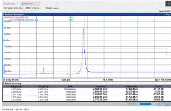
1-N41-PC3-30-80-H-5-CP-QPSK-Edge_1RB_Right-1 @216-Ant1-PASS-see graph
