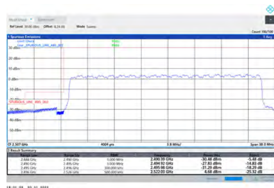
1-N41-PC3-30-30-L-3-DFT-PI2BPSK-Outer_Full-75@0-Ant1-PASS-see graph
