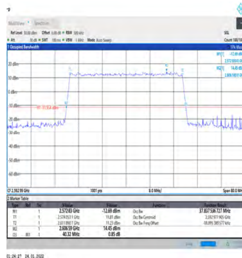
1-N41-PC3-30-40-M-6-CP-QPSK-Outer_Full-106@0 -Ant1-37.838-40.320-≤40-PASS
