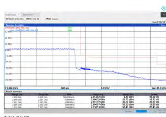
1-N41-PC3-30-40-H-3-DFT-PI2BPSK-Outer_Full-10 0@0-Ant1-PASS-see graph
