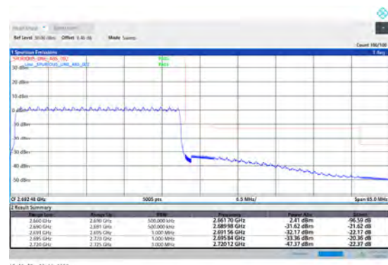
1-N41-PC3-30-30-H-6-CP-QPSK-Outer_Full-78@0-Ant1-PASS-see graph
