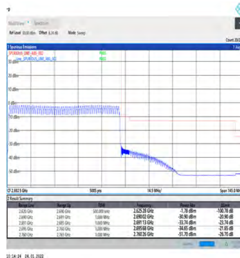
1-N41-PC3-30-70-H-6-CP-QPSK-Outer_Full-Outer_ Full@N/A-Ant1-PASS-see graph
