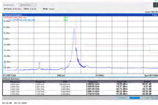
1-N41-PC3-30-40-H-5-CP-QPSK-Edge_1RB_Right-1@105-Ant1-PASS-see graph
