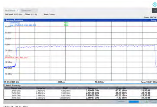
1-N41-PC3-30-100-L-3-DFT-PI2BPSK-Outer_Full-270@0-Ant1-PASS-see graph
