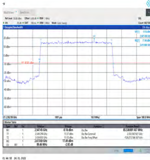
1-N41-PC3-30-90-M-2-DFT-PI2BPSK-Outer_Full-240 @0-Ant1-85.539-89.460-≤90-PASS
