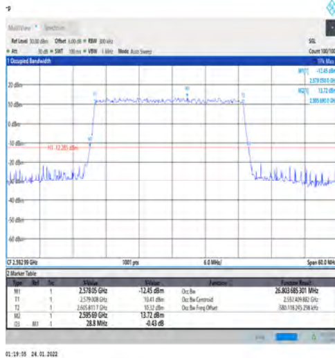
1-N41-PC3-30-30-M-4-DFT-64QAM-Outer_Full-75@ 0-Ant1-26.804-28.800-≤30-PASS
