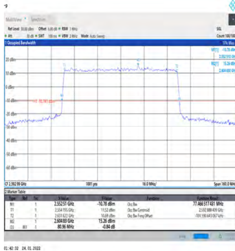
1-N41-PC3-30-80-M-7-CP-16QAM-Outer_Full-217@ 0-Ant1-77.467-80.960-≤80-PASS
