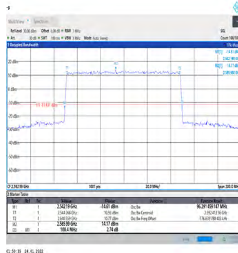
1-N41-PC3-30-100-M-4-DFT-64QAM-Outter_Full-270 @0-Ant1-96.291-100.400-≤100-PASS
