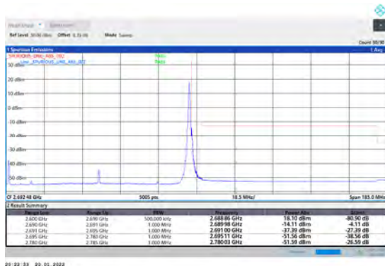
1-N41-PC3-30-90-H-5-CP-QPSK-Edge_1RB_Right-1@244-Ant1-PASS-see graph
