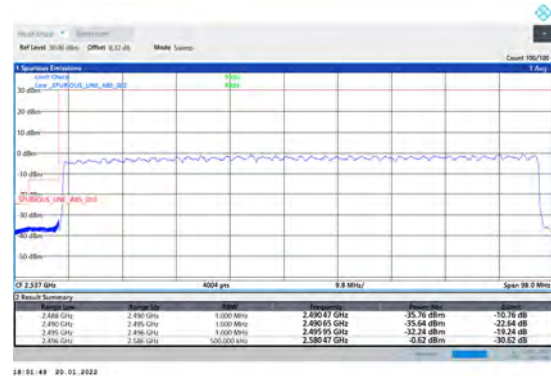
1-N41-PC3-30-90-L-3-DFT-PI2BPSK-Outer_Full-240 @0-Ant1-PASS-see graph
