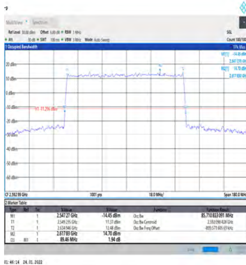
1-N41-PC3-30-90-M-4-DFT-64QAM-Outer_Full-240 @0-Ant1-85.711-89.460-≤90-PASS
