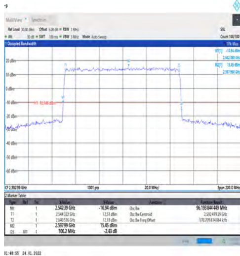
1-N41-PC3-30-100-M-1-DFT-QPSK-Outter_Full-270 @0-Ant1-96.194-100.200-≤100-PASS
