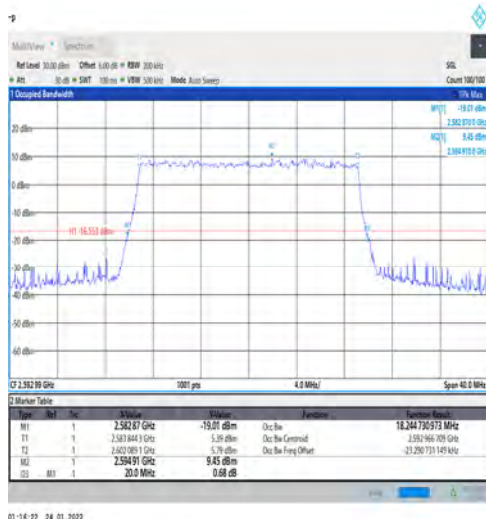
1-N41-PC3-30-20-M-9-CP-256QAM-Outer_Full-51@ 0-Ant1-18.245-20.000-≤20-PASS
