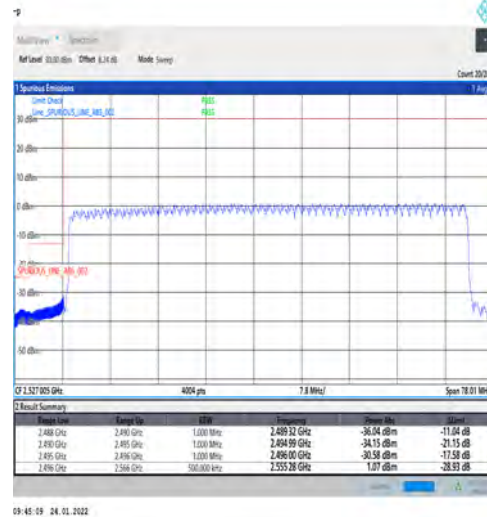
1-N41-PC3-30-70-L-3-DFT-PI2BPSK-Outer_Full-Out-er_Full@N/A-Ant1-PASS-see graph
