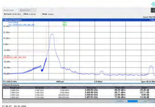
1-N41-PC3-30-20-L-4-CP-QPSK-Edge_1RB_Left-1@0-Ant1-PASS-see graph
