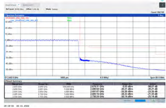
1-N41-PC3-30-40-H-6-CP-QPSK-Outer_Full-106@0-Ant1-PASS-see graph
