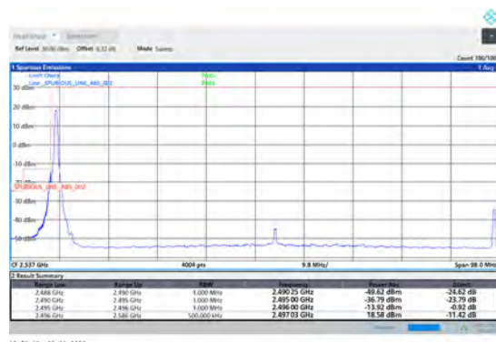
1-N41-PC3-30-90-L-4-CP-QPSK-Edge_1RB_Left-1 @0-Ant1-PASS-see graph
