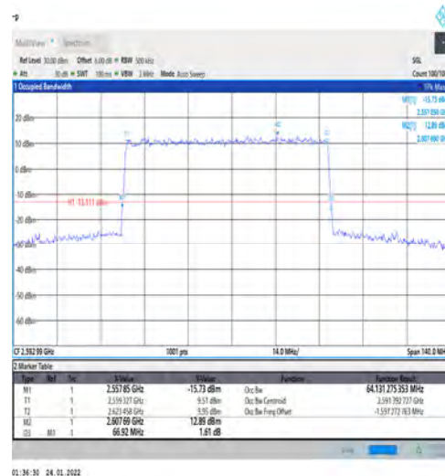
1-N41-PC3-30-70-M-3-DFT-16QAM-Outer_Full-Outer_Full@N/A-Ant1-64.131-66.920-≤70-PASS
