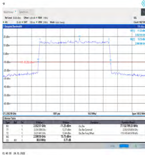
1-N41-PC3-30-80-M-3-DFT-16QAM-Outer_Full-216 @0-Ant1-77.133-80.800-≤80-PASS
