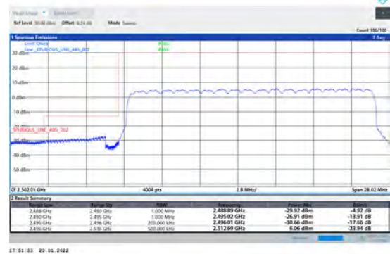
1-N41-PC3-30-20-L-3-DFT-PI2BPSK-Outer_Full-50@0-Ant1-PASS-see graph
