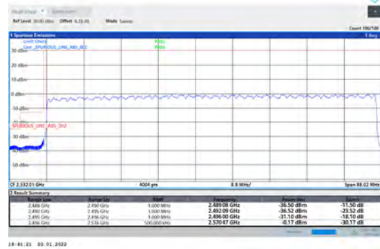
1-N41-PC3-30-80-L-3-DFT-PI2BPSK-Outer_Full-216 @0-Ant1-PASS-see graph
