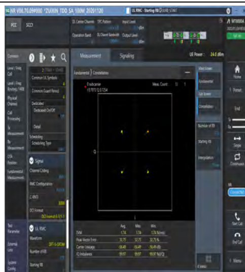
1-N41-PC3-30-100-M-2-DFT-QPSK-Outer_Full-270 0@0-Ant1-see graph-PASS
