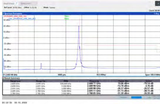
1-N41-PC3-30-90-H-2-DFT-PI2BPSK-Edge_1RB_Right-1@244-Ant1-PASS-see graph
