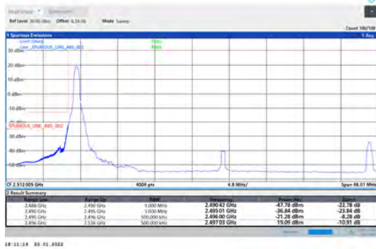
1-N41-PC3-30-40-L-1-DFT-PI2BPSK-Edge_1RB_Lef t1@0-Ant1-PASS-see graph
