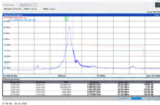
1-N41-PC3-30-20-H-2-DFT-PI2BPSK-Edge_1RB_Right-1@50-Ant1-PASS-see graph
