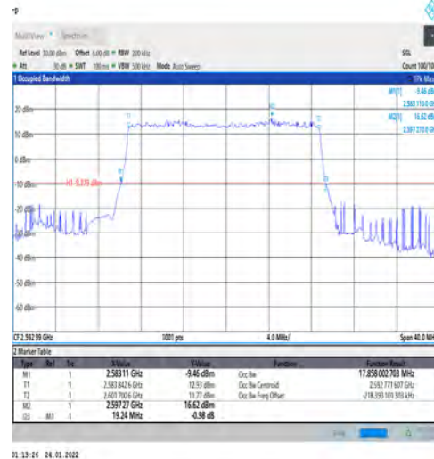
1-N41-PC3-30-20-M-2-DFT-PI2BPSK-Outer_Full-50 @0-Ant1-17.858-19.240-≤20-PASS
