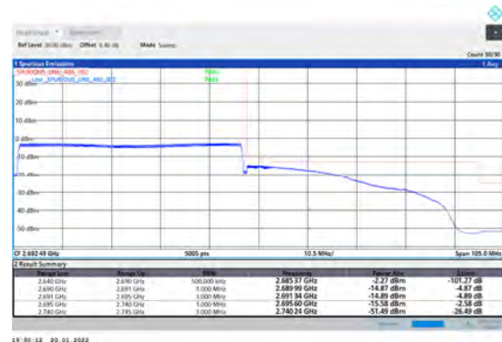
1-N41-PC3-30-50-H-6-CP-QPSK-Outer_Full-133@0 -Ant1-PASS-see graph
