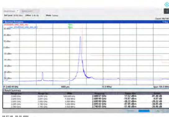
1-N41-PC3-30-50-H-5-CP-QPSK-Edge_1RB_Ri ght-1@132-Ant1-PASS-see graph
