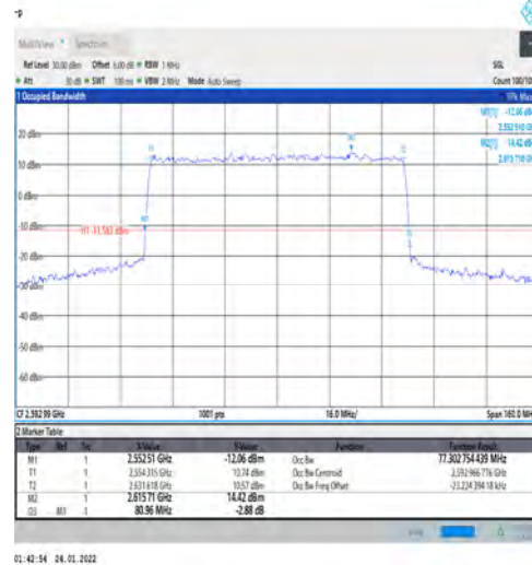
1-N41-PC3-30-80-M-8-CP-64QAM-Outer_Full-217@ 0-Ant1-77.303-80.960-≤80-PASS
