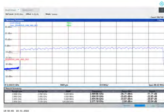
1-N41-PC3-30-80-L-6-CP-QPSK-Outer_Full-217@0-Ant1-PASS-see graph
