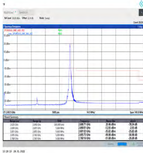
1-N41-PC3-30-70-H-2-DFT-PI2BPSK-Edge_1RB_Ri ght-Edge_1_Right@N/A-Ant1-PASS-see graph
