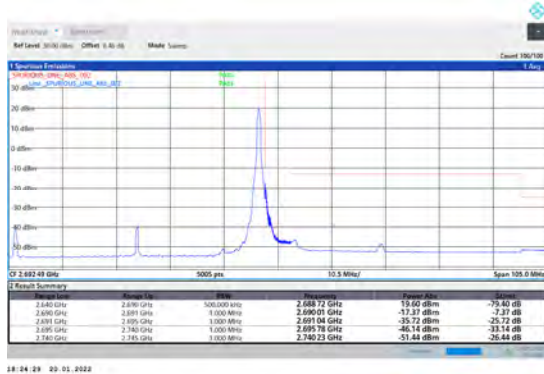
1-N41-PC3-30-50-H-2-DFT-PI2BPSK-Edge_1RB_Ri ght-1@132-Ant1-PASS-see graph
