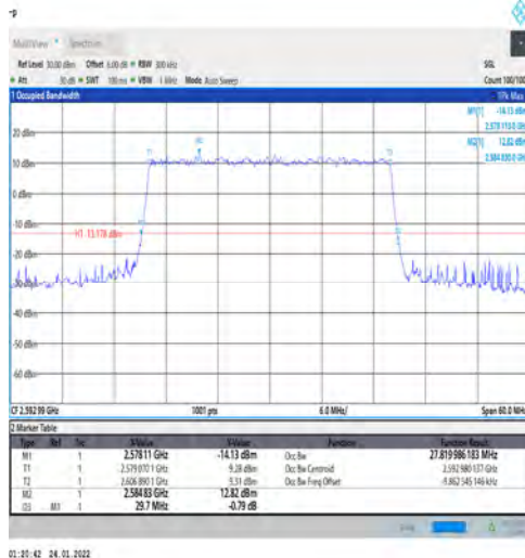
1-N41-PC3-30-30-M-8-CP-64QAM-Outer_Full-78@0 -Ant1-27.82-29.700-≤30-PASS
