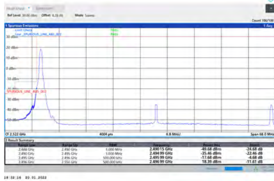
1-N41-PC3-30-60-L-4-CP-QPSK-Edge_1RB_Left-1 @0-Ant1-PASS-see graph
