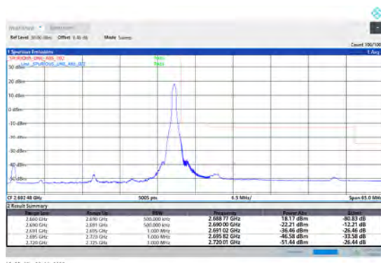
1-N41-PC3-30-30-H-5-CP-QPSK-Edge_1RB_Right-1@77-Ant1-PASS-see graph
