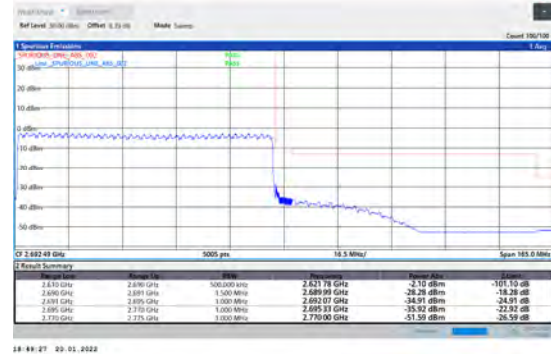
1-N41-PC3-30-80-H-6-CP-QPSK-Outer_Full-217@0 -Ant1-PASS-see graph
