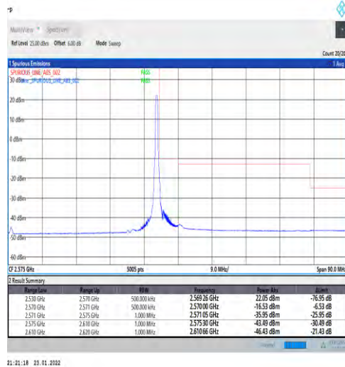
1-N7-PC3-15-40-H-5-CP-QPSK-Edge_1RB_Right-1@215-Ant1-PASS-see graph
