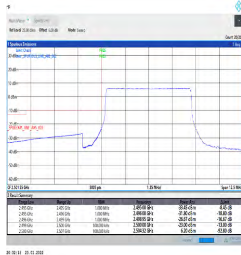
1-N7-PC3-15-5-L-6-CP-QPSK-Outer_Full-25@0-Ant1-PASS-see graph
