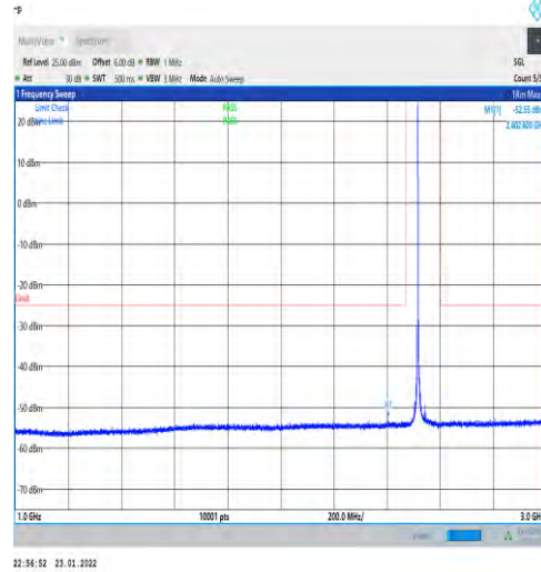
1-N7-PC3-15-40-M-1-DFT-PI2BPSK-Edge_1RB_Left -1@0-1000-3000-Ant1--52.55--25-PASS
