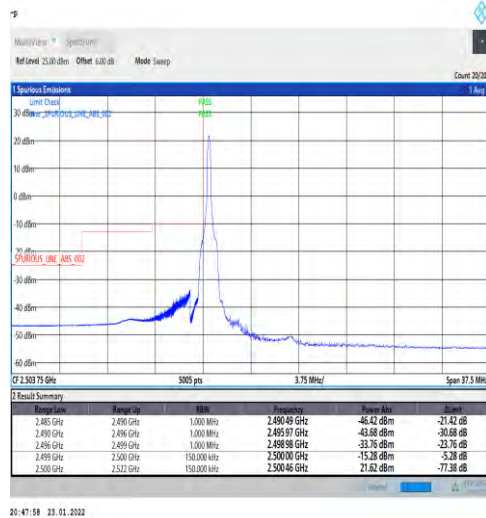
1-N7-PC3-15-15-L-4-CP-QPSK-Edge_1RB_Left-1@0-Ant1-PASS-see graph
