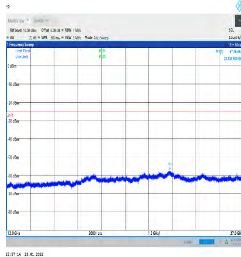
1-N7-PC3-15-40-M-1-DFT-PI2BPSK-Edge_1RB_Left -1@0-12000-27000-Ant1--57.26--25-PASS
