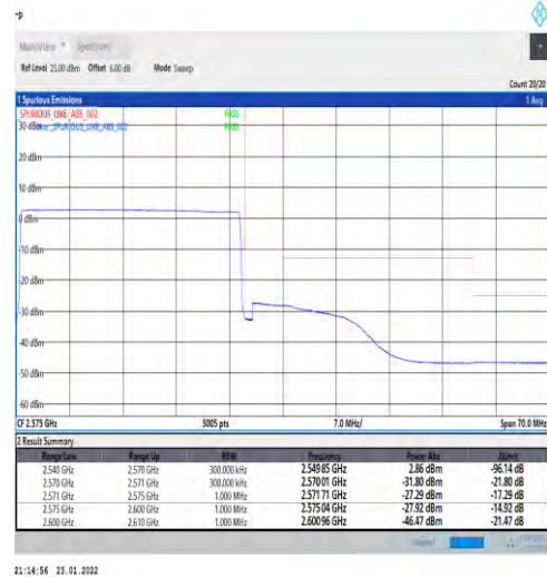
1-N7-PC3-15-30-H-6-CP-QPSK-Outer_Full-160@0-Ant1-PASS-see graph
