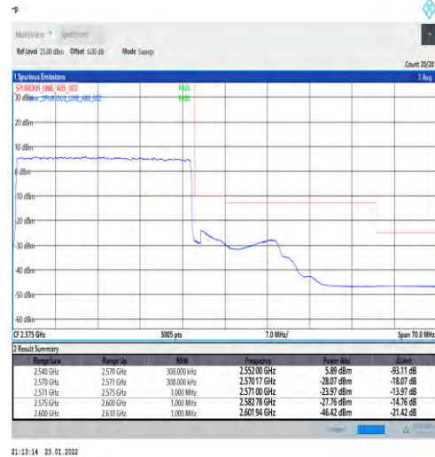
1-N7-PC3-15-30-H-3-DFT-PI2BPSK-Outer_Full-160@0-Ant1-PASS-see graph
