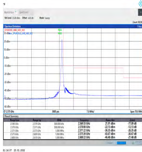
1-N7-PC3-15-30-H-5-CP-QPSK-Edge_1RB_Right-1@159-Ant1-PASS-see graph
