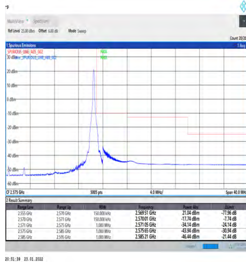
1-N7-PC3-15-15-H-5-CP-QPSK-Edge_1RB_Right-1@78-Ant1-PASS-see graph
