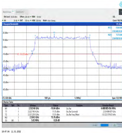
1-N7-PC3-15-5-M-1-DFT-QPSK-Outer_Full-25@0-A nt1-4.489-5.020-≤5-PASS
