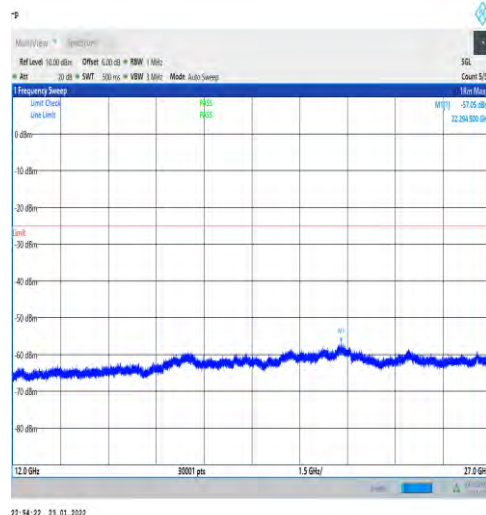
1-N7-PC3-15-40-L-1-DFT-PI2BPSK-Edge_1RB_Left- 1@0-12000-27000-Ant1--57.05--25-PASS
