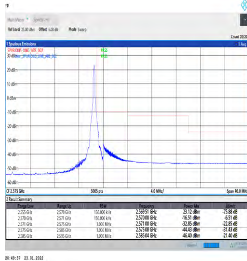
1-N7-PC3-15-15-H-2-DFT-PI2BPSK-Edge_1RB_Right-1@78-Ant1-PASS-see graph
