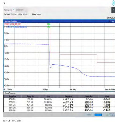
1-N7-PC3-15-25-H-6-CP-QPSK-Outer_Full-133@0-Ant1-PASS-see graph
