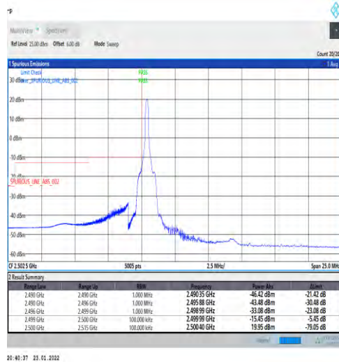
1-N7-PC3-15-10-L-4-CP-QPSK-Edge_1RB_Left-1@0-Ant1-PASS-see graph
