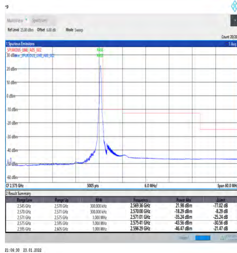
1-N7-PC3-15-25-H-5-CP-QPSK-Edge_1RB_Right-1@132-Ant1-PASS-see graph
