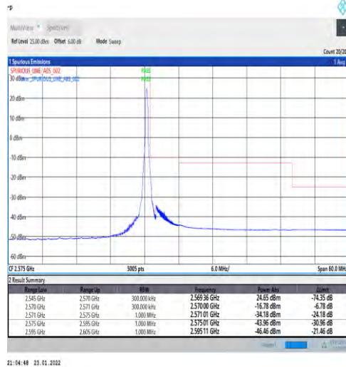
1-N7-PC3-15-25-H-2-DFT-PI2BPSK-Edge_1RB_Right-1@132-Ant1-PASS-see graph
