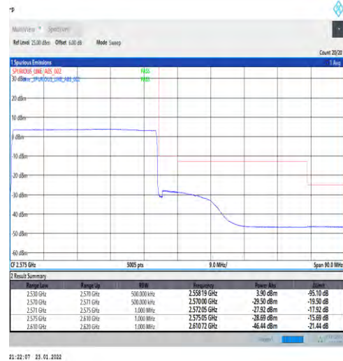
1-N7-PC3-15-40-H-6-CP-QPSK-Outer_Full-216@0-Ant1-PASS-see graph
