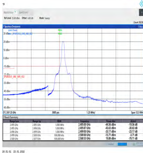
1-N7-PC3-15-5-L-4-CP-QPSK-Edge_1RB_Left-1@0-Ant1-PASS-see graph
