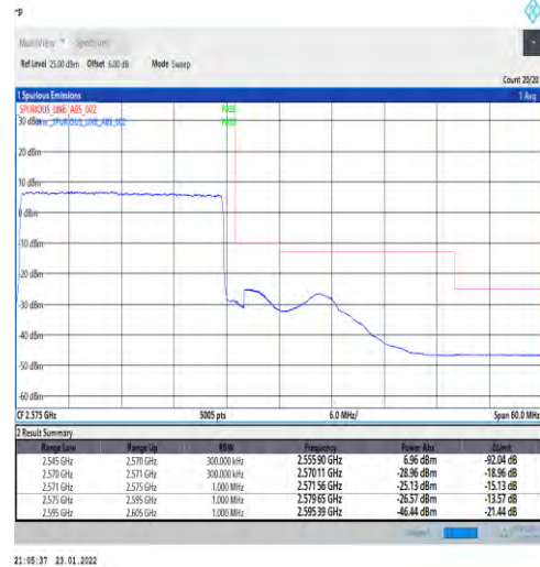
1-N7-PC3-15-25-H-3-DFT-PI2BPSK-Outer_Full-128@0-Ant1-PASS-see graph
