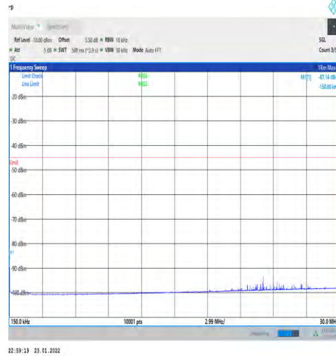
1-N7-PC3-15-40-H-1-DFT-PI2BPSK-Edge_1RB_Left -1@0-0.15-30-Ant1--87.14--45-PASS
