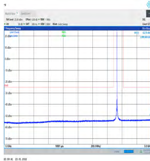
1-N7-PC3-15-40-H-1-DFT-PI2BPSK-Edge_1RB_Left -1@0-1000-3000-Ant1--52.70--25-PASS
