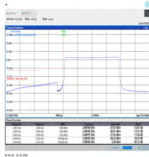
1-N7-PC3-15-10-L-6-CP-QPSK-Outer_Full-52@0-Ant1-PASS-see graph
