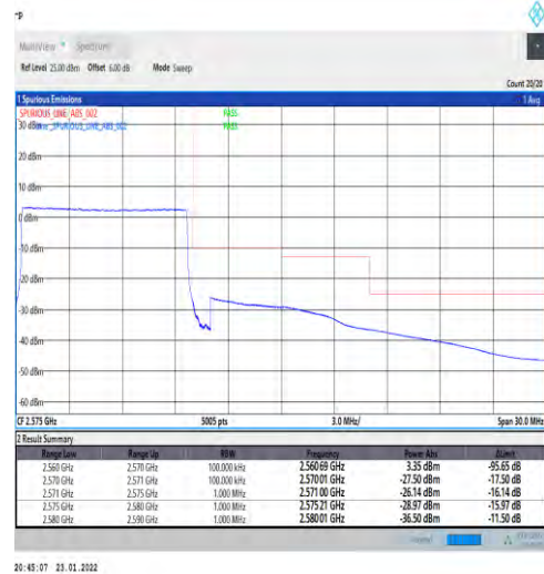
1-N7-PC3-15-10-H-6-CP-QPSK-Outer_Full-52@0-Ant1-PASS-see graph
