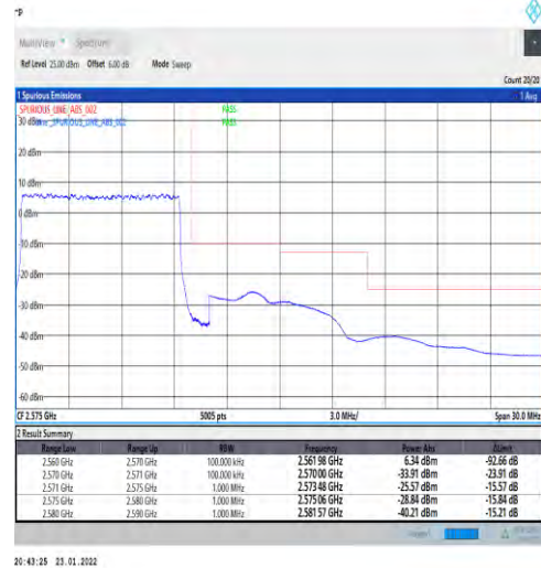
1-N7-PC3-15-10-H-3-DFT-PI2BPSK-Outer_Full-50@0-Ant1-PASS-see graph
