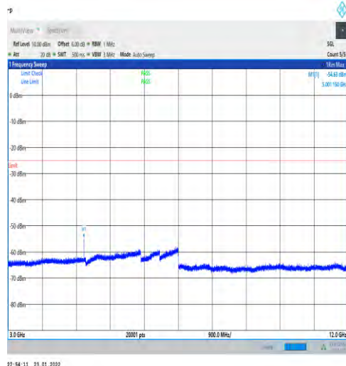
1-N7-PC3-15-40-L-1-DFT-PI2BPSK-Edge_1RB_Left -1@0-3000-12000-Ant1--54.63--25-PASS
