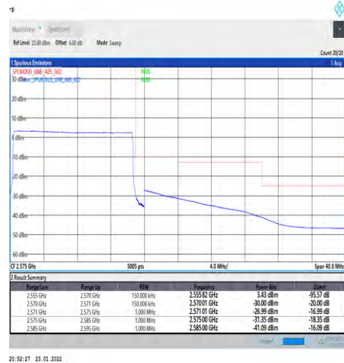
1-N7-PC3-15-15-H-6-CP-QPSK-Outer_Full-79@0-Ant1-PASS-see graph
