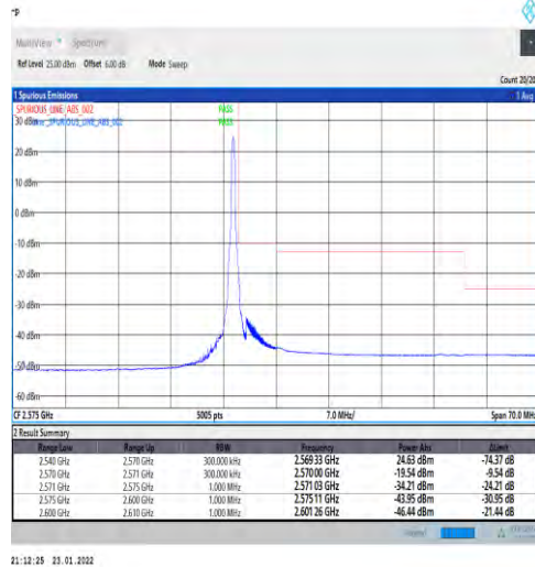
1-N7-PC3-15-30-H-2-DFT-PI2BPSK-Edge_1RB_Right-1@159-Ant1-PASS-see graph
