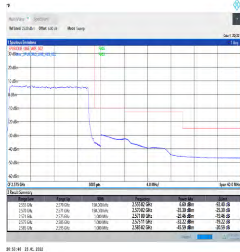
1-N7-PC3-15-15-H-3-DFT-PI2BPSK-Outer_Full-75@0-Ant1-PASS-see graph
