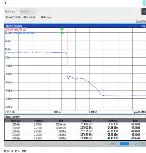
1-N7-PC3-15-40-H-3-DFT-PI2BPSK-Outer_Full-216@0-Ant1-PASS-see graph
