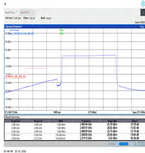
1-N7-PC3-15-15-L-6-CP-QPSK-Outer_Full-79@0-Ant1-PASS-see graph
