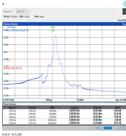
1-N7-PC3-15-5-L-1-DFT-PI2BPSK-Edge_1RB_Left-1@0-Ant1-PASS-see graph
