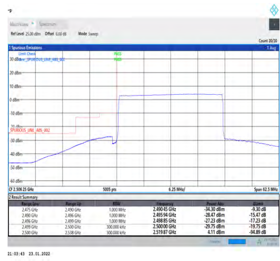
1-N7-PC3-15-25-L-6-CP-QPSK-Outer_Full-133@0-Ant1-PASS-see graph
