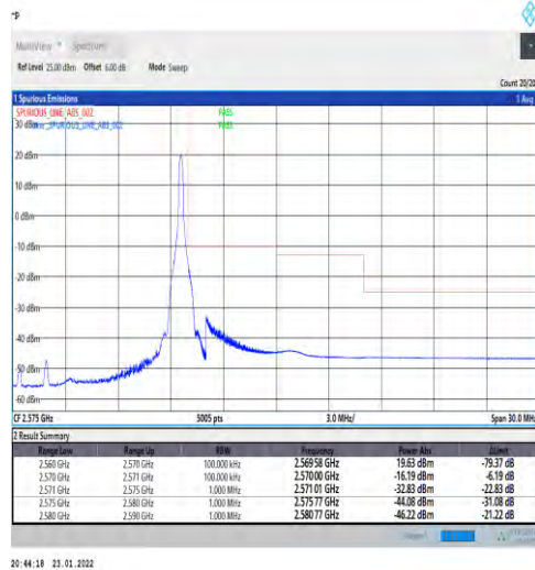
1-N7-PC3-15-10-H-5-CP-QPSK-Edge_1RB_Right-1@51-Ant1-PASS-see graph
