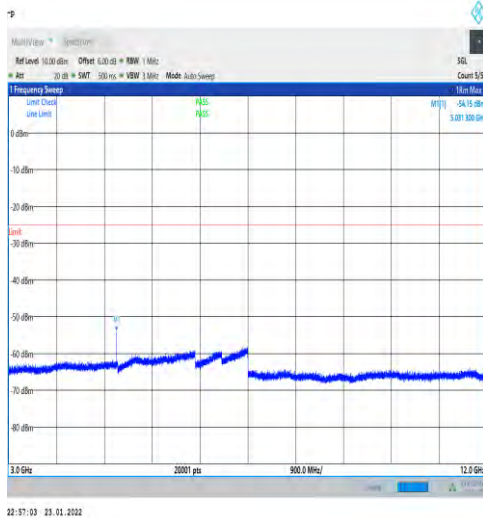
1-N7-PC3-15-40-M-1-DFT-PI2BPSK-Edge_1RB_Lef t-1@0-3000-12000-Ant1--54.15--25-PASS
