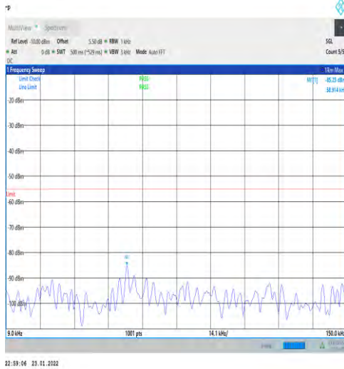
1-N7-PC3-15-40-H-1-DFT-PI2BPSK-Edge_1RB_Left -1@0-0.009-0.15-Ant1--85.23--55-PASS
