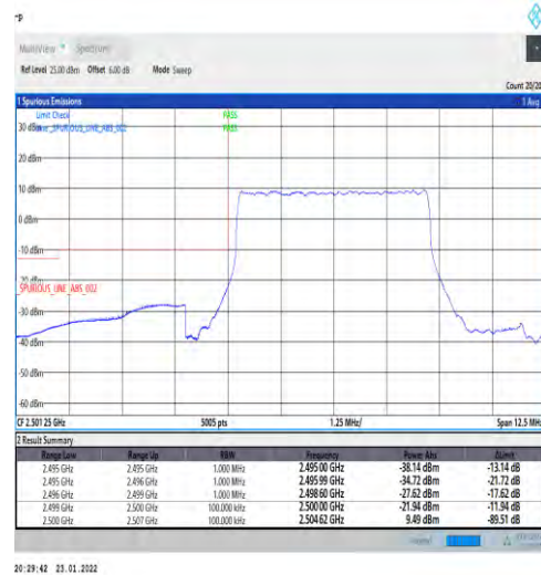
1-N7-PC3-15-5-L-3-DFT-PI2BPSK-Outer_Full-25@0-Ant1-PASS-see graph
