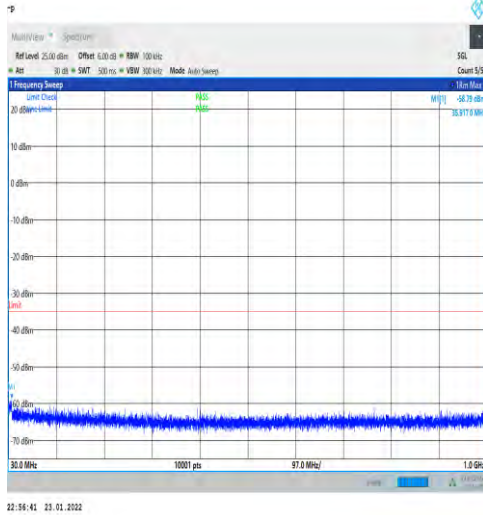
1-N7-PC3-15-40-M-1-DFT-PI2BPSK-Edge_1RB_Lef t-1@0-30-1000-Ant1--58.79--35-PASS
