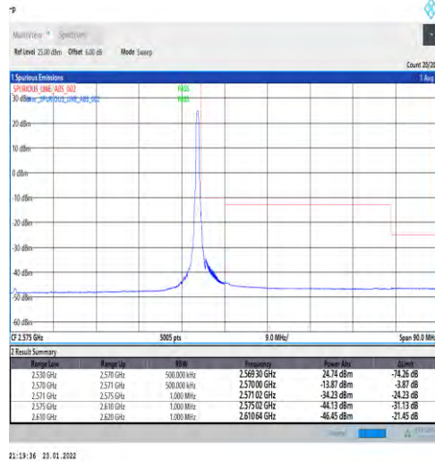
1-N7-PC3-15-40-H-2-DFT-PI2BPSK-Edge_1RB_Right-1@215-Ant1-PASS-see graph
