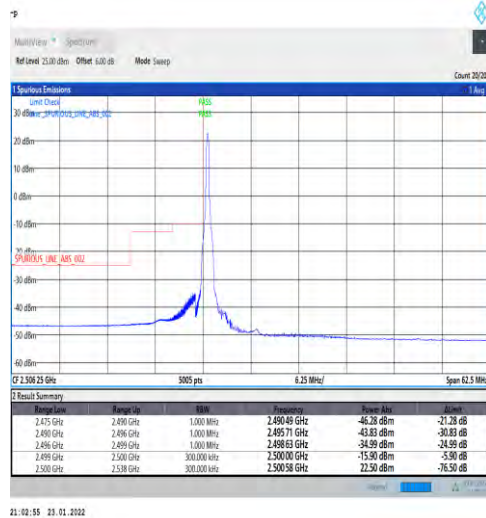
1-N7-PC3-15-25-L-4-CP-QPSK-Edge_1RB_Left-1@0-Ant1-PASS-see graph
