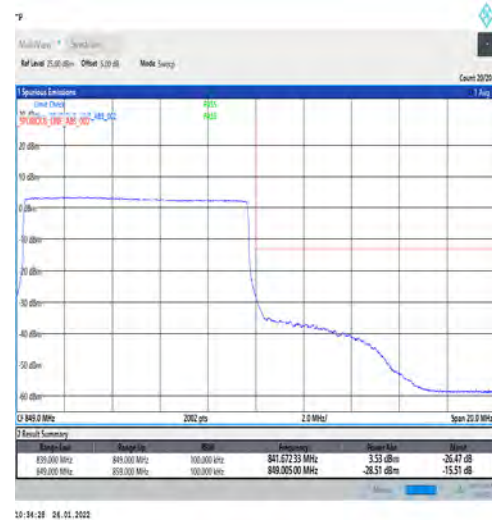
1-N5-PC3-15-10-H-6-CP-QPSK-Outer_Full-52@0-Ant1-seegraph-PASS-see graph
