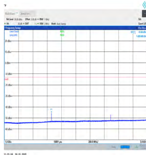
1-N5-PC3-15-20-H-1-DFT-PI2BPSK-Edge_1RB_Left -1@0-1000-3000-Ant1--45.60--13-PASS
