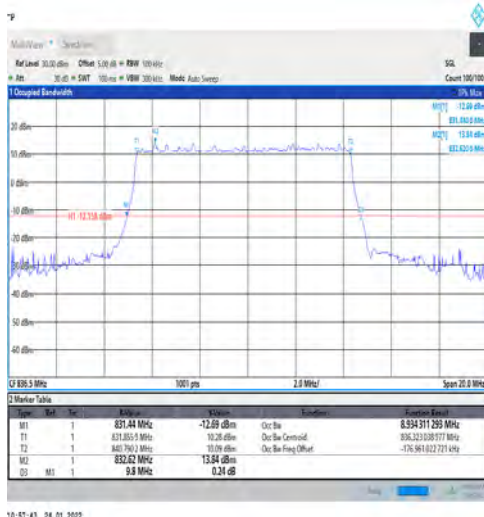
1-N5-PC3-15-10-M-4-DFT-64QAM-Outer_Full-50@0-Ant1-8.934-9.800≤10-PASS
