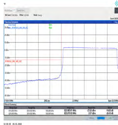
1-N5-PC3-15-10-L-6-CP-QPSK-Outer_Full-52@0-Ant1-seegraph-PASS-see graph
