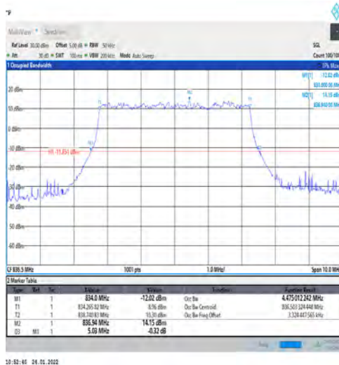
1-N5-PC3-15-5-M-3-DFT-16QAM-Outer_Full-25@0- Ant1-4.475-5.030≤5-PASS
