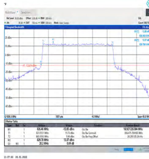
1-N5-PC3-15-20-M-7-CP-16QAM-Outer_Full-106@0-Ant1-18.927-20.200-≤20-PASS
