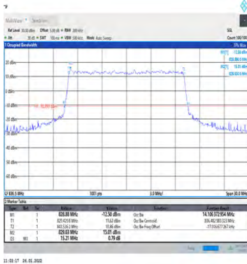
1-N5-PC3-15-15-M-7-CP-16QAM-Outer_Full-79@0- Ant1-14.106-15.210-≤15-PASS
