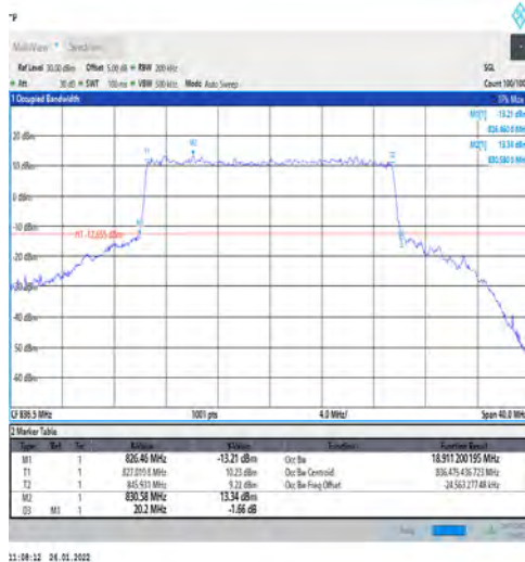
1-N5-PC3-15-20-M-8-CP-64QAM-Outer_Full-106@0-Ant1-18.911-20.200-≤20-PASS
