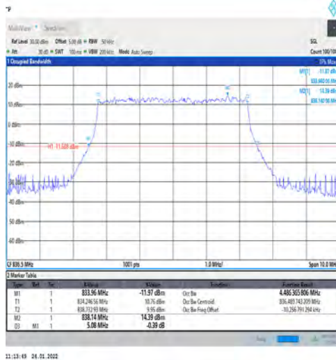
1-N5-PC3-15-5-M-1-DFT-QPSK-Outer_Full-25@0-A nt1-4.486-5.080≤5-PASS
