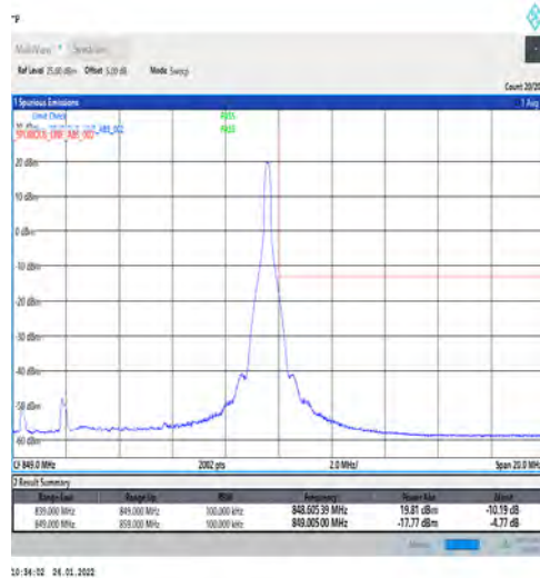
1-N5-PC3-15-10-H-5-CP-QPSK-Edge_1RB_Right-1@51-Ant1-seegraph-PASS-see graph
