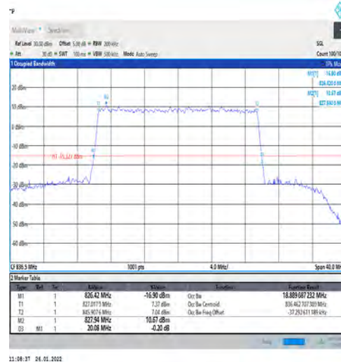
1-N5-PC3-15-20-M-9-CP-256QAM-Outer_Full-106@0-Ant1-18.89-20.080-≤20-PASS
