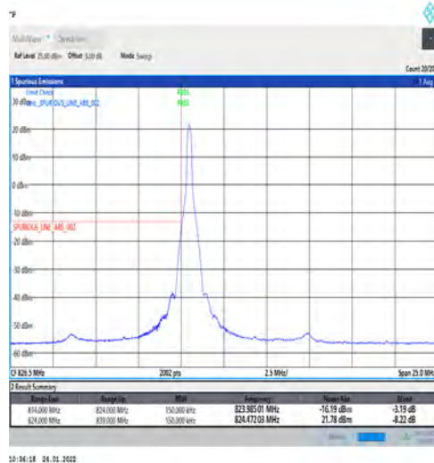
1-N5-PC3-15-15-L-4-CP-QPSK-Edge_1RB_Left-1@0-Ant1-seegraph-PASS-see graph
