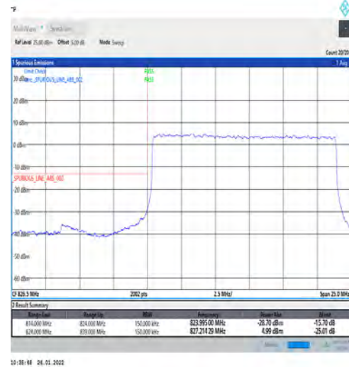
1-N5-PC3-15-15-L-3-DFT-PI2BPSK-Outer_Full-75 @0-Ant1-seegraph-PASS-see graph
