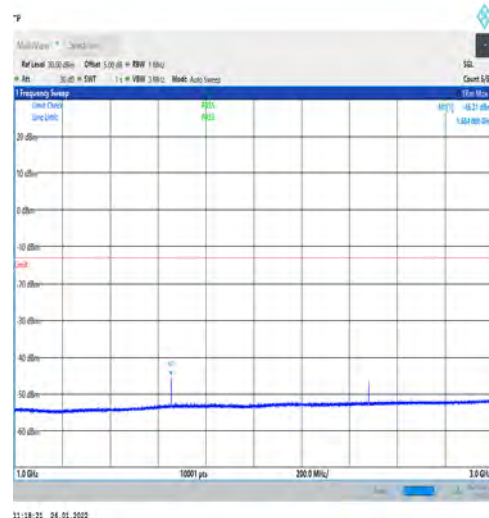
1-N5-PC3-15-20-M-1-DFT-PI2BPSK-Edge_1RB_Left -1@0-1000-3000-Ant1--45.21--13-PASS
