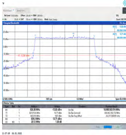
1-N5-PC3-15-20-M-6-CP-QPSK-Outer_Full-106@0-Ant1-18.9-20.120-≤20-PASS
