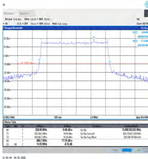
1-N5-PC3-15-15-M-1-DFT-QPSK-Outer_Full-75@0- Ant1-13.498-14.430-≤15-PASS
