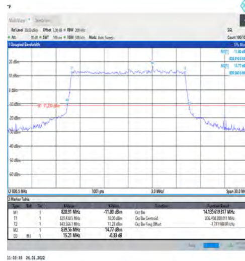
1-N5-PC3-15-15-M-8-CP-64QAM-Outer_Full-79@0- Ant1-14.136-15.210-≤15-PASS
