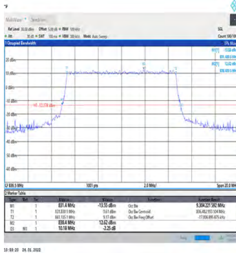
1-N5-PC3-15-10-M-8-CP-64QAM-Outer_Full-52@0 -Ant1-9.304-10.180-≤10-PASS
