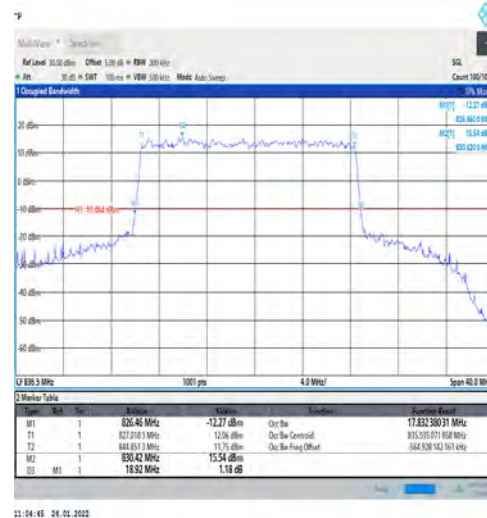
1-N5-PC3-15-20-M-1-DFT-QPSK-Outer_Full-100@0- Ant1-17.832-18.920-≤20-PASS
