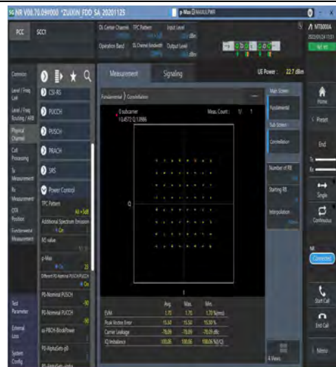
1-N5-PC3-15-20-M-4-DFT-64QAM-Outer_Full-100 @0-Ant1-see graph-PASS
