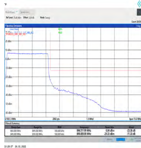
1-N5-PC3-15-5-H-6-CP-QPSK-Outer_Full-25@0-Ant1-seegraph-PASS-see graph
