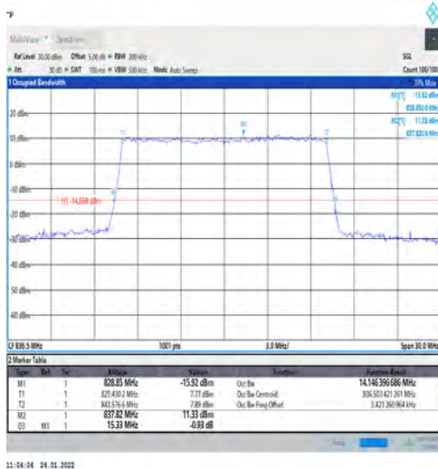
1-N5-PC3-15-15-M-9-CP-256QAM-Outer_Full-79@0- Ant1-14.146-15.330-≤15-PASS
