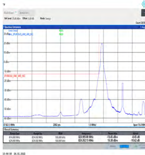
1-N5-PC3-15-5-L-4-CP-QPSK-Edge_1RB_Left-1@0-A nt1-seegraph-PASS-see graph
