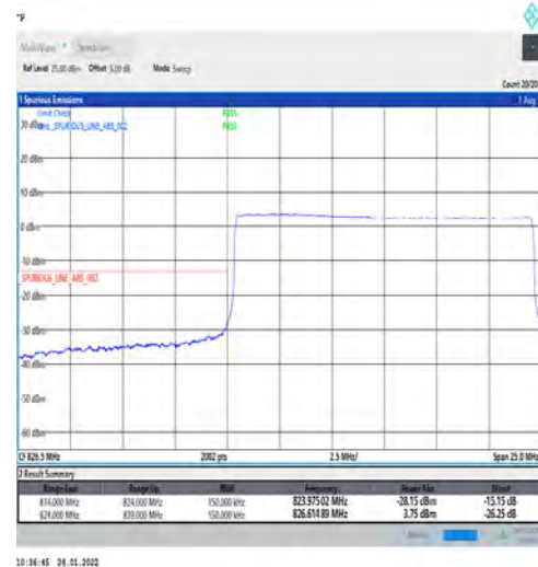
1-N5-PC3-15-15-L-6-CP-QPSK-Outer_Full-79@0-Ant1-seegraph-PASS-see graph
