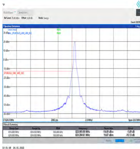
1-N5-PC3-15-10-L-4-CP-QPSK-Edge_1RB_Left-1@0-Ant1-seegraph-PASS-see graph
