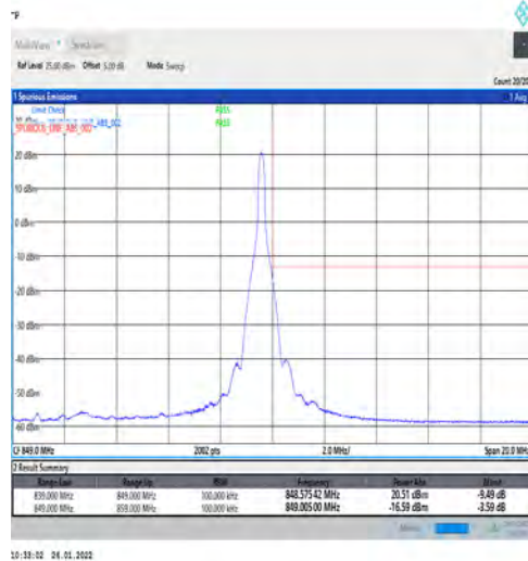
1-N5-PC3-15-10-H-2-DFT-PI2BPSK-Edge_1RB_Right-1@51-Ant1-seegraph-PASS-see graph
