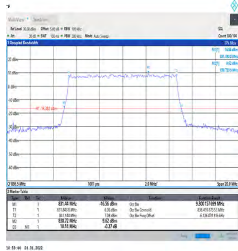
1-N5-PC3-15-10-M-9-CP-256QAM-Outer_Full-52@0- Ant1-9.3-10.140-≤10-PASS
