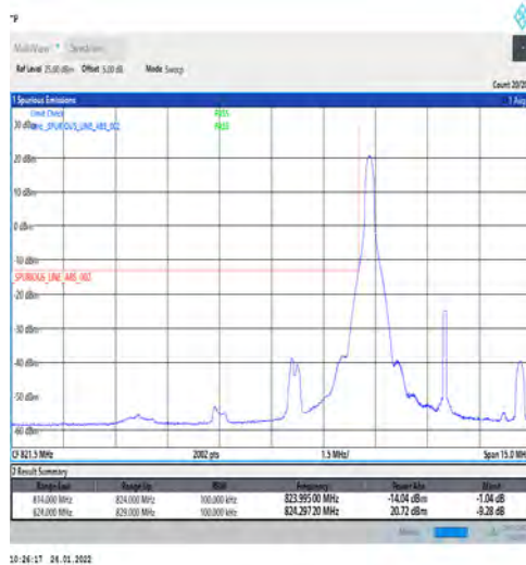
1-N5-PC3-15-5-L-1-DFT-PI2BPSK-Edge_1RB_Left-1 @0-Ant1-seegraph-PASS-see graph
