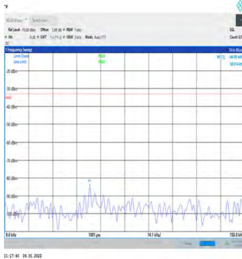
1-N5-PC3-15-20-M-1-DFT-PI2BPSK-Edge_1RB_Left -1@0-0.009-0.15-Ant1--84.95--33-PASS
