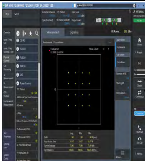
1-N5-PC3-15-20-M-3-DFT-16QAM-Outer_Full-100@ 0-Ant1-see graph-PASS
