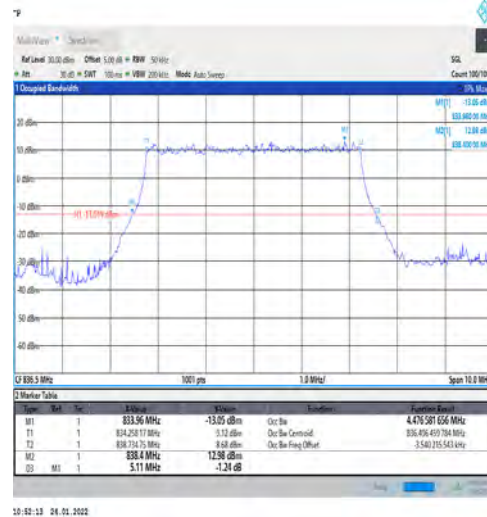
1-N5-PC3-15-5-M-2-DFT-PI2BPSK-Outer_Full-25@0 -Ant1-4.477-5.110≤5-PASS
