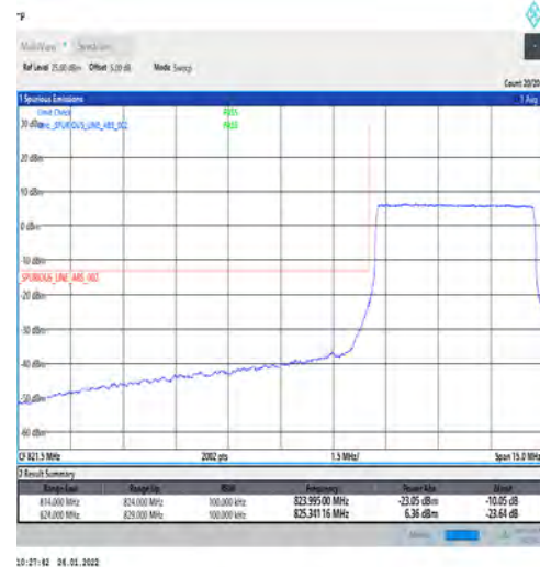
1-N5-PC3-15-5-L-6-CP-QPSK-Outer_Full-25@0-A nt1-seegraph-PASS-see graph
