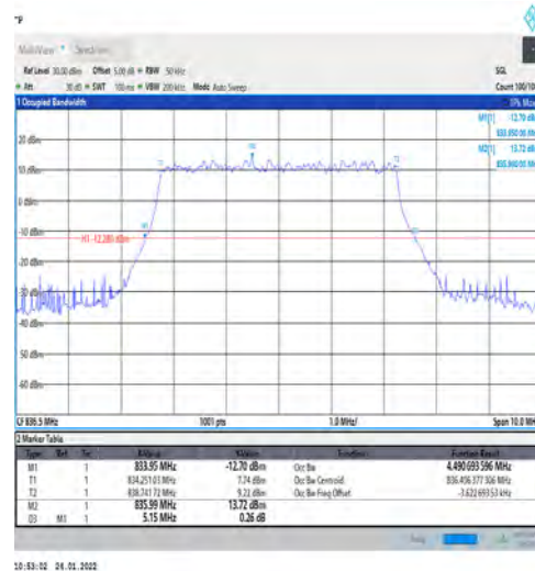
1-N5-PC3-15-5-M-4-DFT-64QAM-Outer_Full-25@0- Ant1-4.491-5.150≤5-PASS
