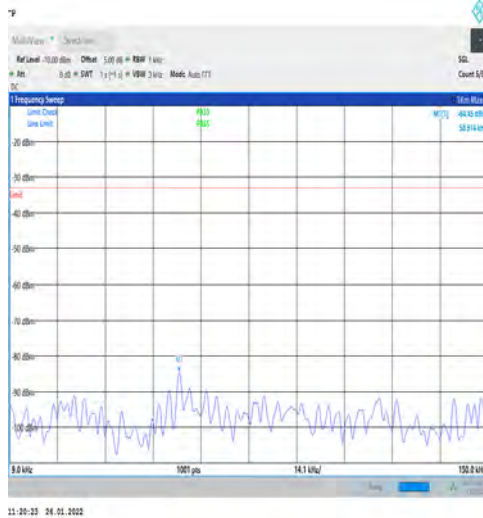
1-N5-PC3-15-20-H-1-DFT-PI2BPSK-Edge_1RB_Left -1@0-0.009-0.15-Ant1--84.45--33-PASS
