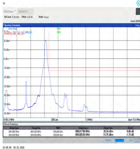
1-N5-PC3-15-5-H-2-DFT-PI2BPSK-Edge_1RB_Right-1 @24-Ant1-seegraph-PASS-see graph
