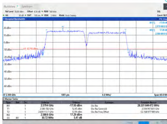
CA_38C-15MHz-15MHz-QPSK-QPSK-37925-38075-75RB#0-75RB#0
