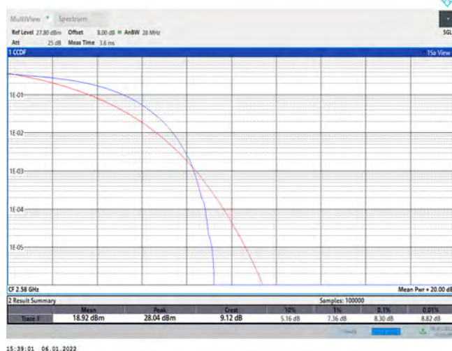
Band38-20MHz-QPSK-38000-100RB#0
