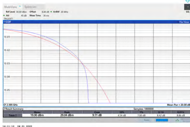
Band38-20MHz-QPSK-38000-100RB#0
