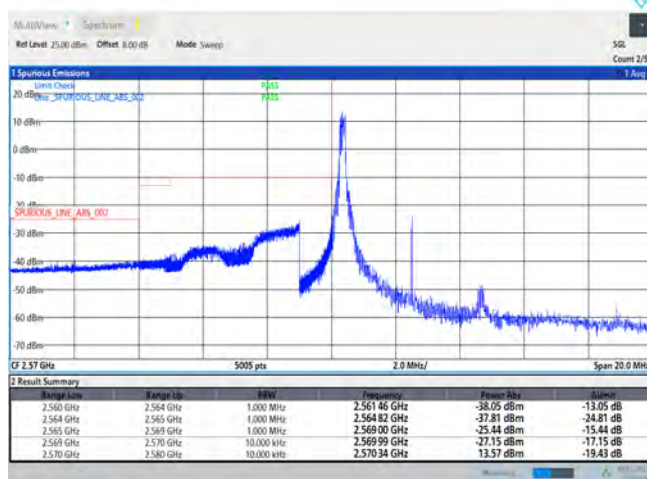
Band38-5MHz-QPSK-37775-25RB#0
