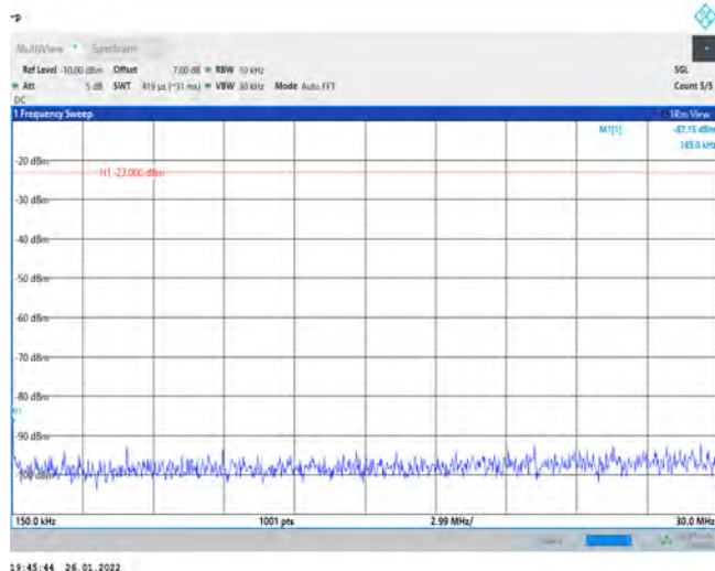
Band26-15MHz-QPSK-26965-1RB#0-Range3:30~1000MHz
