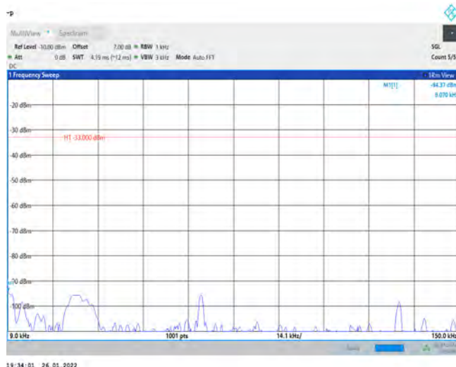
Band26-15MHz-QPSK-26915-1RB#0-Range1:0.009~0.15MHz
