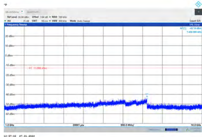
Band26-15MHz-16QAM-26965-1RB#0-Range2:1000~10000MHz
