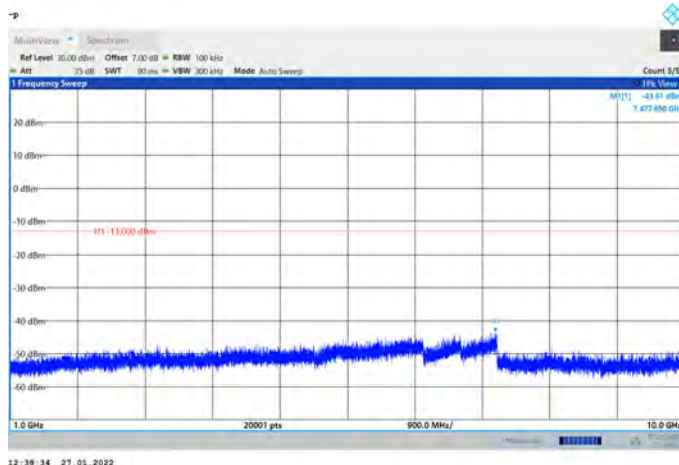
Band26-15MHz-256QAM-26965-1RB#0-Range2:1000~10000MHz
