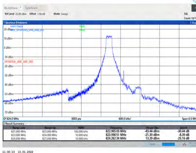
Band26-1.4MHz-QPSK-26797-6RB#0
