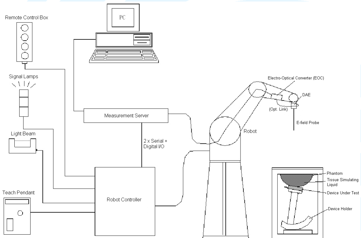
Fig-3.1 DASY Measurement System
