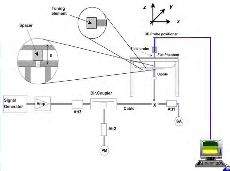
Fig-3.7 System Verification Setup
