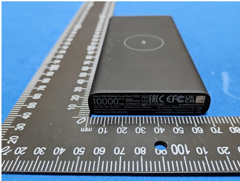
EUT2 Photo
