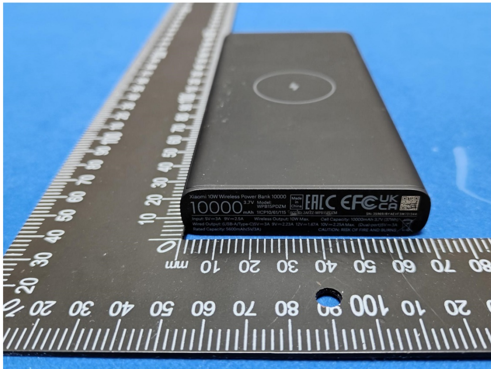
EUT1 Photo
