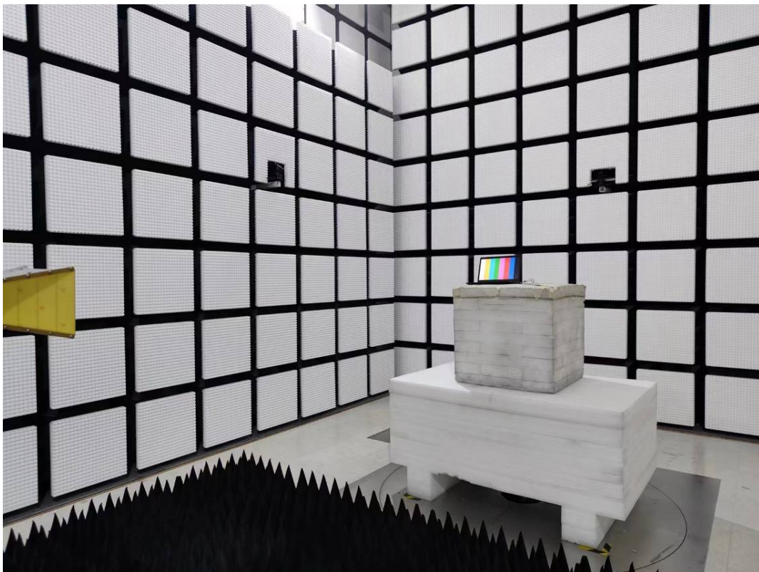
Radiated Emission Above 1GHz View (AVIBG21AUFL_6211ANT)
