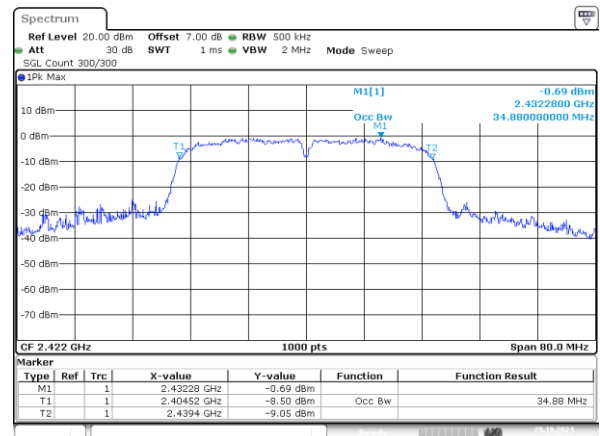
802.11n40_2422MHz 34.880MHz
