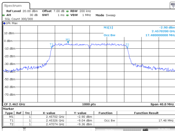
802.11n20_2462MHz 17.480MHz
