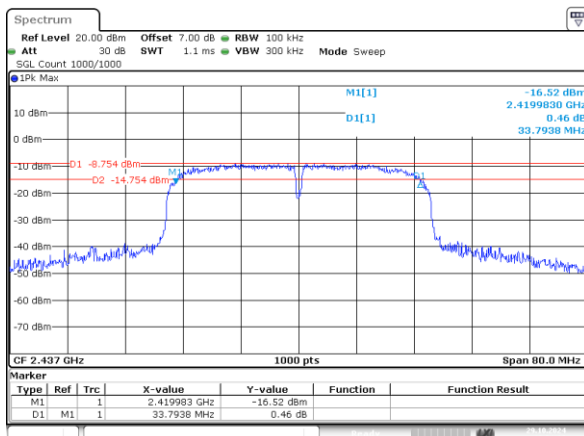
802.11n40_2437MHz 33.794MHz
