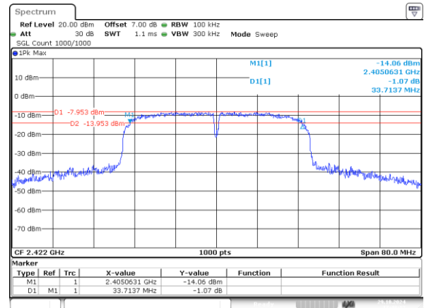
802.11n40_2422MHz 33.714MHz
