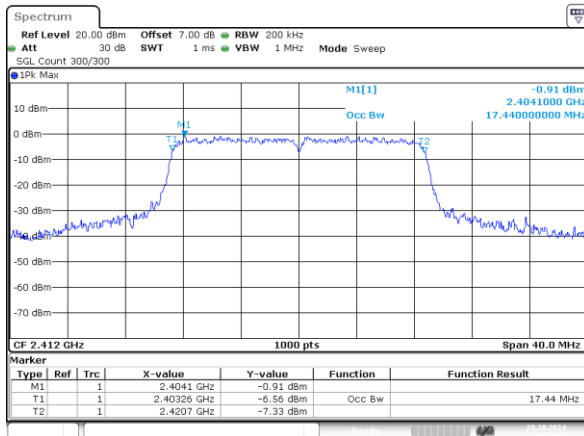
802.11n20_2412MHz 17.440MHz
