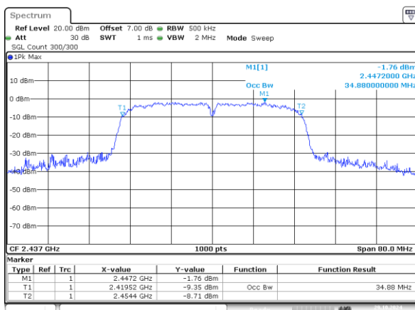
802.11n40_2437MHz 34.880MHz
