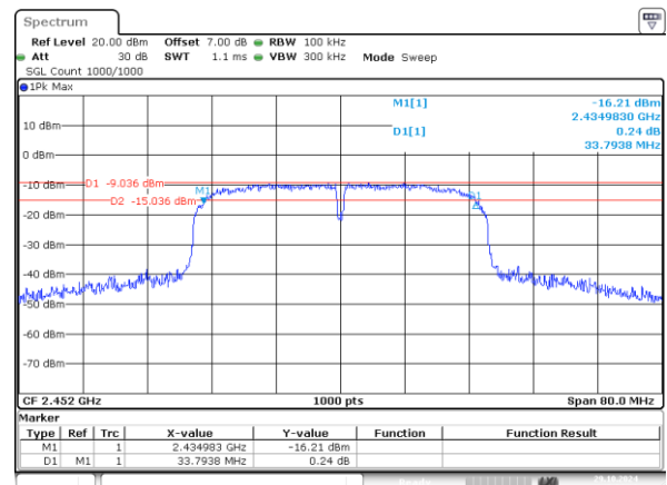
802.11n40_2452MHz 33.794MHz
