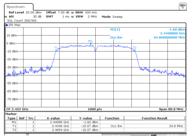
802.11n40_2452MHz 34.800MHz
