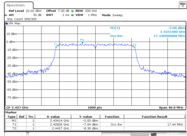
802.11n20_2437MHz 17.440MHz
