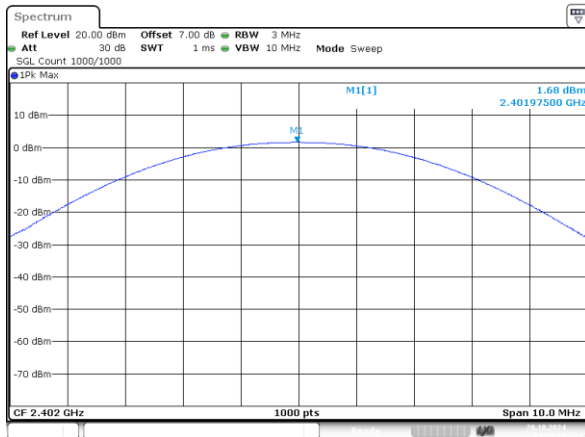
DH5_Low 1.68dBm
