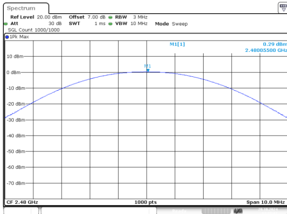
DH5_High 0.29dBm
