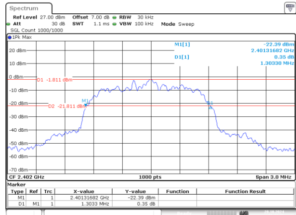
2DH5_Low 1.303MHz
