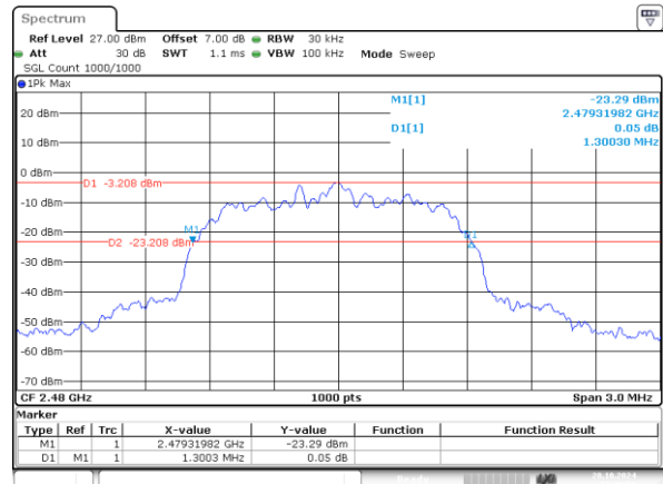
2DH5_High 1.300MHz
