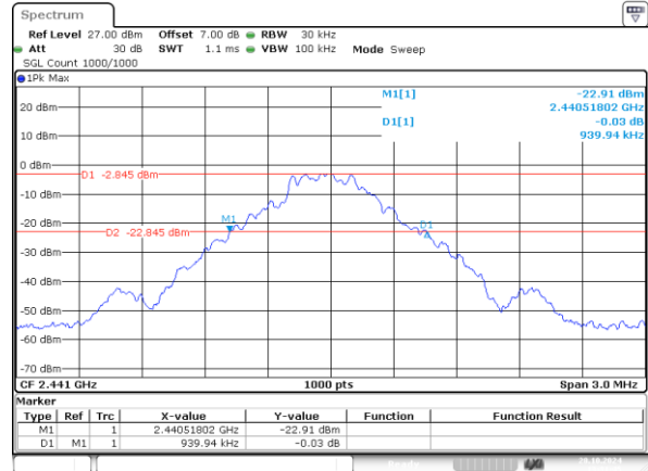
DH5_Middle 0.940MHz
