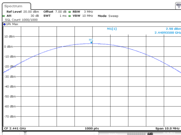
2DH5_Middle 2.98dBm
