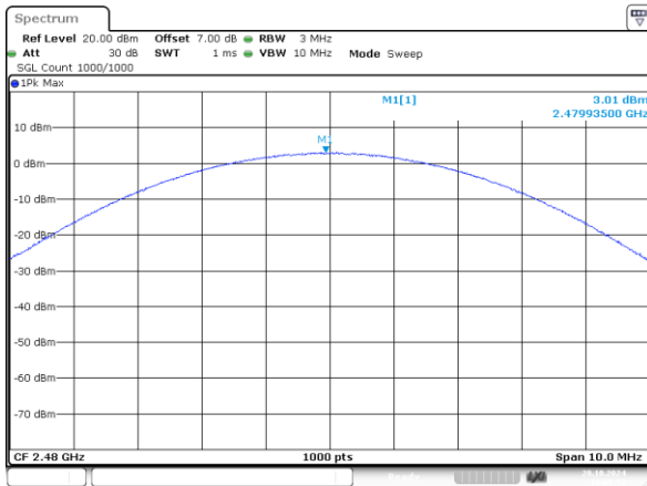
3DH5_High 3.01dBm
