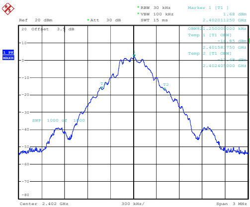
DH1_Low
