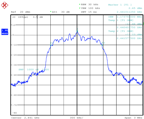
2DH1_Middle
