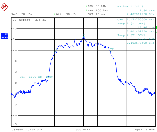
2DH1_Low
