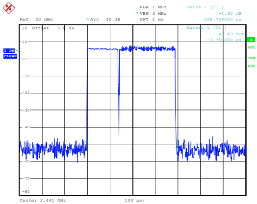
2DH1_Hopping
