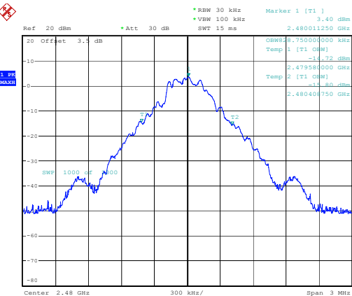
DH1_High
