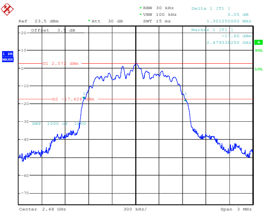
2DH1_High
