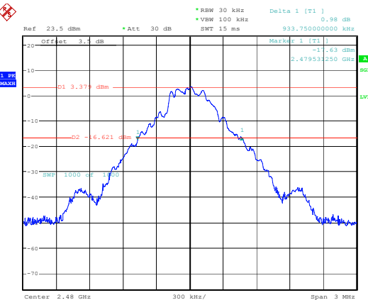
DH1_High
