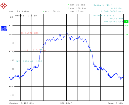
2DH1_Low
