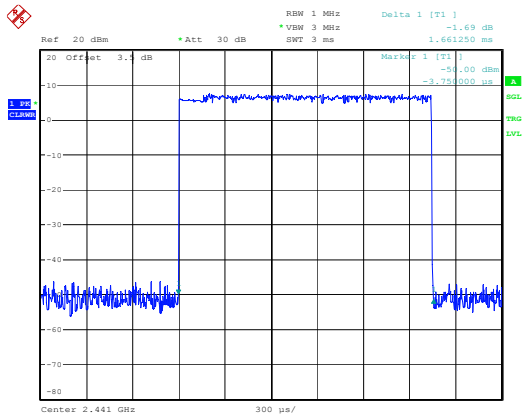
2DH3_Hopping
