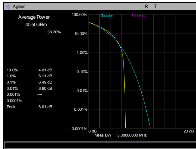
Plot 102. Peak to Average Ratio, Channel 14, Part 24
