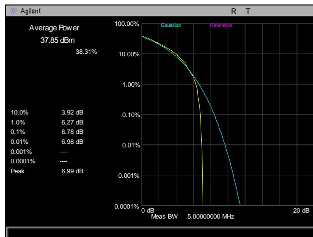
Plot 103. Peak to Average Ratio, Channel 425, Part 24
