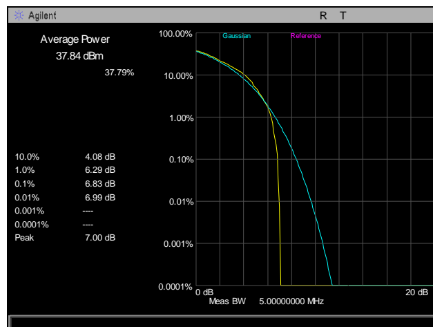
Plot 104. Peak to Average Ratio, Channel 1186, Part 24
