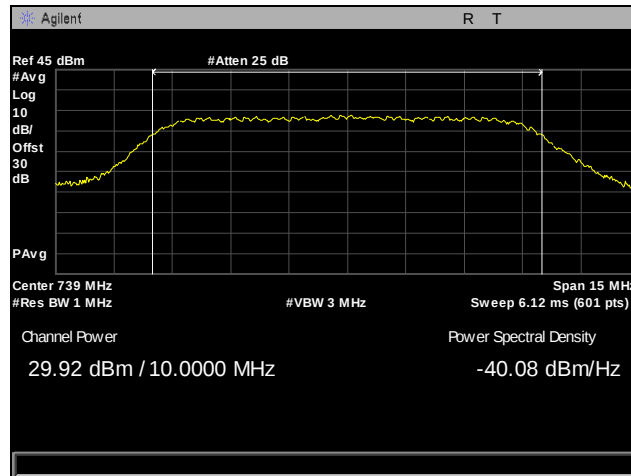
Plot 19. EIRP, Channel 5780, Conducted Power, Part 27, 10 MHz, LTE700
