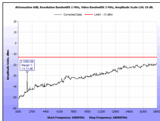
Plot 80. Radiated Spurious Emissions, Low Channel, 1 GHz – 18 GHz, Part 27, 5 MHz, LTE2100
