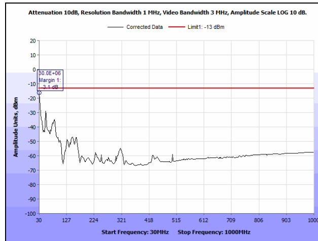
Plot 61. Radiated Spurious Emissions, Low Channel, 30 MHz – 1 GHz, Part 24, 5 MHz
