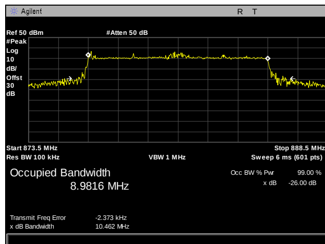
Plot 29. Occupied Bandwidth, Channel 2520, Part 22, 10 MHz
