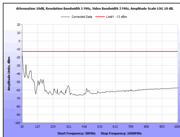
Plot 69. Radiated Spurious Emissions, Mid Channel, 30 MHz – 1 GHz, Part 24, 10 MHz
