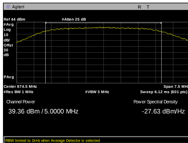
Plot 2. ERP, Channel 2455, Conducted Power, Part 22, 5 MHz
