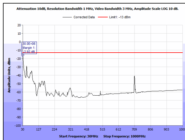
Plot 63. Radiated Spurious Emissions, Mid Channel, 30 MHz – 1 GHz, Part 24, 5 MHz
