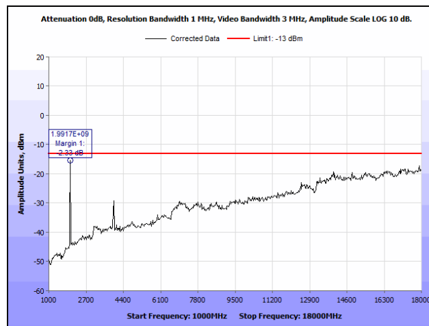
Plot 72. Radiated Spurious Emissions, High Channel, 1 GHz – 18 GHz, Part 24, 10 MHz
