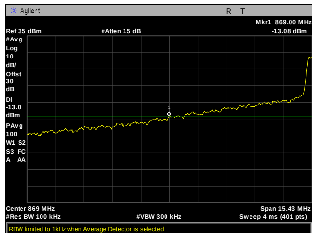
Plot 246. Conducted Band Edge, Channel 2520 (Full Power), 10 MHz, Part 22
