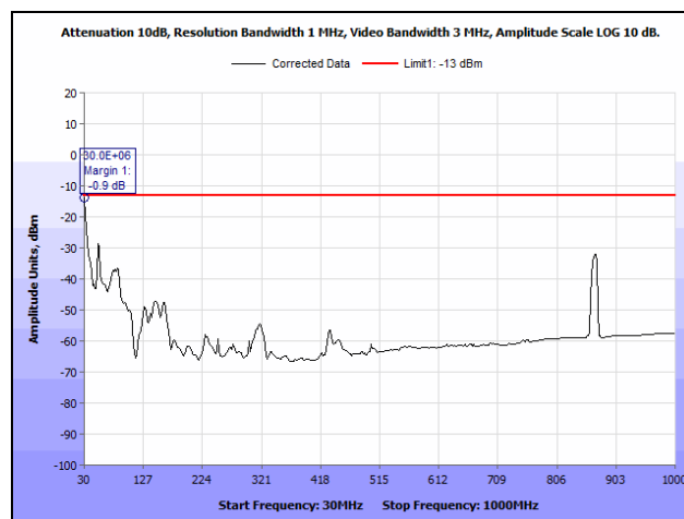
Plot 57. Radiated Spurious Emissions, Mid Channel, 30 MHz – 1 GHz, Part 22, 10 MHz
