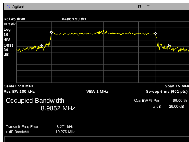
Plot 44. Occupied Bandwidth, Channel 5790, Part 27, 10 MHz, LTE700
