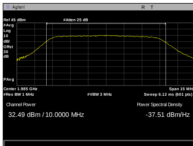
Plot 12. EIRP, Channel 1150, Conducted Power, Part 24, 10 MHz
