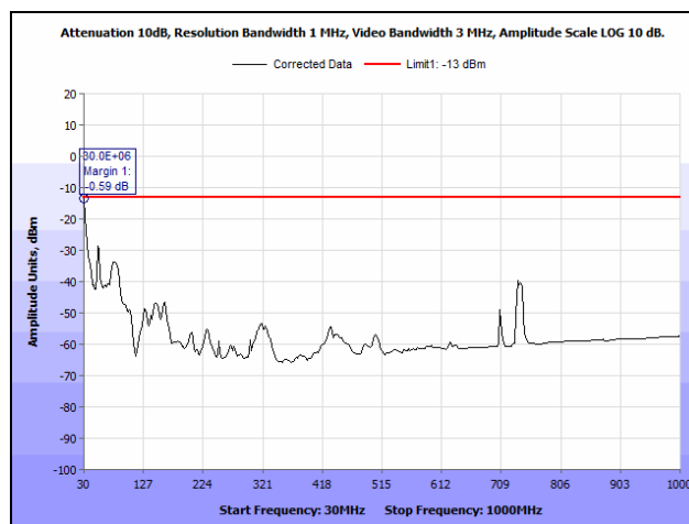
Plot 87. Radiated Spurious Emissions, Mid Channel, 30 MHz – 1 GHz, Part 27, 10 MHz, LTE700
