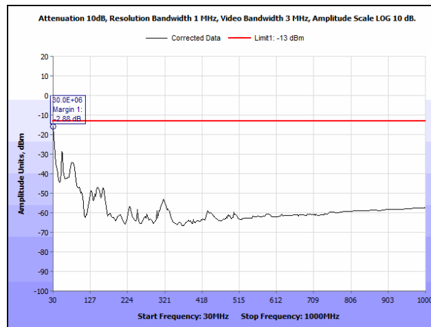
Plot 71. Radiated Spurious Emissions, High Channel, 30 MHz – 1 GHz, Part 24, 10 MHz
