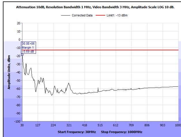
Plot 79. Radiated Spurious Emissions, Low Channel, 30 MHz – 1 GHz, Part 27, 5 MHz, LTE2100
