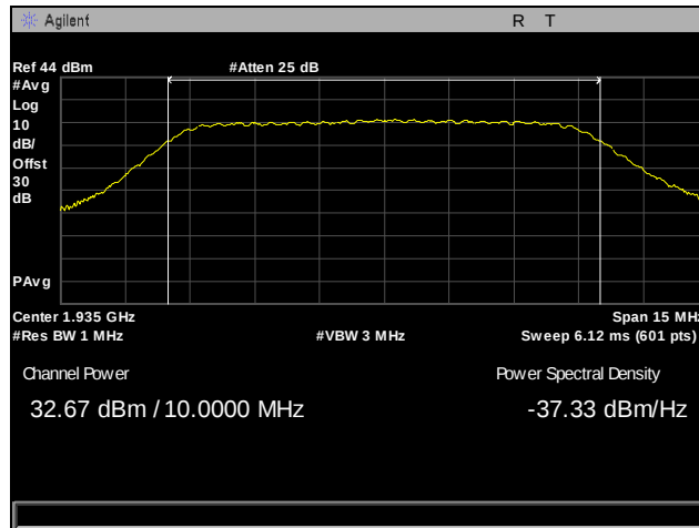
Plot 10. EIRP, Channel 650, Conducted Power, Part 24, 10 MHz
