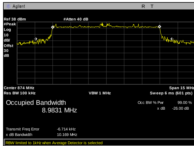
Plot 28. Occupied Bandwidth, Channel 2450, Part 22, 10 MHz
