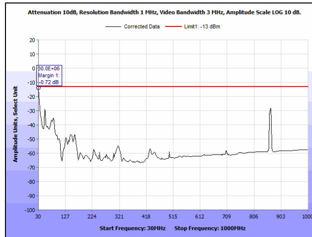
Plot 49. Radiated Spurious Emissions, Low Channel, 30 MHz – 1 GHz, Part 22, 5 MHz
