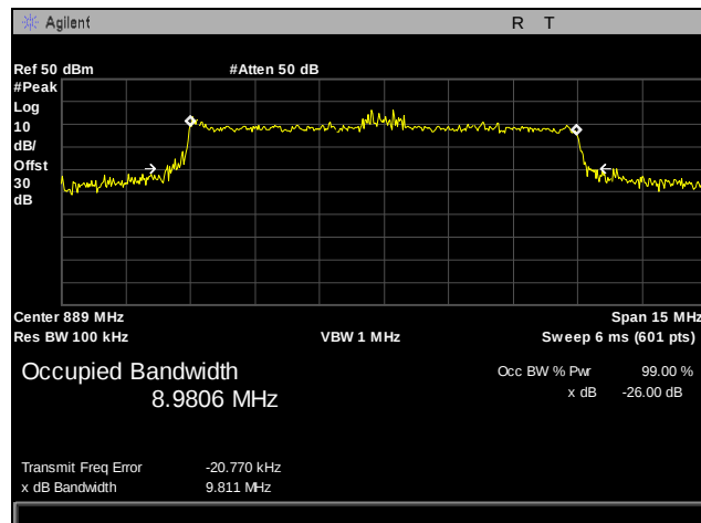
Plot 30. Occupied Bandwidth, Channel 2600, Part 22, 10 MHz
