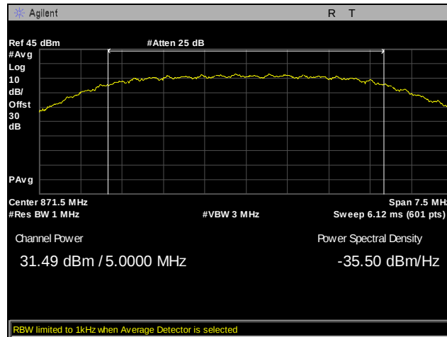
Plot 1. ERP, Channel 2425, Conducted Power, Part 22, 5 MHz
