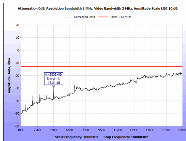
Plot 86. Radiated Spurious Emissions, Low Channel, 1 GHz – 18 GHz, Part 27, 10 MHz, LTE700
