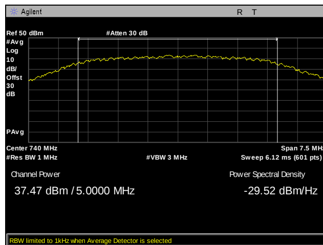
Plot 14. EIRP, Channel 5790, Conducted Power, Part 27, 5 MHz, LTE700
