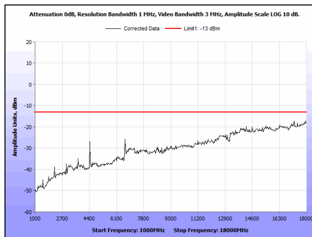
Plot 78. Radiated Spurious Emissions, High Channel, 1 GHz – 18 GHz, Part 27, 5 MHz, LTE700
