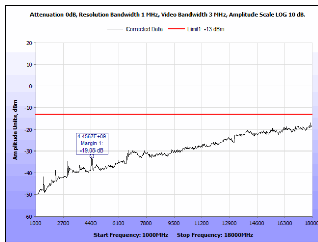
Plot 90. Radiated Spurious Emissions, High Channel, 1 GHz – 18 GHz, Part 27, 10 MHz, LTE700
