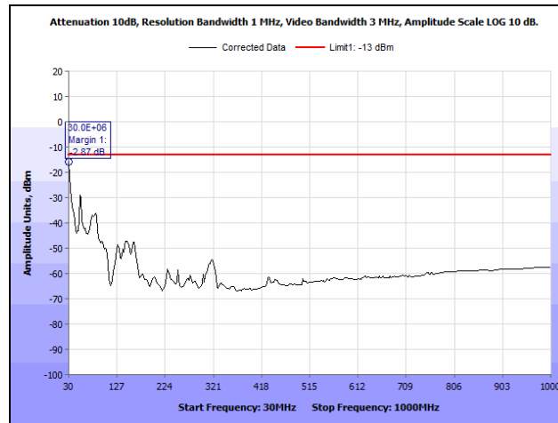
Plot 67. Radiated Spurious Emissions, Low Channel, 30 MHz – 1 GHz, Part 24, 10 MHz
