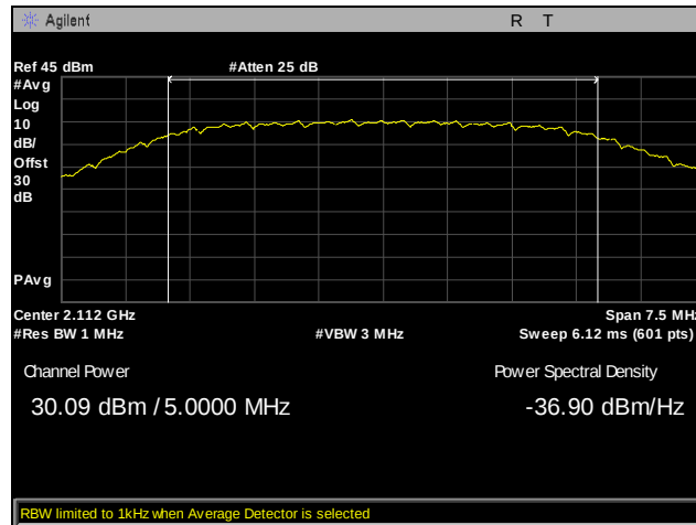
Plot 16. EIRP, Channel 1975, Conducted Power, Part 27, 5 MHz, LTE2100
