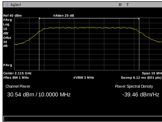
Plot 22. EIRP, Channel 2000, Conducted Power, Part 27, 10 MHz, LTE2100
