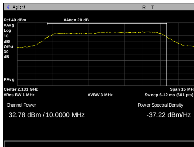
Plot 23. EIRP, Channel 2160, Conducted Power, Part 27, 10 MHz, LTE2100
