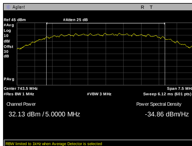
Plot 15. EIRP, Channel 5825, Conducted Power, Part 27, 5 MHz, LTE700
