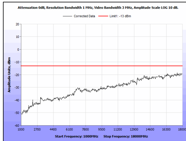
Plot 74. Radiated Spurious Emissions, Low Channel, 1 GHz – 18 GHz, Part 27, 5 MHz, LTE700
