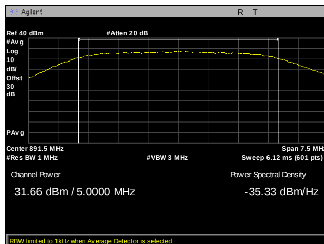
Plot 3. ERP, Channel 2625, Conducted Power, Part 22, 5 MHz
