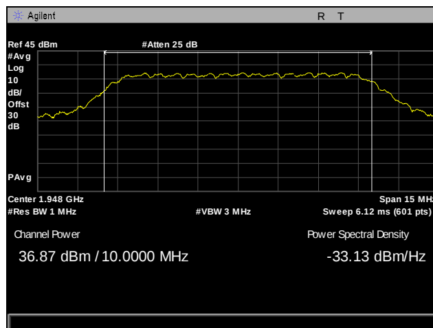
Plot 11. EIRP, Channel 780, Conducted Power, Part 24, 10 MHz
