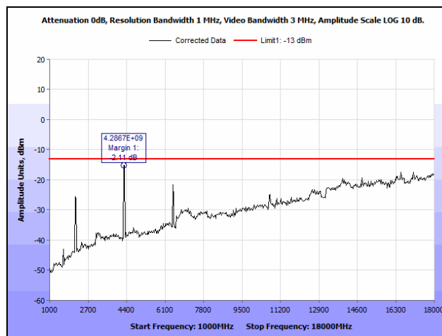
Plot 96. Radiated Spurious Emissions, High Channel, 1 GHz – 18 GHz, Part 27, 10 MHz, LTE2100
