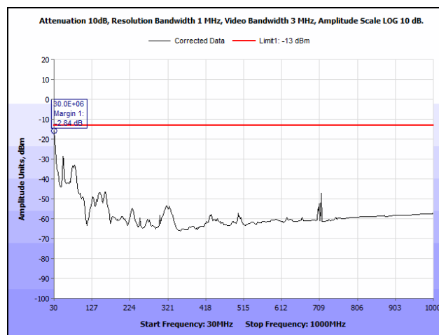
Plot 65. Radiated Spurious Emissions, High Channel, 30 MHz – 1 GHz, Part 24, 5 MHz
