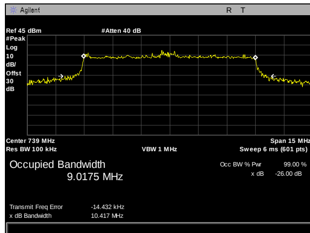
Plot 43. Occupied Bandwidth, Channel 5780, Part 27, 10 MHz, LTE700
