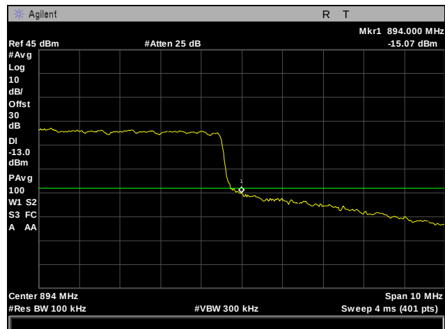
Plot 247. Conducted Band Edge, Channel 2600, 10 MHz, Part 22
