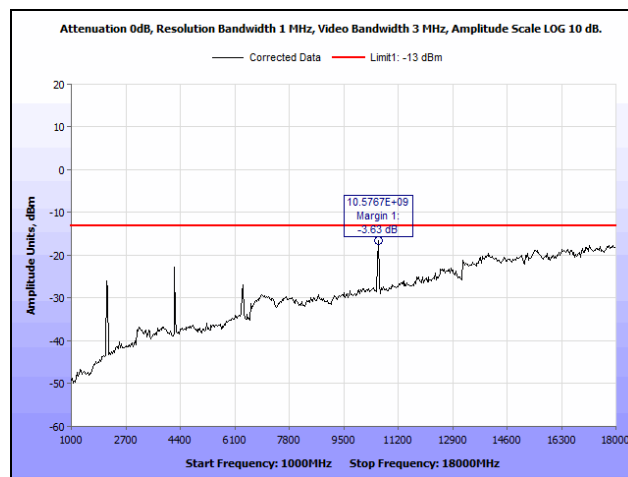
Plot 92. Radiated Spurious Emissions, Low Channel, 1 GHz – 18 GHz, Part 27, 10 MHz, LTE2100
