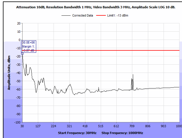
Plot 73. Radiated Spurious Emissions, Low Channel, 30 MHz – 1 GHz, Part 27, 5 MHz, LTE700
