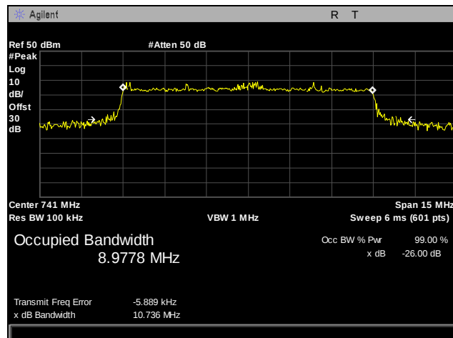
Plot 45. Occupied Bandwidth, Channel 5800, Part 27, 10 MHz, LTE700
