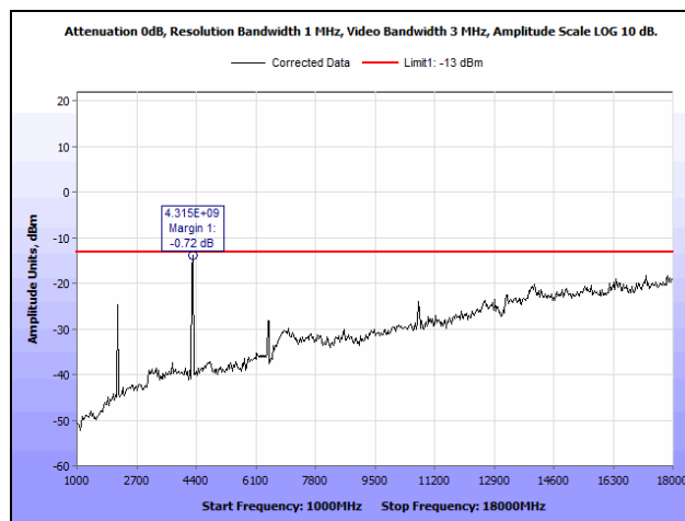
Plot 84. Radiated Spurious Emissions, High Channel, 1 GHz – 18 GHz, Part 27, 5 MHz, LTE2100
