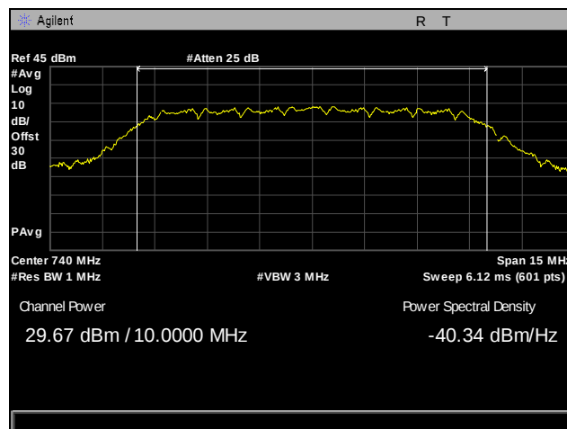
Plot 20. EIRP, Channel 5790, Conducted Power, Part 27, 10 MHz, LTE700
