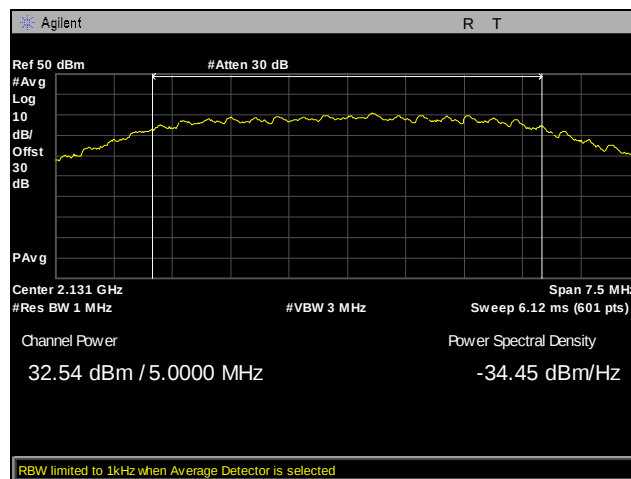
Plot 17. EIRP, Channel 2160, Conducted Power, Part 27, 5 MHz, LTE2100
