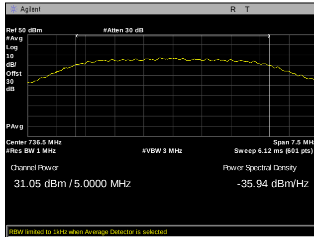
Plot 13. EIRP, Channel 5755, Conducted Power, Part 27, 5 MHz, LTE700
