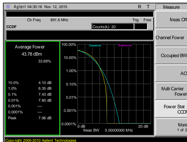
Plot 102. Peak to Average Ratio, Channel 4458, Part 22
