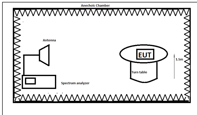
Figure 3. Block Diagram, Above 1 GHz
