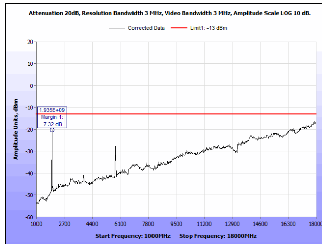
Plot 26. Radiated Spurious Emissions, Low Channel, 1 GHz – 18 GHz, Part 24
