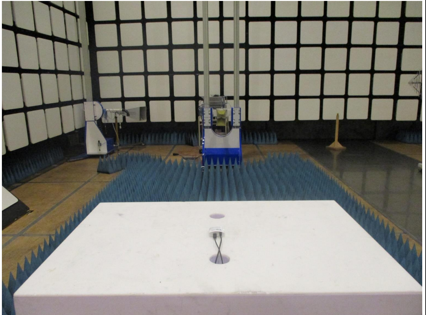
Bild / Picture 2: Test Setup, Radiated disturbance (> 1 GHz)
