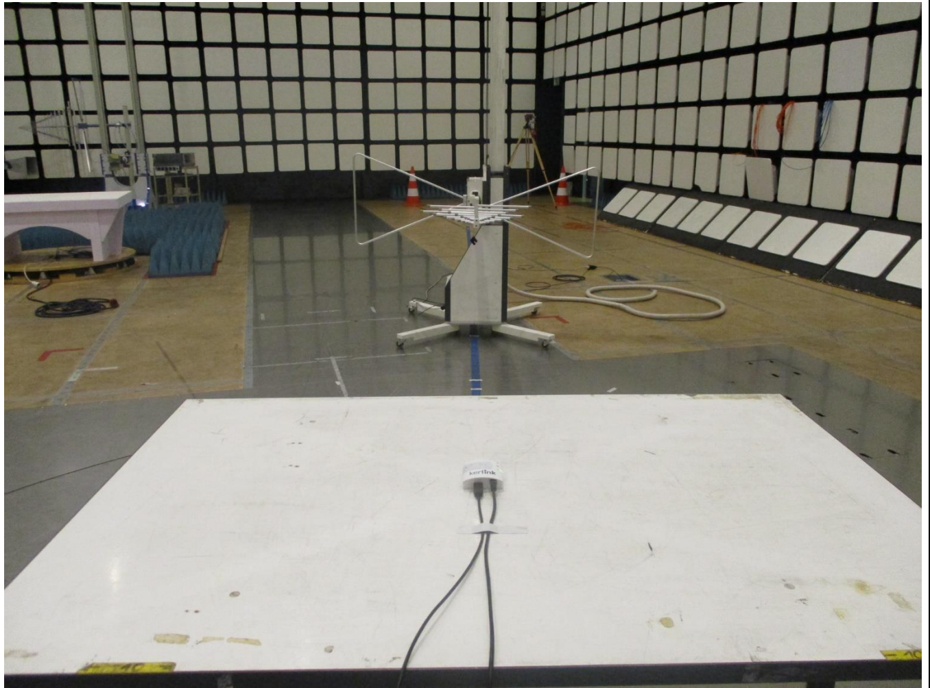
Bild / Picture 1: Test Setup, Radiated disturbance (30 MHz - 1 GHz)
