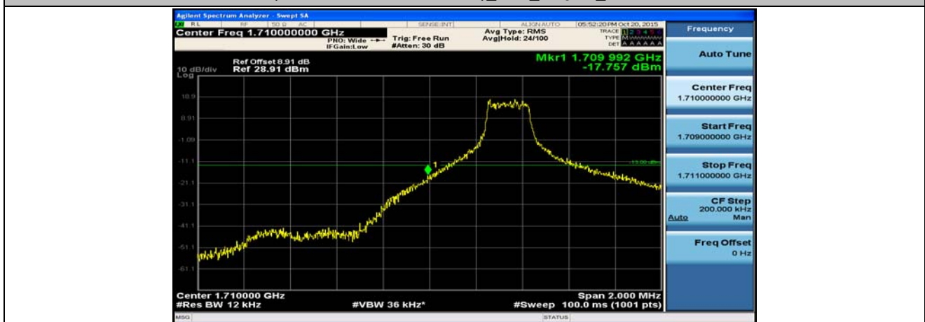
(Channel Bandwidth: 5 MHz)_LCH_16QAM_1RB#12
