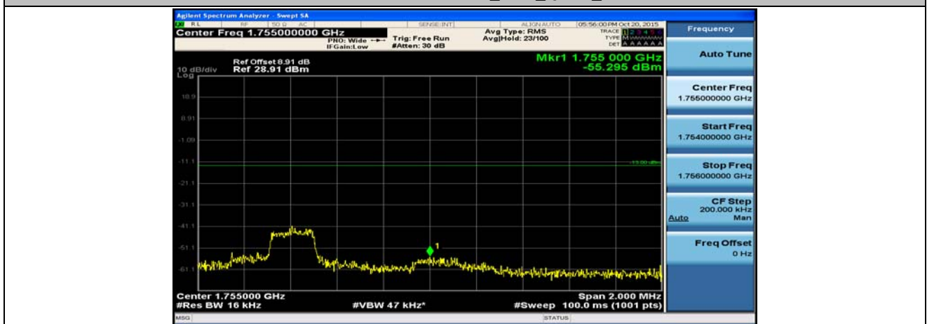
Channel Bandwidth: 10 MHz_HCH_QPSK_1RB#24
