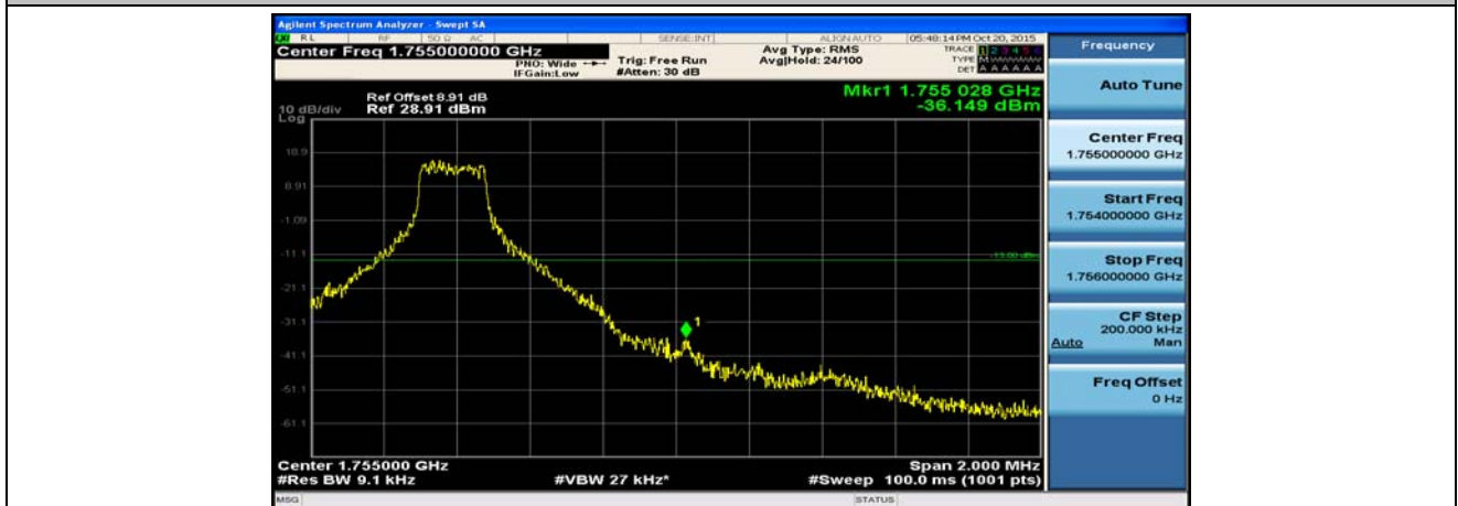
(Channel Bandwidth: 1.4 MHz)_HCH_QPSK_1RB#5
