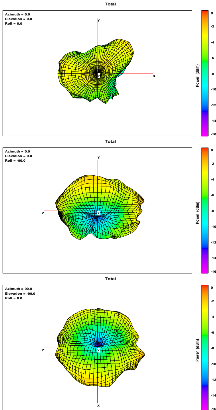
Eureka_2.4GHz_Right
