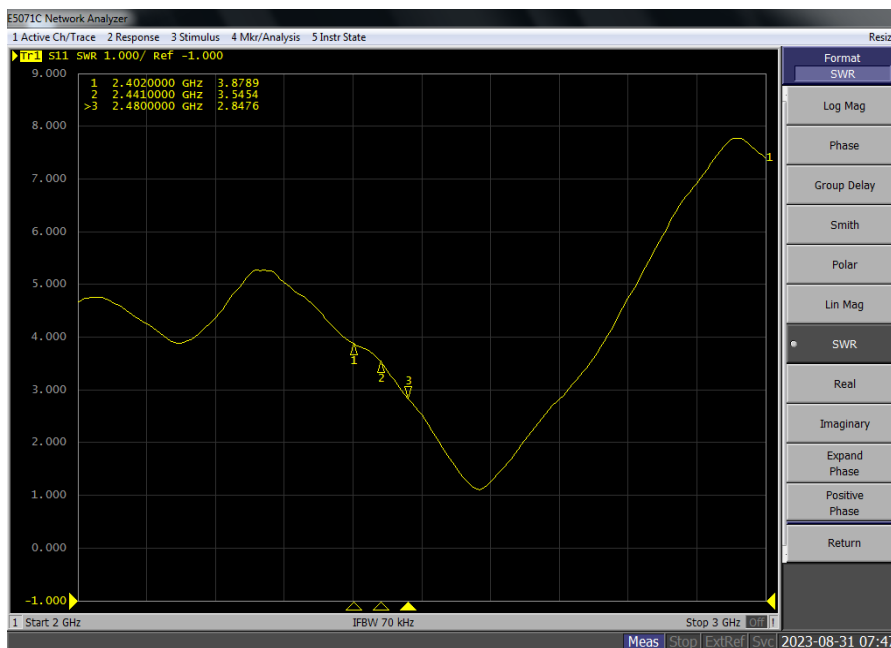
Eureka_2.4GHz_Right
