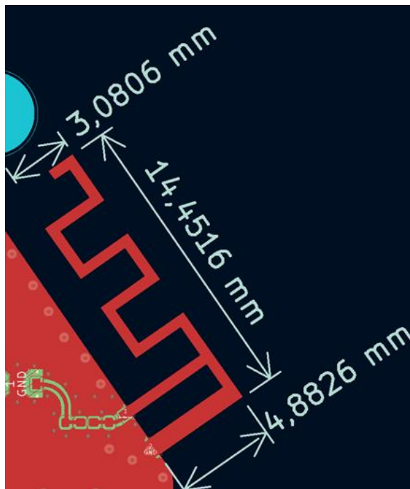
Antenna Dimensions (Eureka_2.4GHz_Right)
