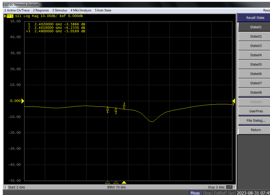
Eureka_2.4GHz_Left
