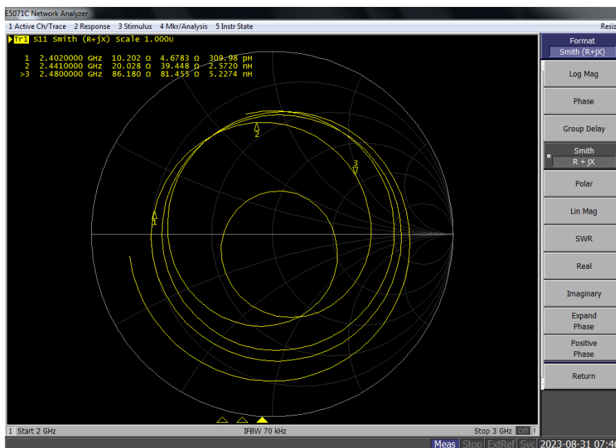
Eureka_2.4GHz_Left
