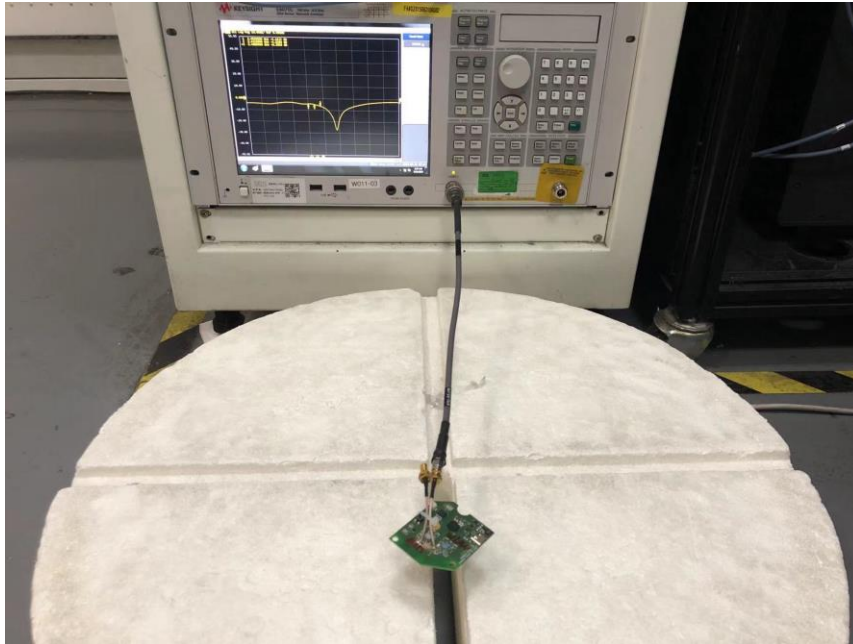
Eureka_2.4GHz_Right Impedance Setup
