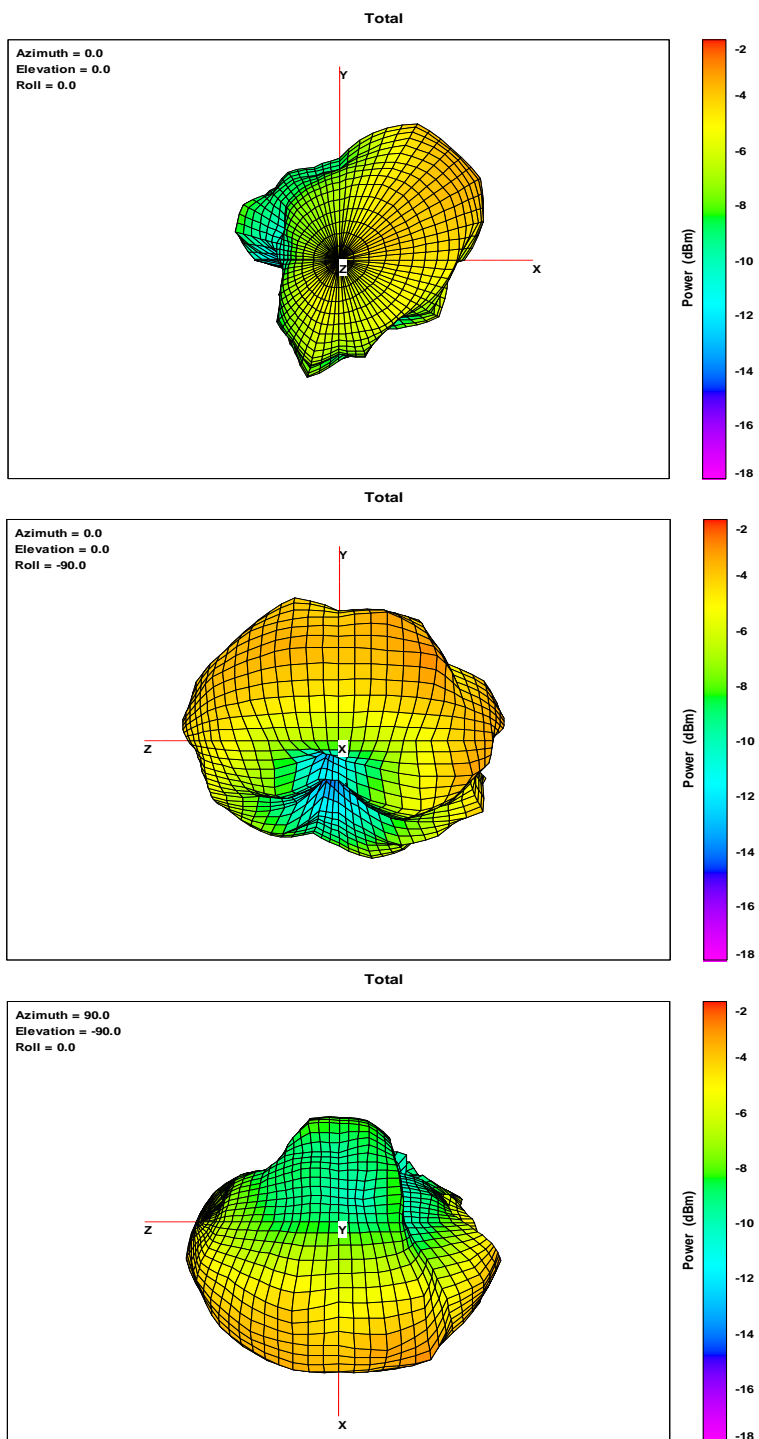
Eureka_2.4GHz_Left
