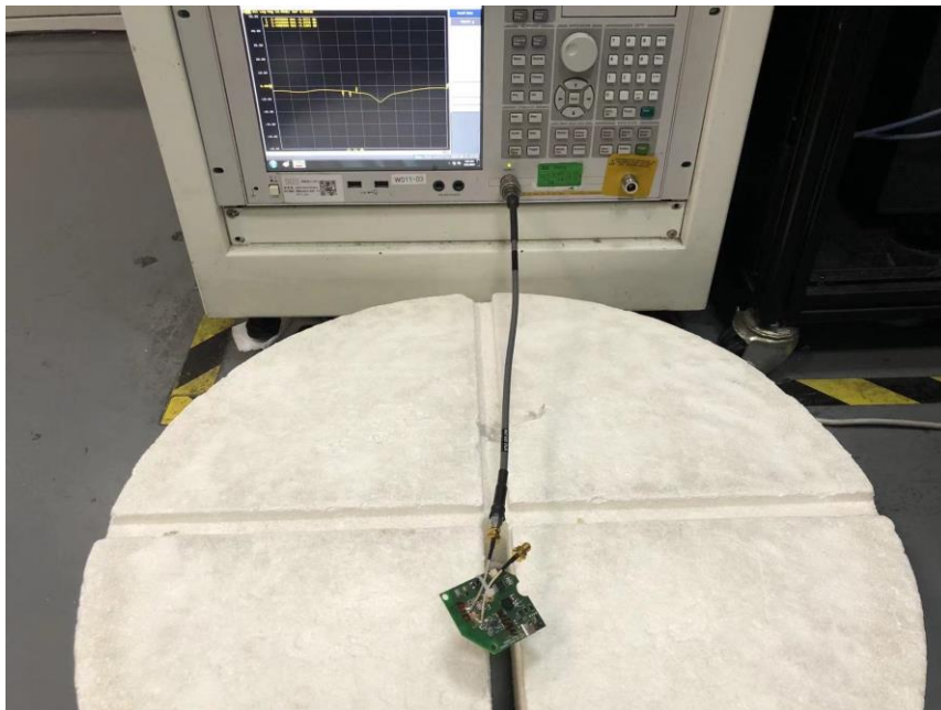
Eureka_2.4GHz_Left Impedance Setup
