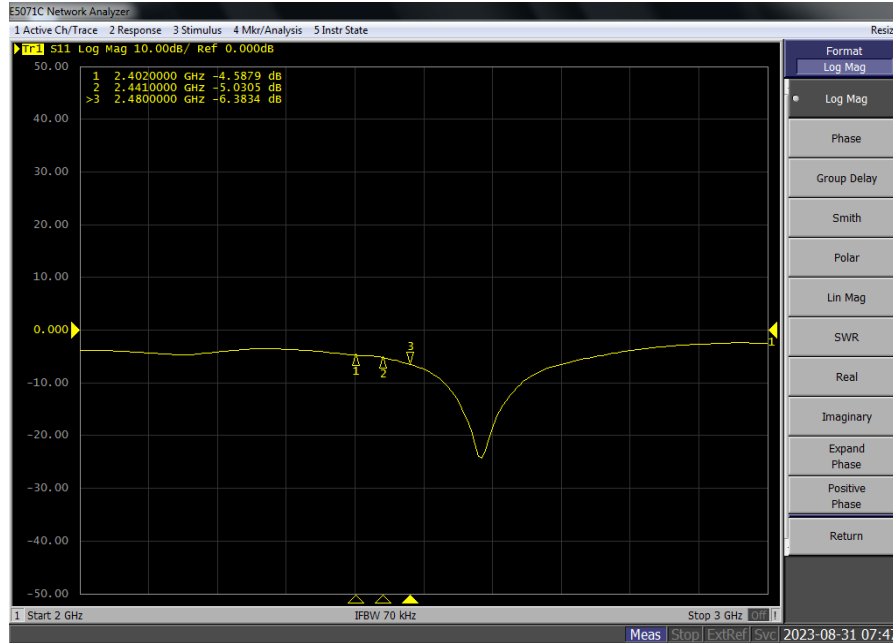
Eureka_2.4GHz_Right
