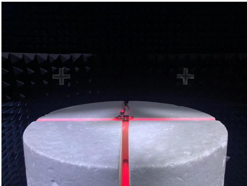
Eureka_2.4GHz_Left Free Space View
