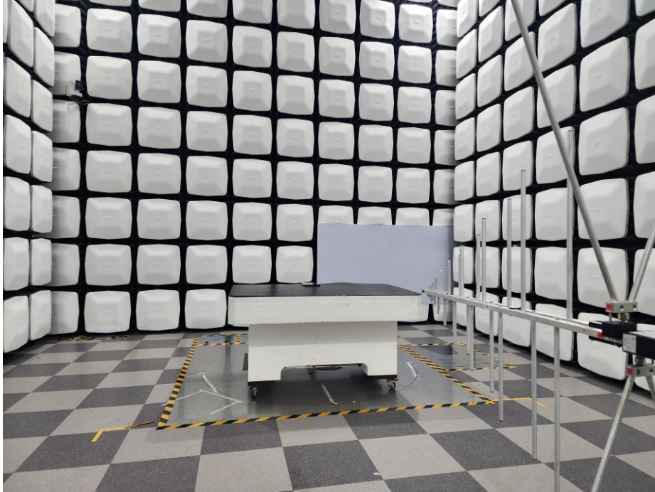
Radiated Test Picture(Front)_Below 1GHz
