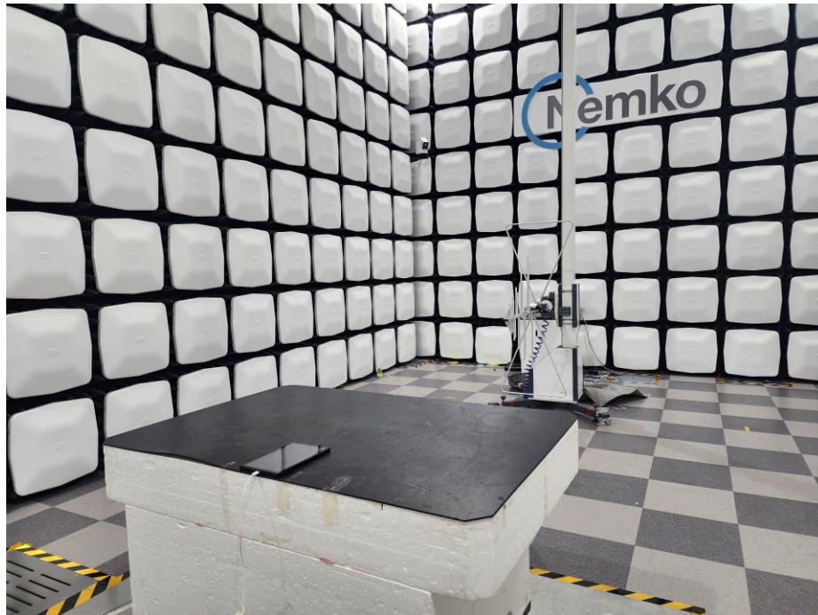
Radiated Test Picture(Rear)_Below 1GHz
