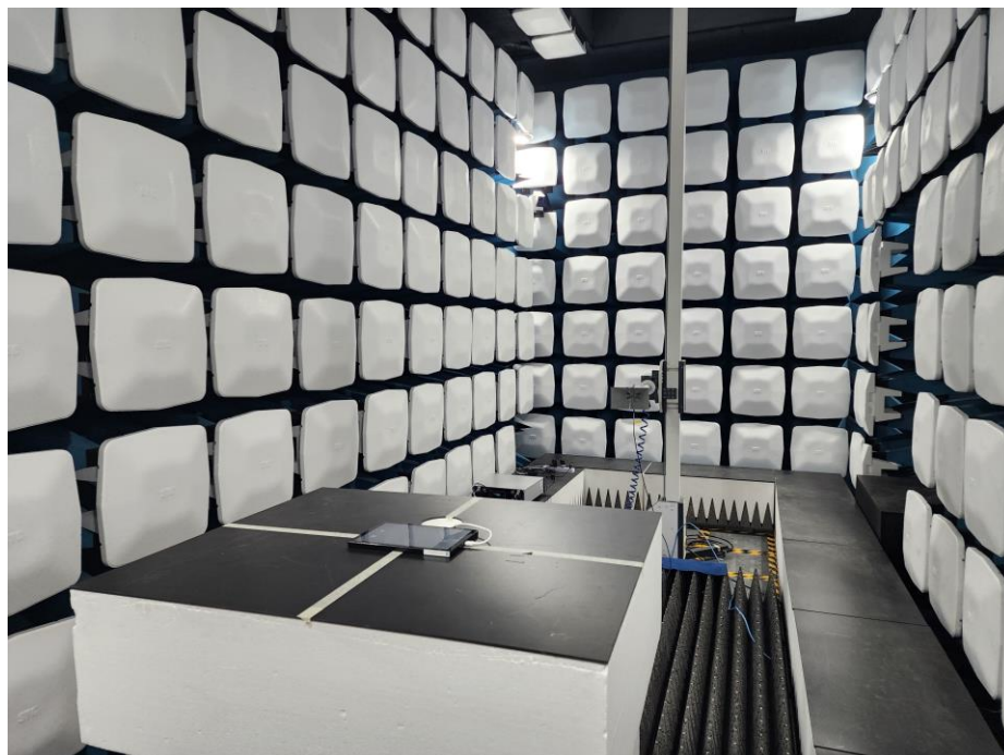
Radiated Test Picture(Rear)_Above 1GHz
