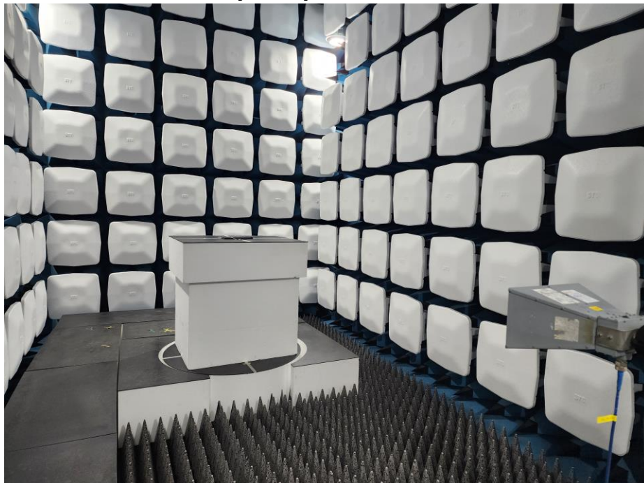
Radiated Test Picture(Front)_Above 1GHz
