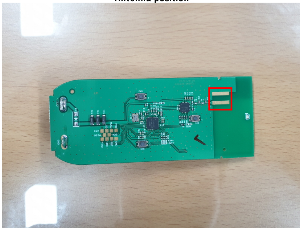
Antenna connection
