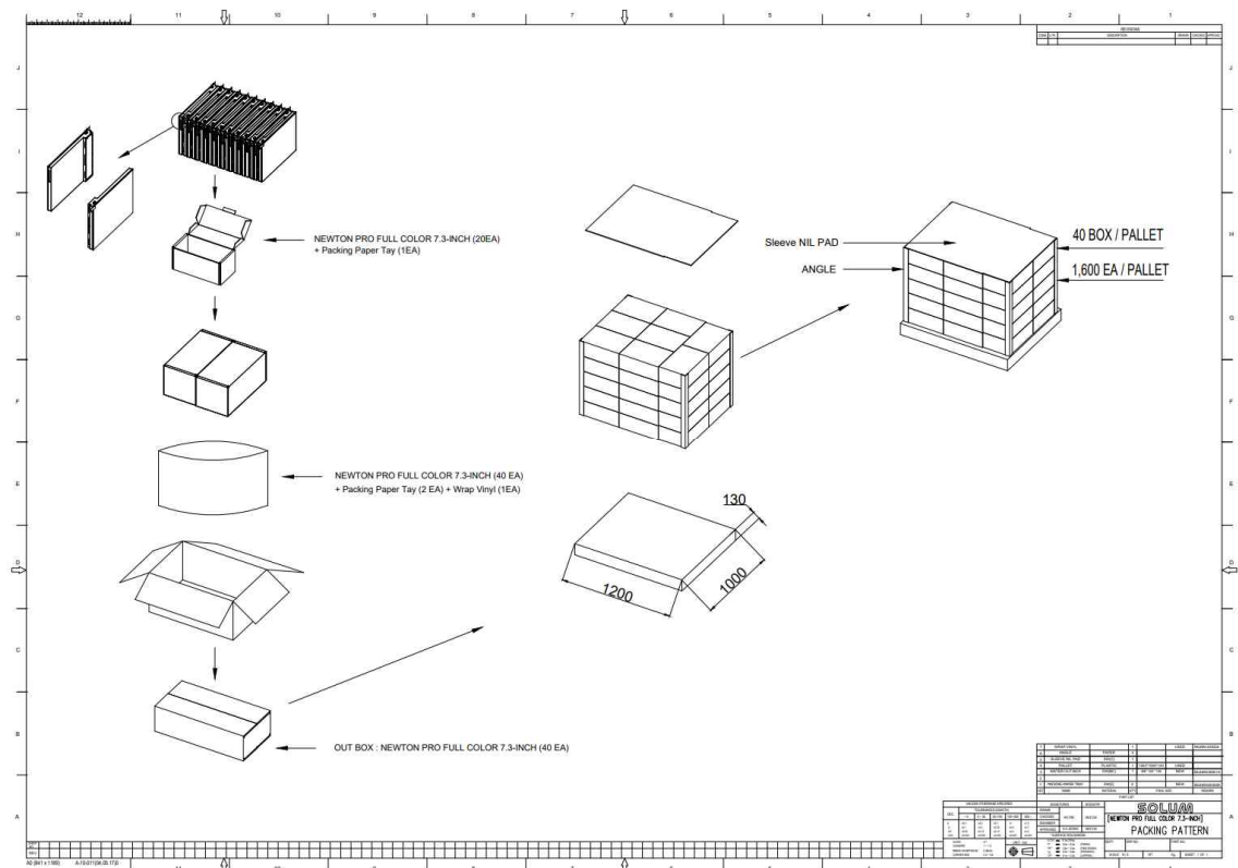
Figure 12. 7.3" Packing-Diagram (1,200 X 1,000)
