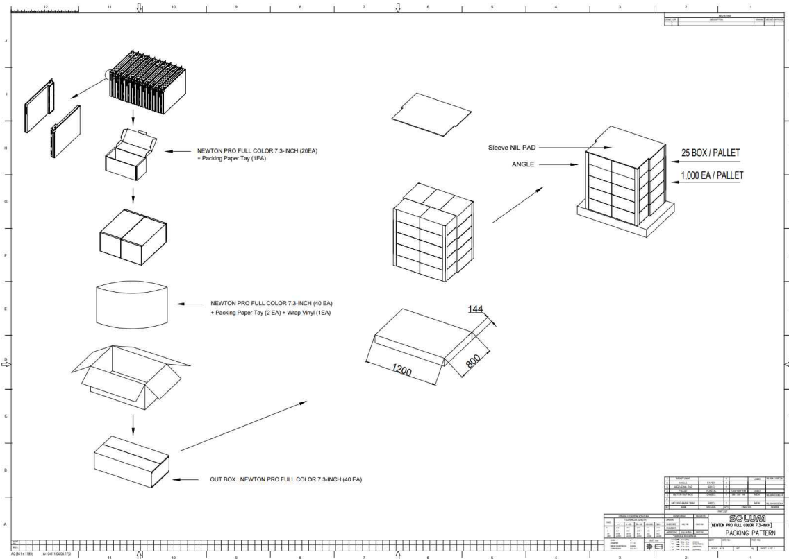
Figure 11. 7.3" Packing-Diagram (1,200 X 800)
