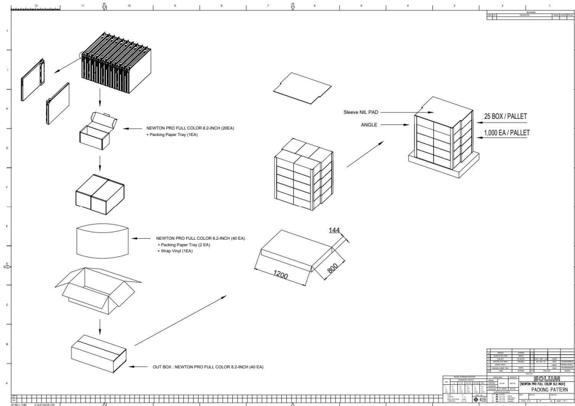
Figure 13. 8.2" Packing-Diagram (1,200 X 800)
