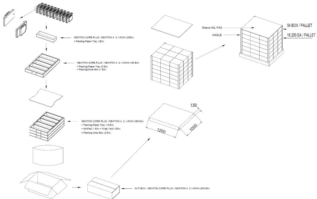
Figure 13. 2.1" PACKING-DIAGRAM (1,200 X 1,000)
