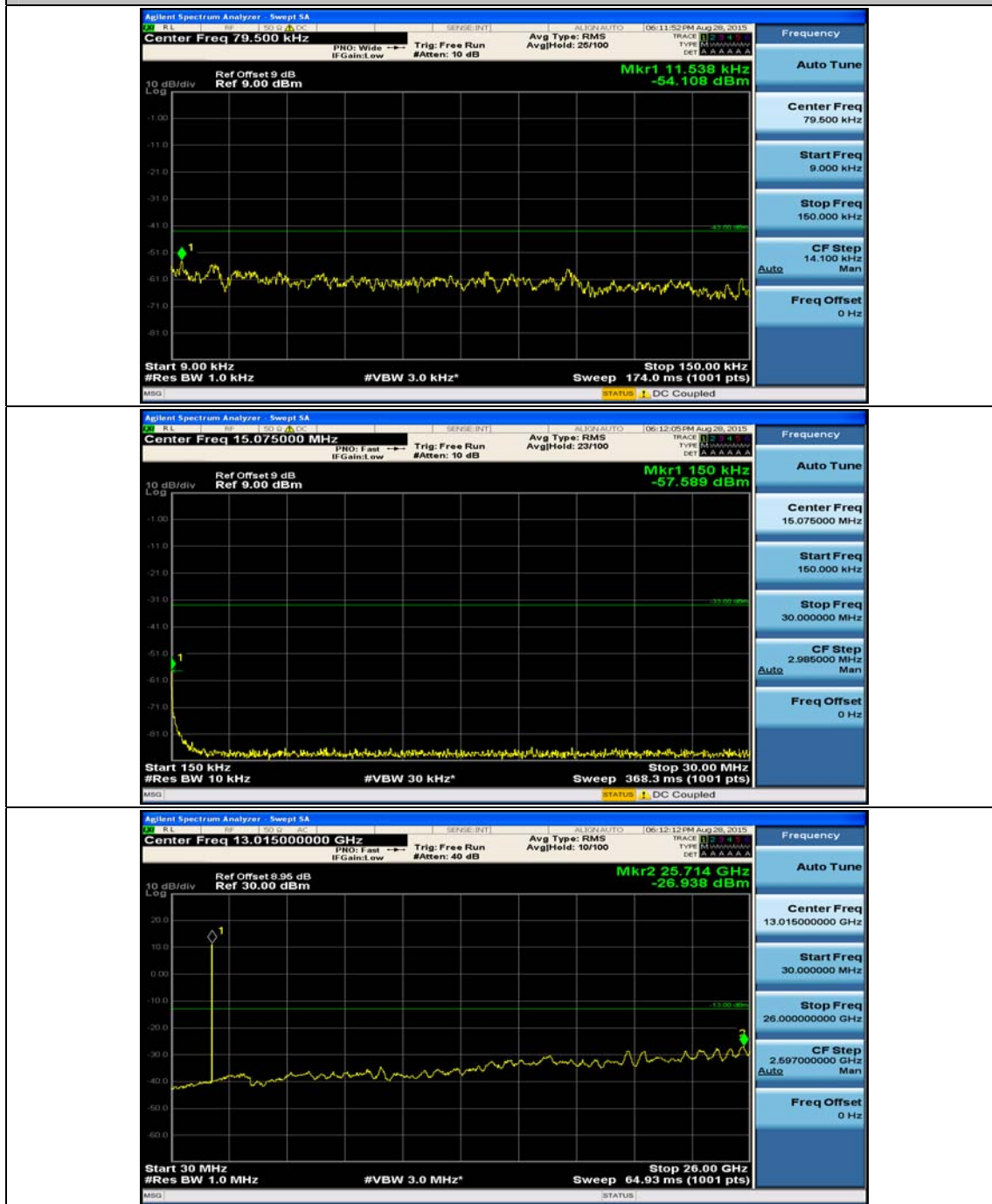
(Channel Bandwidth: 5 MHz)_MCH_16QAM_1RB#12
