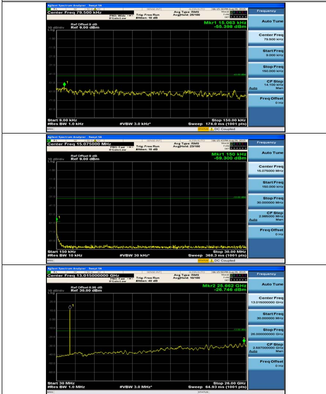
(Channel Bandwidth: 5 MHz)_HCH_16QAM_1RB#24
