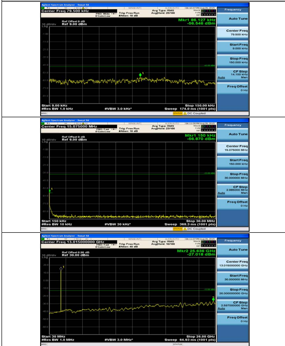
(Channel Bandwidth: 5 MHz)_MCH_QPSK_1RB#24
