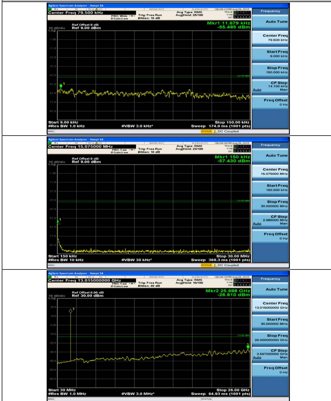
(Channel Bandwidth: 5 MHz)_LCH_16QAM_1RB#24
