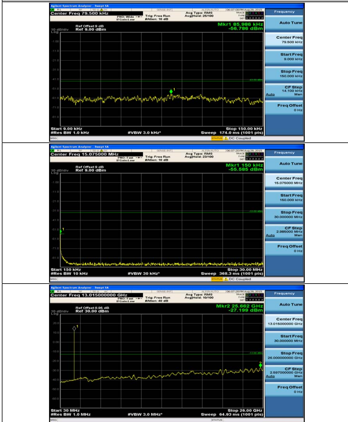
(Channel Bandwidth: 5 MHz)_LCH_QPSK_1RB#12
