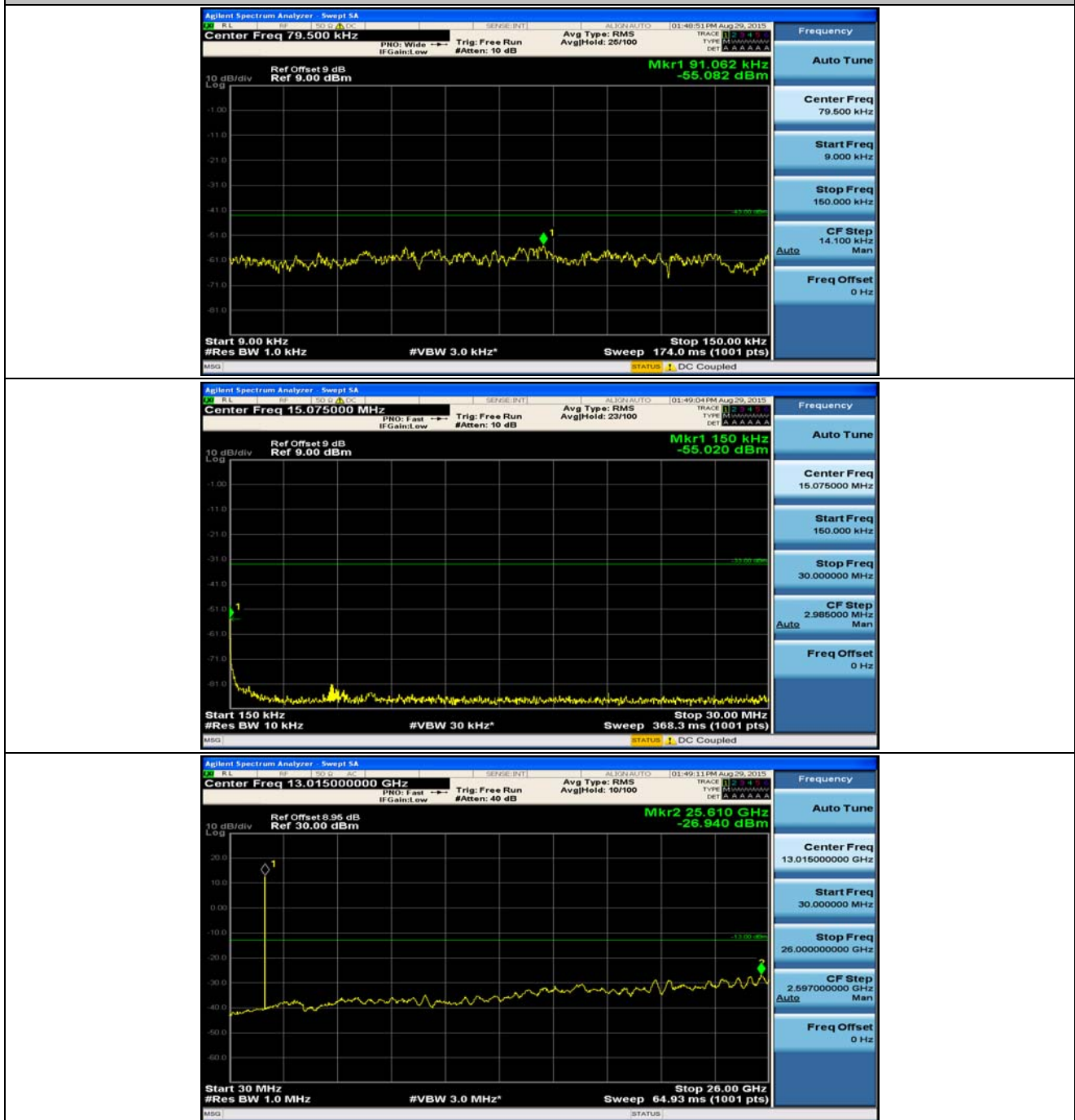
(Channel Bandwidth: 20 MHz)_HCH_QPSK_1RB#49
