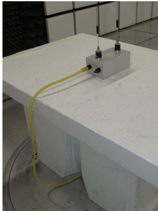
Figure 4: Radiated Emissions - Rear View – Below 1GHz
