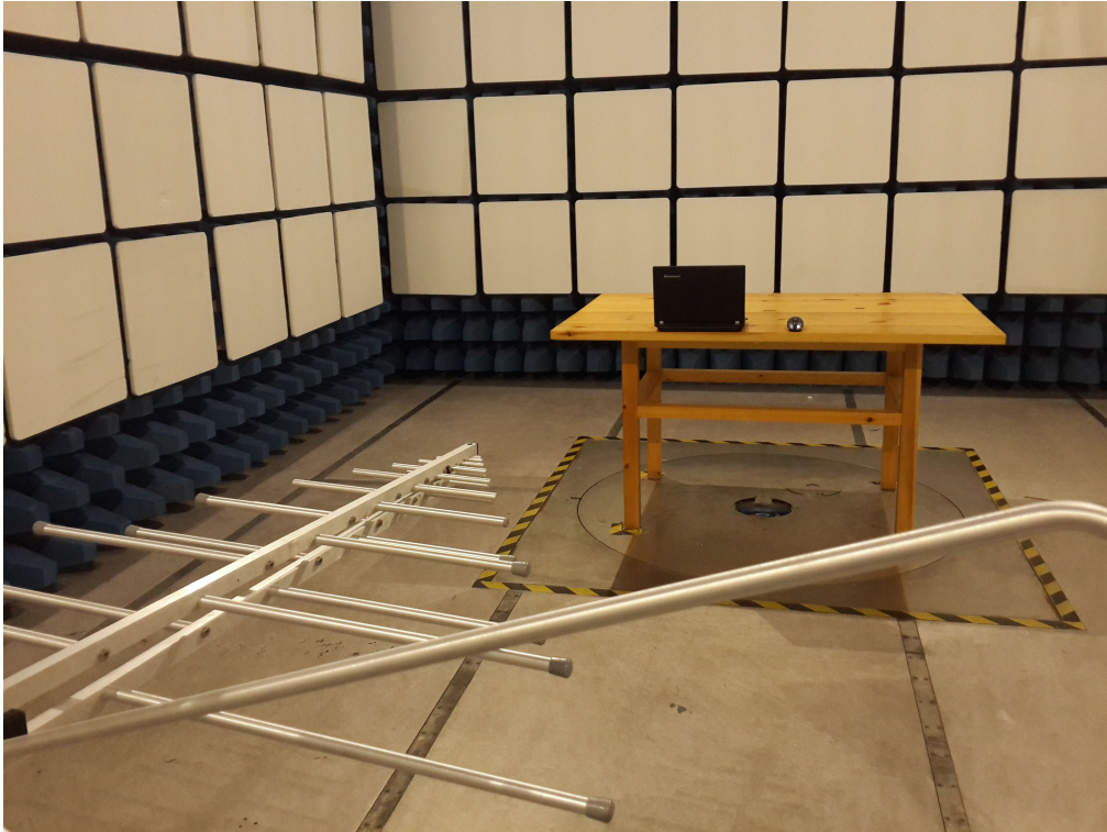
30 MHz-1 GHz (The Working test mode)
