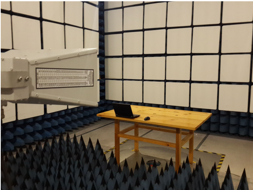
Above 1 GHz (The Working test mode)
