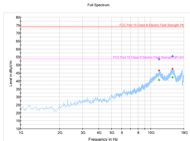
Figure 8.1-10: Radiated spurious emissions >1GHz for EUT with iPhone 6 – CDMA BCo Ch1013
